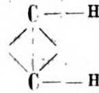
Acetylen
