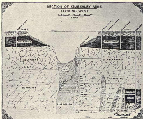
FIG. 4. SECTION OF KIMBERLEY MINE.
