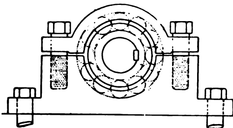
Abb. 408. Kugellager, 1857.
