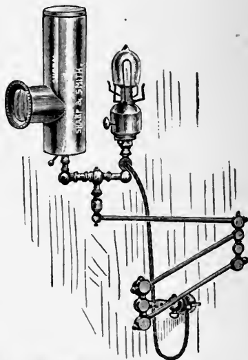
FIG. 56.—MODIFIED MACKENZIE'S RACK-MOVEMENT BULL'S-EYE CONDENSER. For gas or incandescent electric light.
