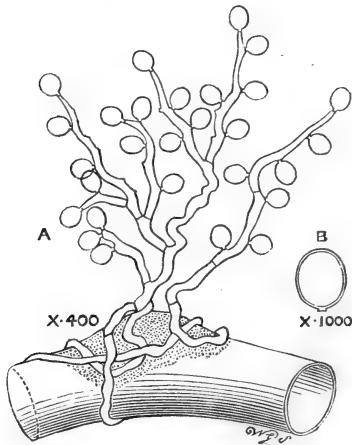
FIG. 2.—CLOVER MILDEW.
