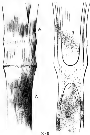
FIG. 25.—STRAW BLIGHT.
