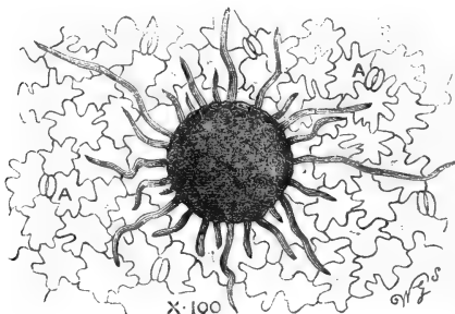
FIG. 123.—PEA MILDEW.
