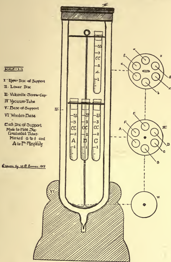
Apparatus Made By Emery Amend New York.
