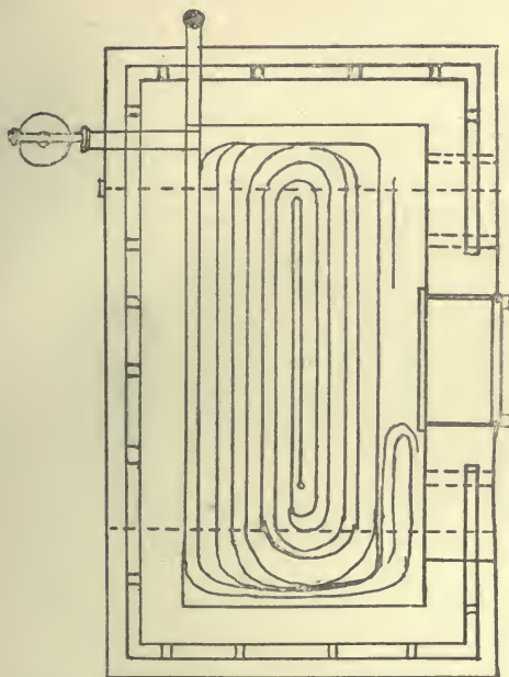
Fig. 16.—Plan showing arrangement of heating pipes.
