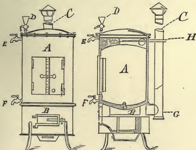
Fig. 32.—Elevation.
