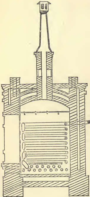
Fig. 14.—Longitudinal section.
