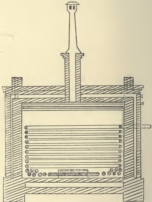
Fig. 15.—Transverse section.
