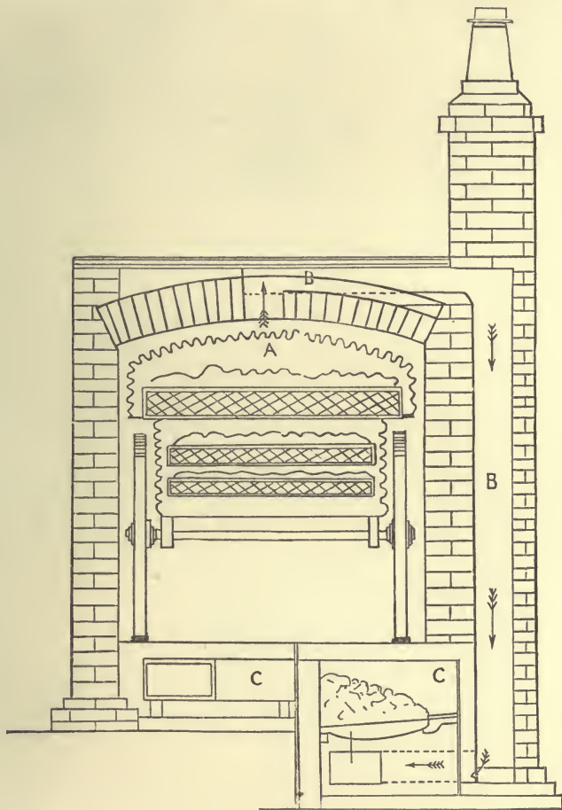
Fig. 4. Transverse section.
