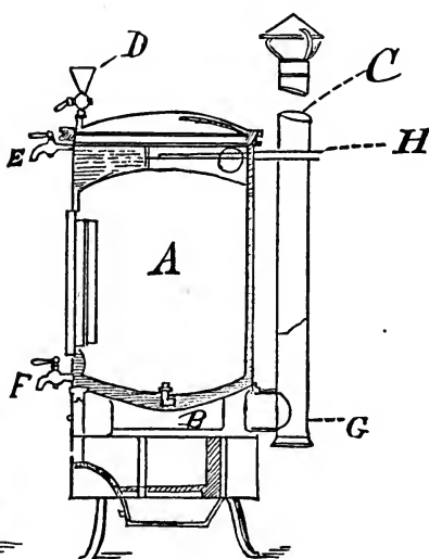
Fig. 33.—Longitudinal section.
