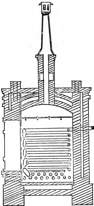
Fig. 14.—Longitudinal section.
