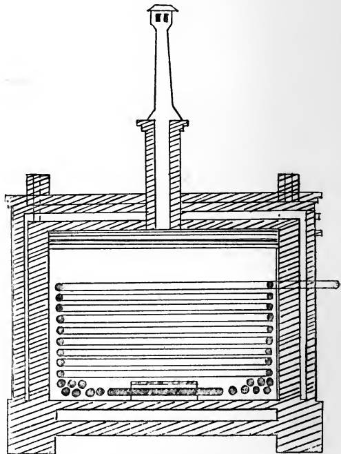
Fig. 15.—Transverse section.
