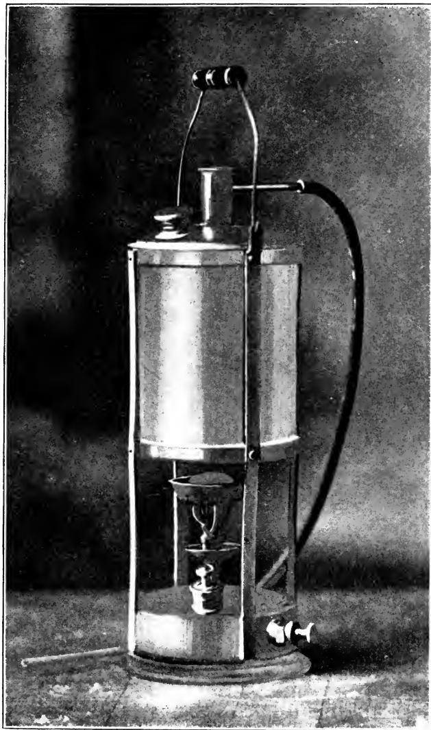
THE REX GENERATOR.
