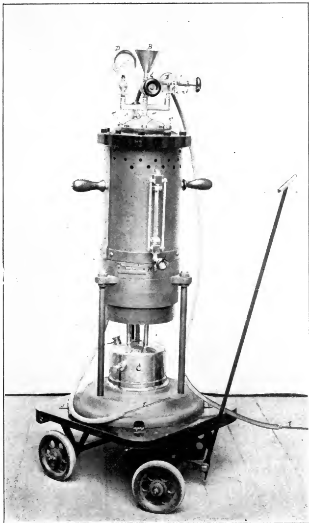
KNY-SCHEERER GENERATOR. NO. 3.
