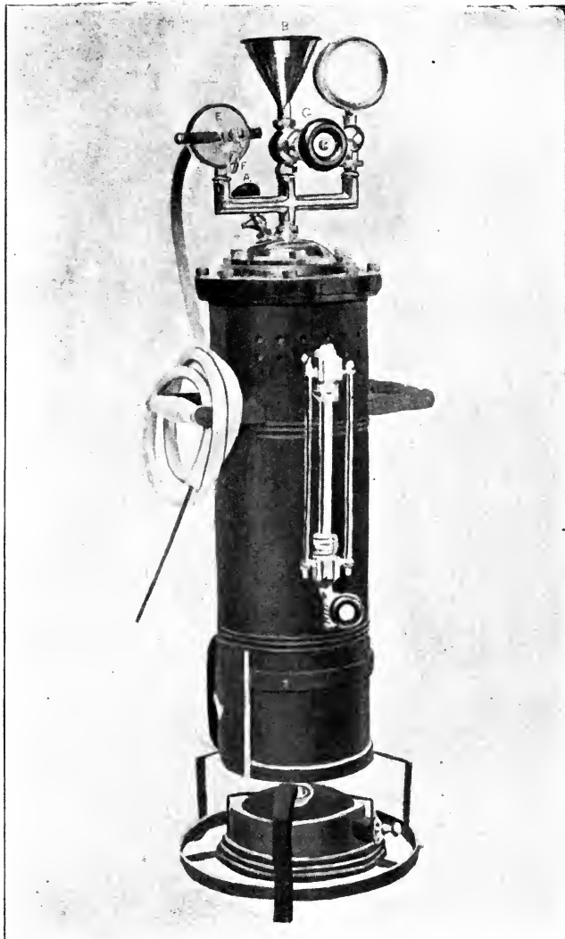
THE KNY-SCHEERER GENERATOR NO. 2.
