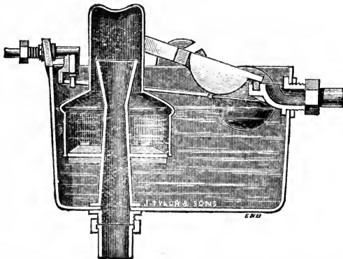
FIG. 303.—Capped single-syphon cistern water waste-preventer.
