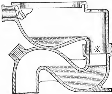
FIG. 158.—Wash-out water-closet in two pieces.
