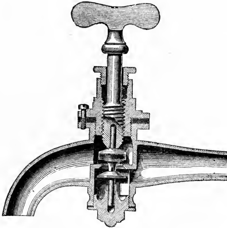
FIG. 317.—Section of same.
