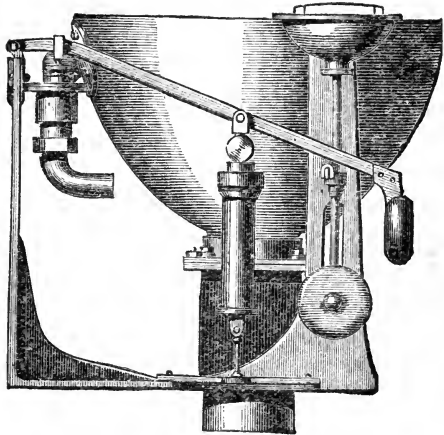
FIG. 183.—Ordinary valve water-closet.
