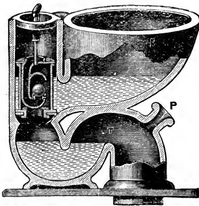
FIG. 179.—Safety plug-valve water-closet, trapped over floor.
