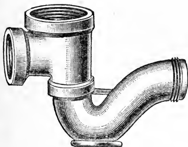
FIG. 87.—Adjustable interceptor.
