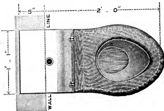
FIG. 192.—Plan of corbel wash-down water-closet.
