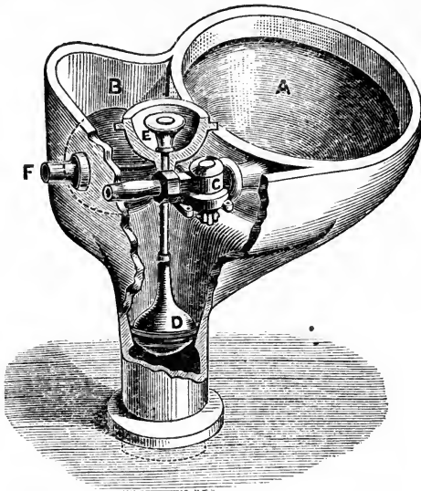
FIG. 178.—Trapless twin-basin water-closet.
