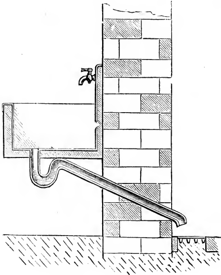
FIG. 239.—Lead-lined trough.
