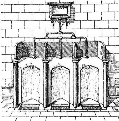
FIG. 216.—Improved urinal range.
