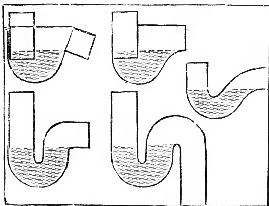
FIG. 143.—Various lead traps.
