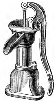
FIG. 345.—American pitcher pump.
