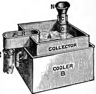
FIG. 103.—Tinned-copper grease-collector for placing under scullery sink for daily removal.
