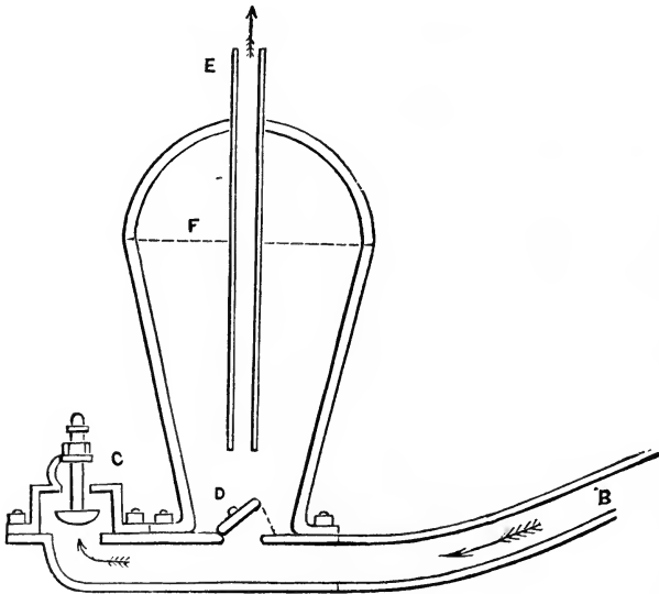
FIG. 352.—Section of American hydraulic ram.
