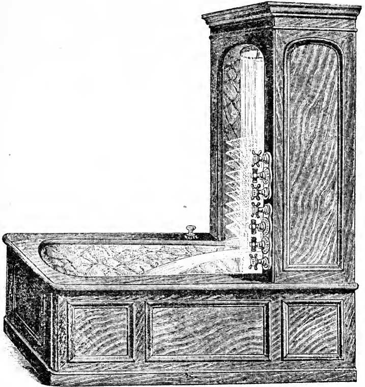
FIG. 262.—Wood-encased reclining shower and douche bath.
