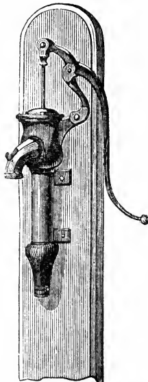
FIG. 344.—Lift pump on plank.
