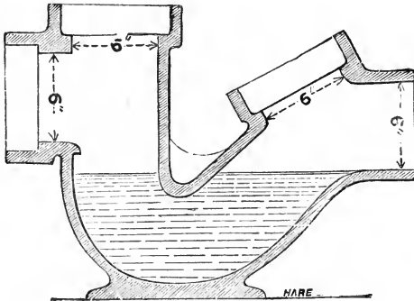
FIG. 75.—Interceptor trap.
