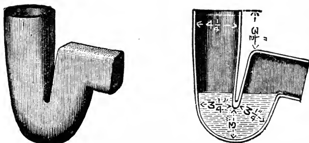
FIG. 146.—Anti D -traps.
