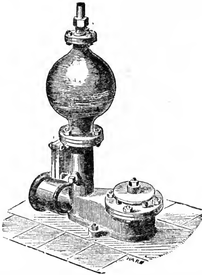
FIG. 354.—English hydraulic ram, single foot-valve.
