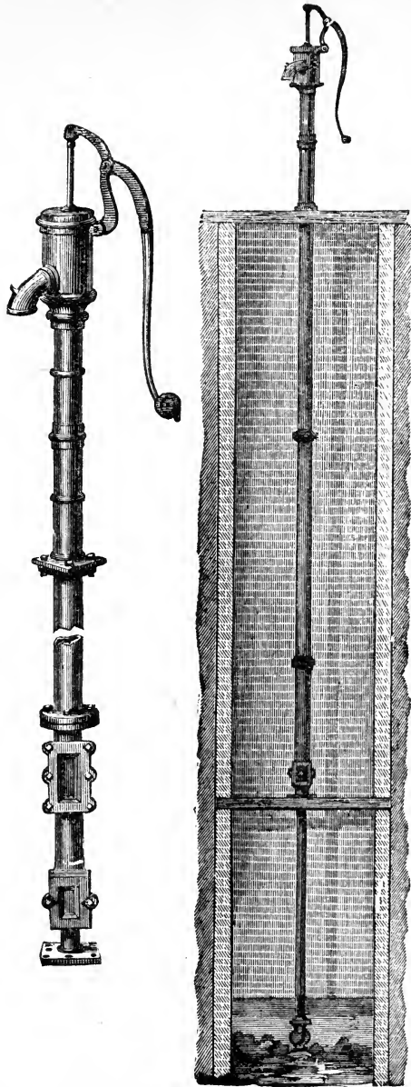
FIG. 346.—Illustrations of deep-well lift pump before and after being fixed in deep well.
