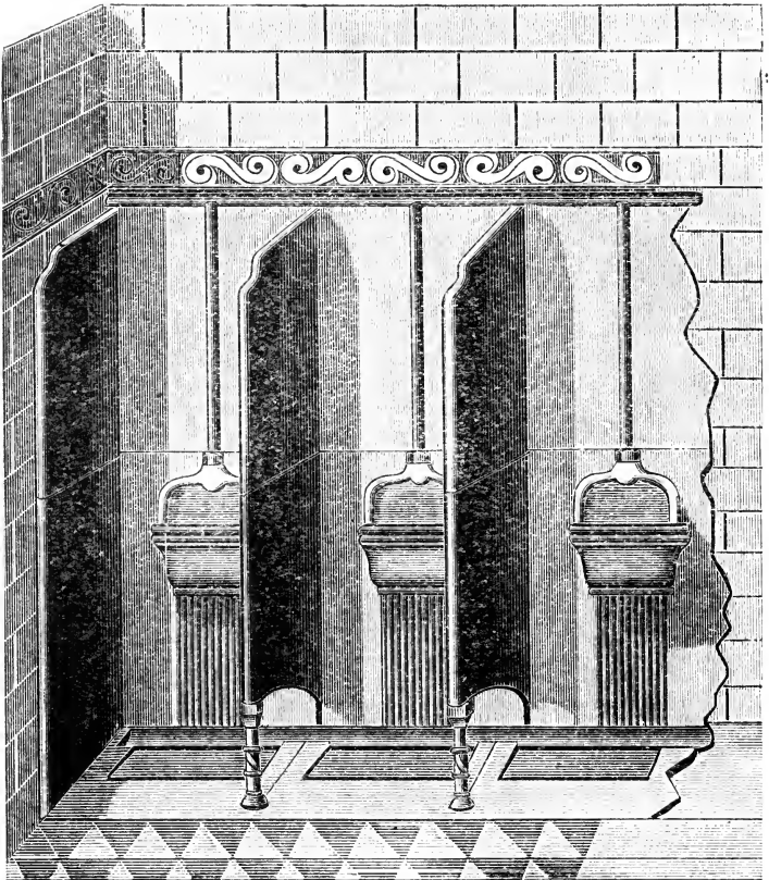
FIG. 215.—Fire-clay wall range of urinals.
