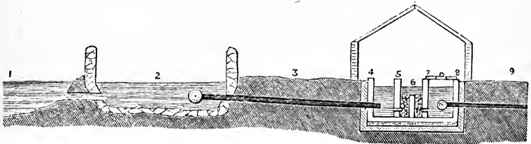
FIG. 341.—Filtering arrangement at head of water supply for river water. 3
