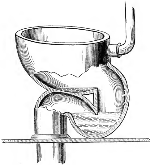
FIG. 159.—Wash-out water-closet in one piece.
