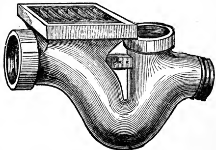
FIG. 78.—Interceptor trap.
