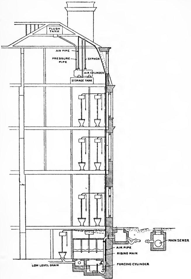
FIG. 16.—Patent Sewage Lift.
