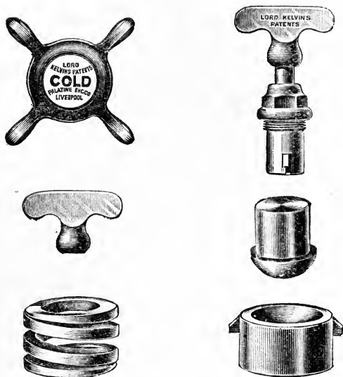
FIG. 329.—Details of Kelvin taps.
