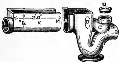
FIG. 81.—Chamber channel and interceptor.
