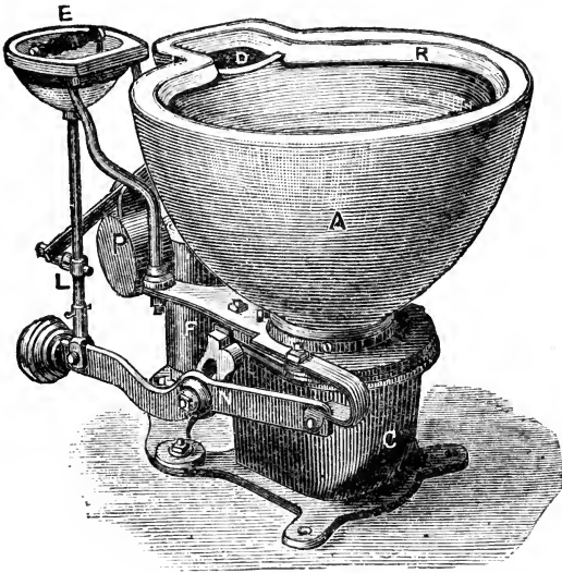
FIG. 186.—Improved valve water-closet.
