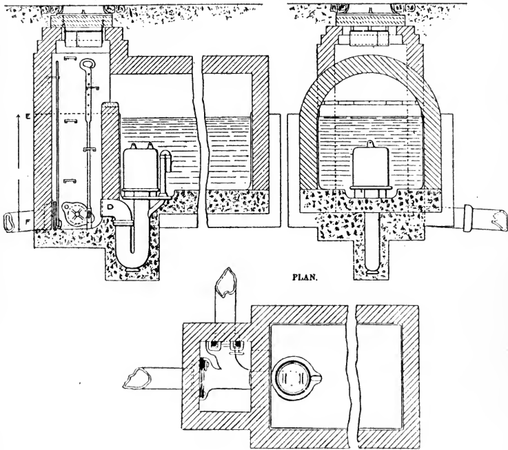
FIG. 17.—Adams' Patent Flush Syphon.
