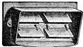
FIG. 109.—Ornamental quadruple mica flap-valve, showing also back view and construction of the mica valves, hung on copper loops, and moving with the slightest breath of air to open or close.
