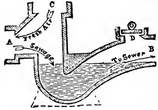
FIG. 76.—Interceptor trap.
