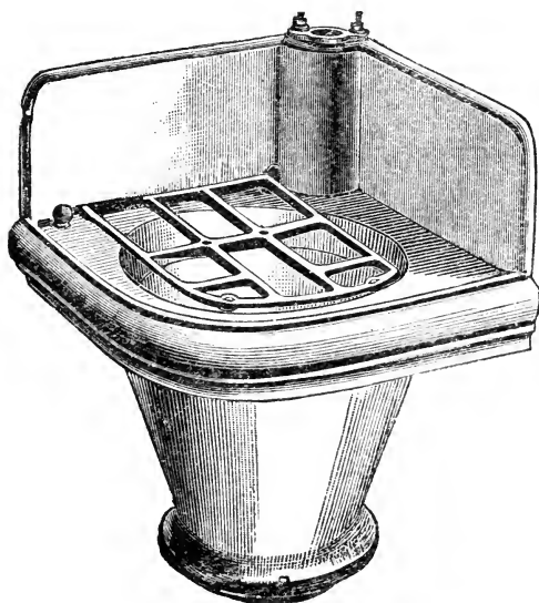
FIG. 221.—Improved earthenware slop-sink, with can-rest hinged over.
