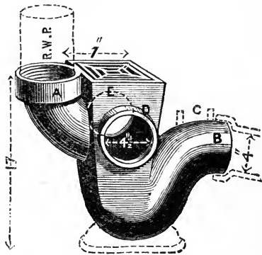
FIG. 95.—Disconnecting receiver.
