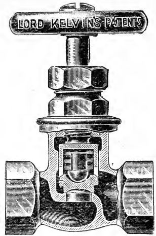
FIG. 340.—Kelvin steam tap.
