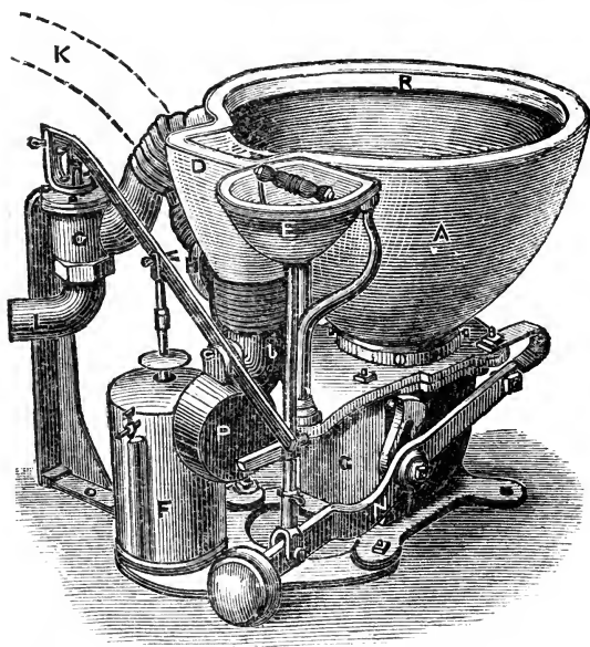
FIG. 185.—Improved valve water-closet.
