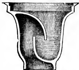
FIG. 152.—Mid-feather trap.
