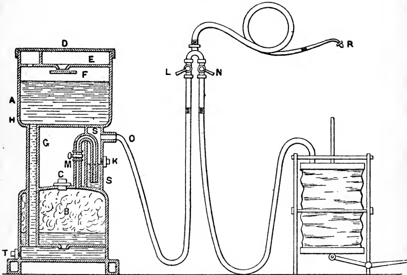
FIG. 155.—Lead-burning machine.
