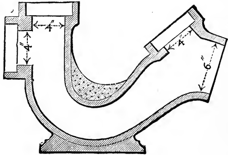
FIG. 77.—Interceptor trap.
