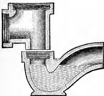
FIG. 85.—Adjustable interceptor.
