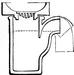
FIG. 97.—Gully-trap.
