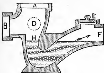
FIG. 79.—Interceptor trap.
