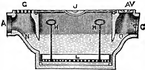
FIG. 102.—Earthenware grease-trap, with galvanised-iron cover and lifting tray.
