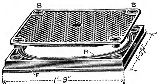
FIG. 73.—Reliable screw-down cover.
