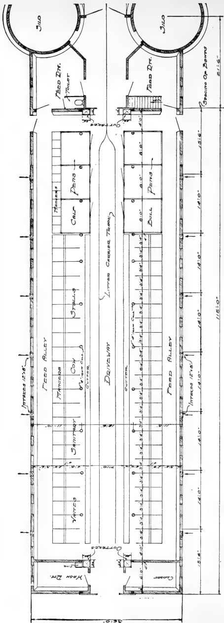
Ground Floor Plan—Dr. David Roberts' Stock Barn, Waukesha, Wis.
