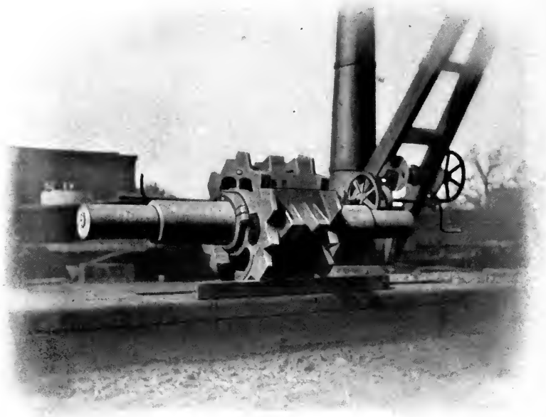
UPPER TUMBLER AND SHAFT
