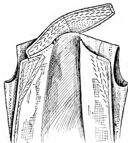
Fig. 307. Stretch the Collar Between Notches
