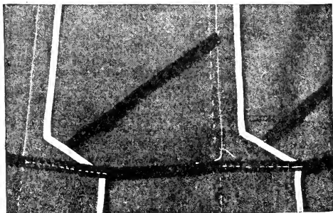
Fig. 299. Supporting Inlaid Plaits
