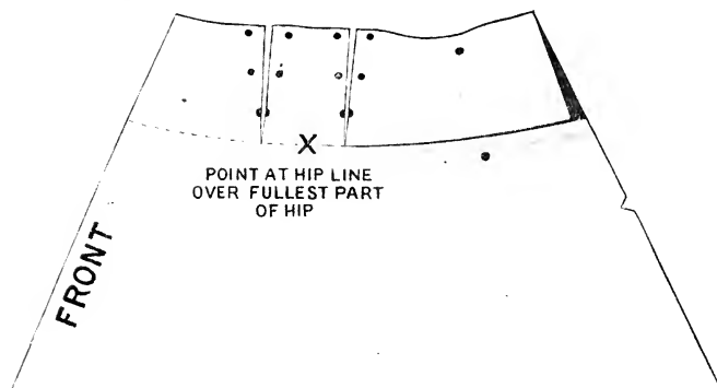
Fig. 210. When the Hips Are Large
