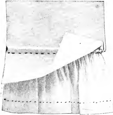
Fig. 38. Ruffle Inserted in a Hem
