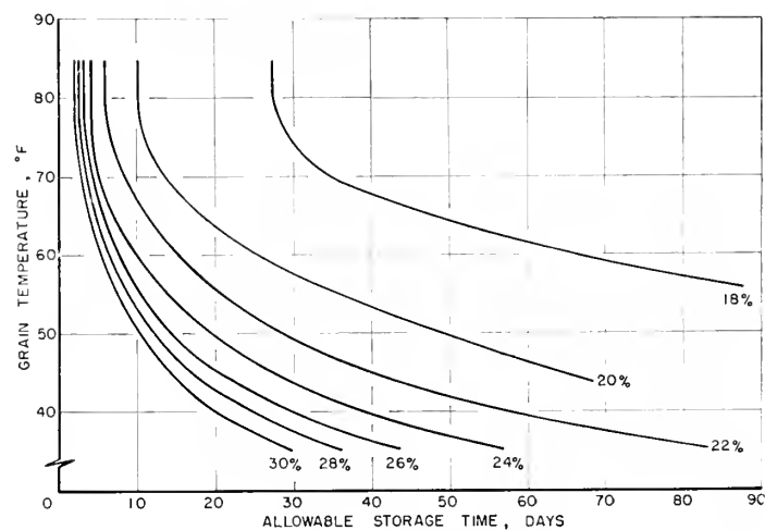
Allowable storage time for shelled corn at various temperatures and moisture contents. During these times the grain will lose .5 percent in dry matter but will still be acceptable. Data are from the U. S. Department of Agriculture Grain Storage Research Laboratory at Ames, Iowa. (Fig. 3)
