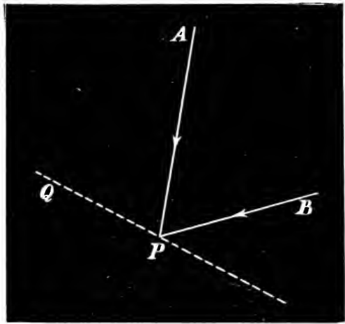
Fig. 63. — MOMENT OF MOMENTUM UNALTERED BY COLLISION.
