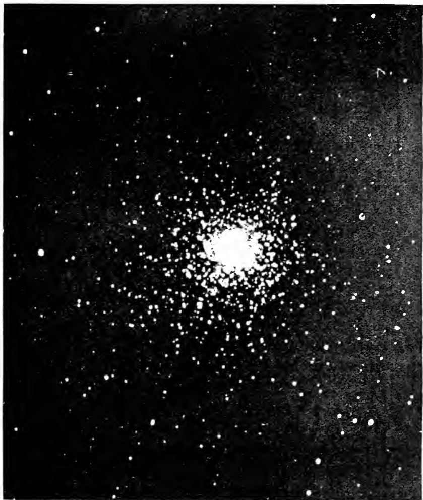
Fig. 9.—THE CLUSTER IN HERCULES.
