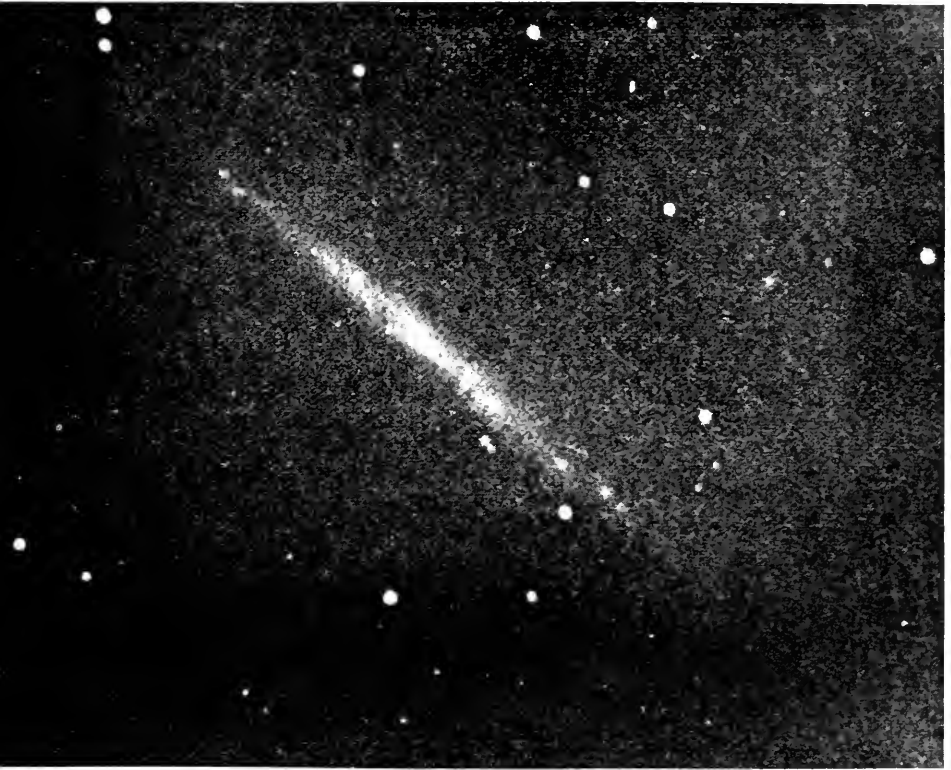
Fig. 35.—EDGE VIEW OF A SPIRAL BOLDLY SHOWN (n.g.c. 4565; in Coma Berenices).
