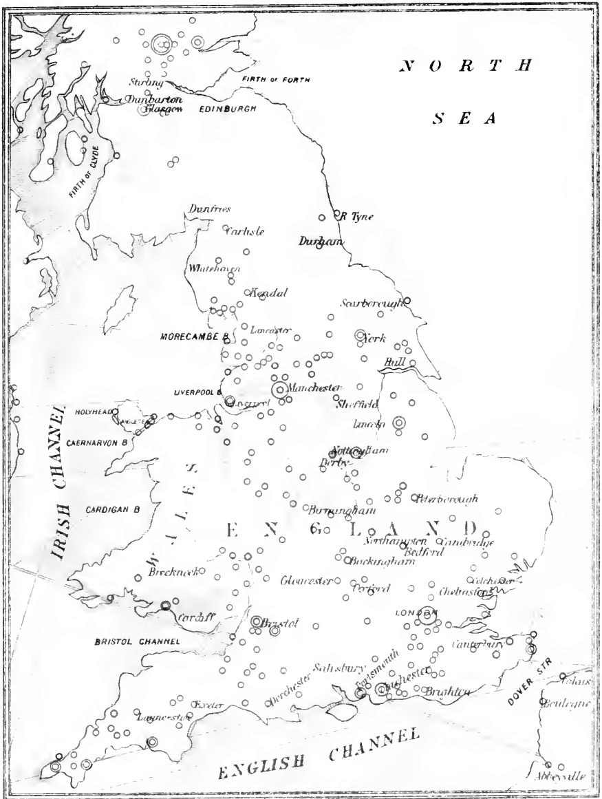
SHOWING LOCALITIES OF EARTHQUAKES
