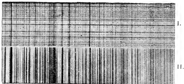
Fig. 15.— I. SPECTRUM OF THE SUN.
