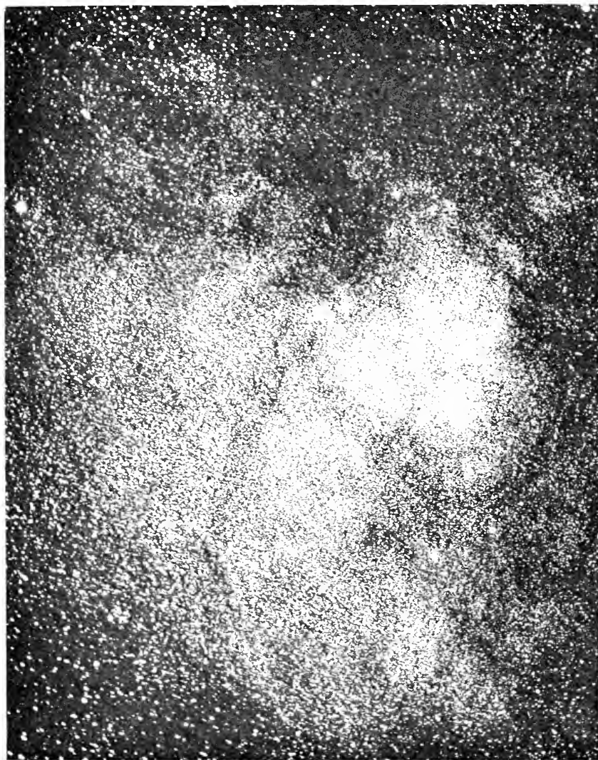
Fig. 32.—PORTION OF THE MILKY WAY (NEAR MESSIER II.).
