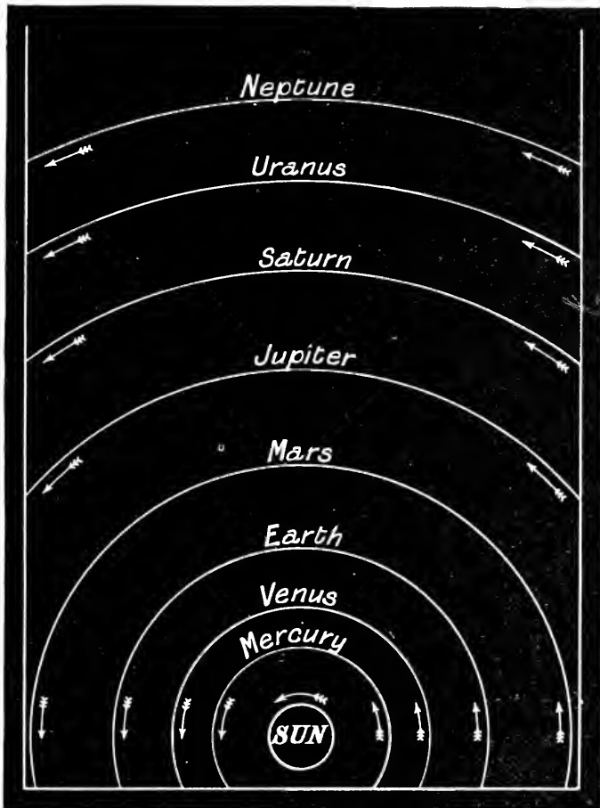
Fig. 48.—ILLUSTRATION OF THE SECOND CONCORD.
