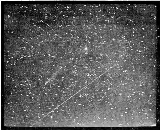
Fig. 16.—BROOKS' COMET AND METEOR TRAIL. (November 13th, 1893. Exposure 2 hours.)
