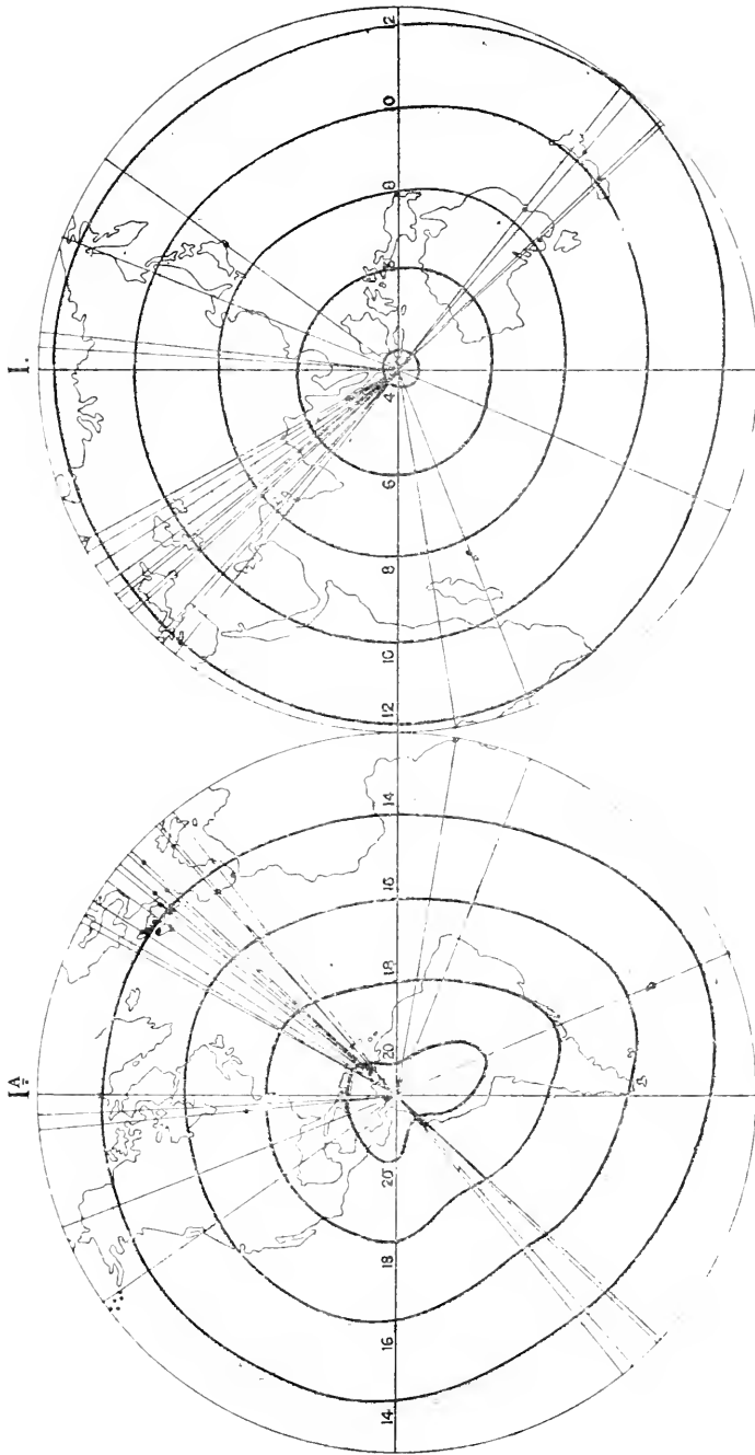
Fig. 27.—SPREAD OF THE AIR-WAVE FROM KRAKATOA TO THE ANTIPODES.
