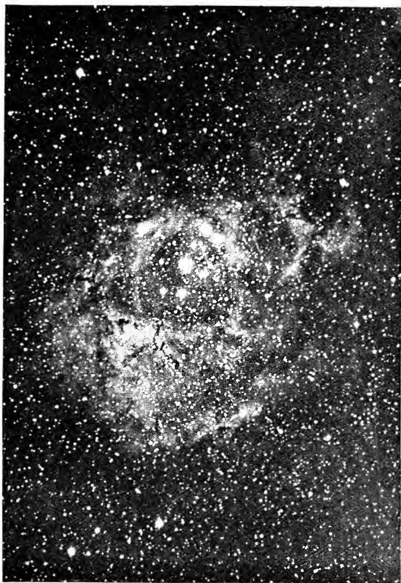
Fig. 5.—NEBULOUS REGION AND STAR CLUSTER (n.g.c. 2237-9 in Monoceros).
