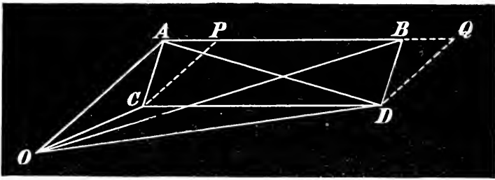
Fig. 61.—A USEFUL GEOMETRICAL PROPOSITION.
