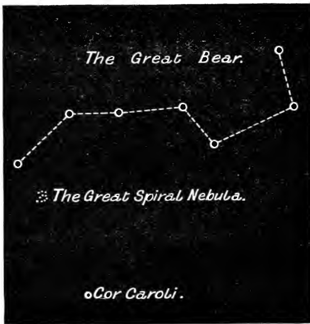
Fig. 29.—HOW TO FIND THE GREAT SPIRAL NEBULA.
