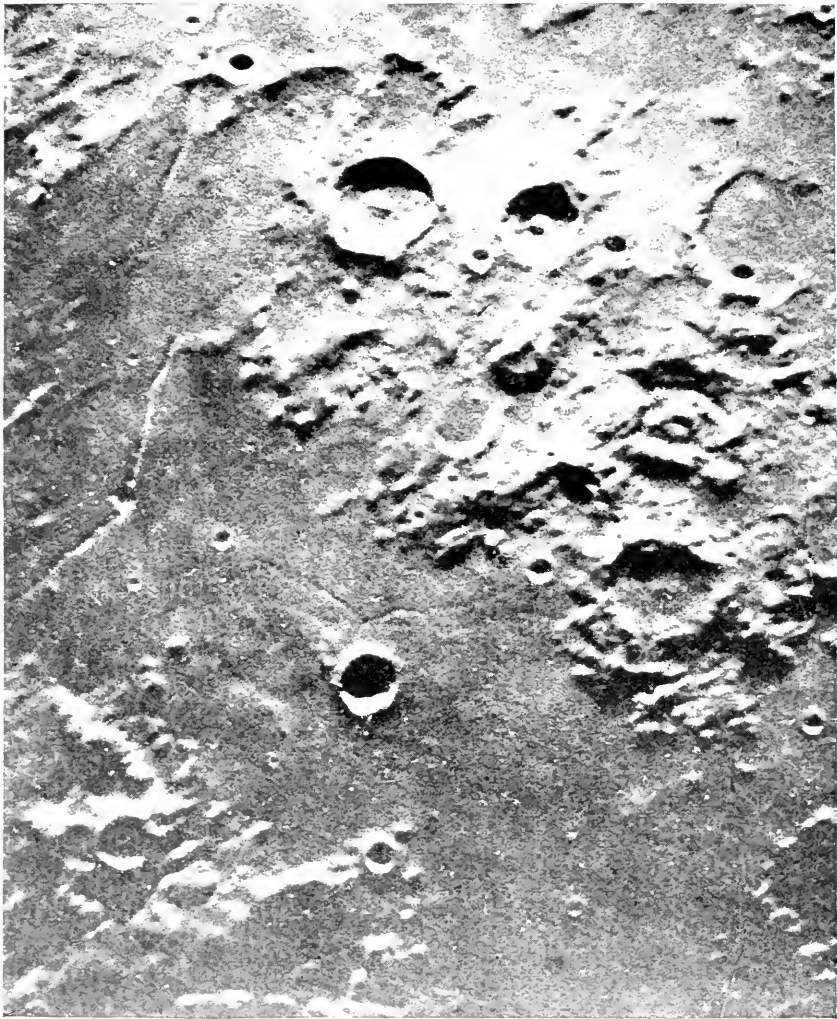
Fig. 39.—LUNAR CRATERS: HYGINUS AND ALBATEGNIUS.
