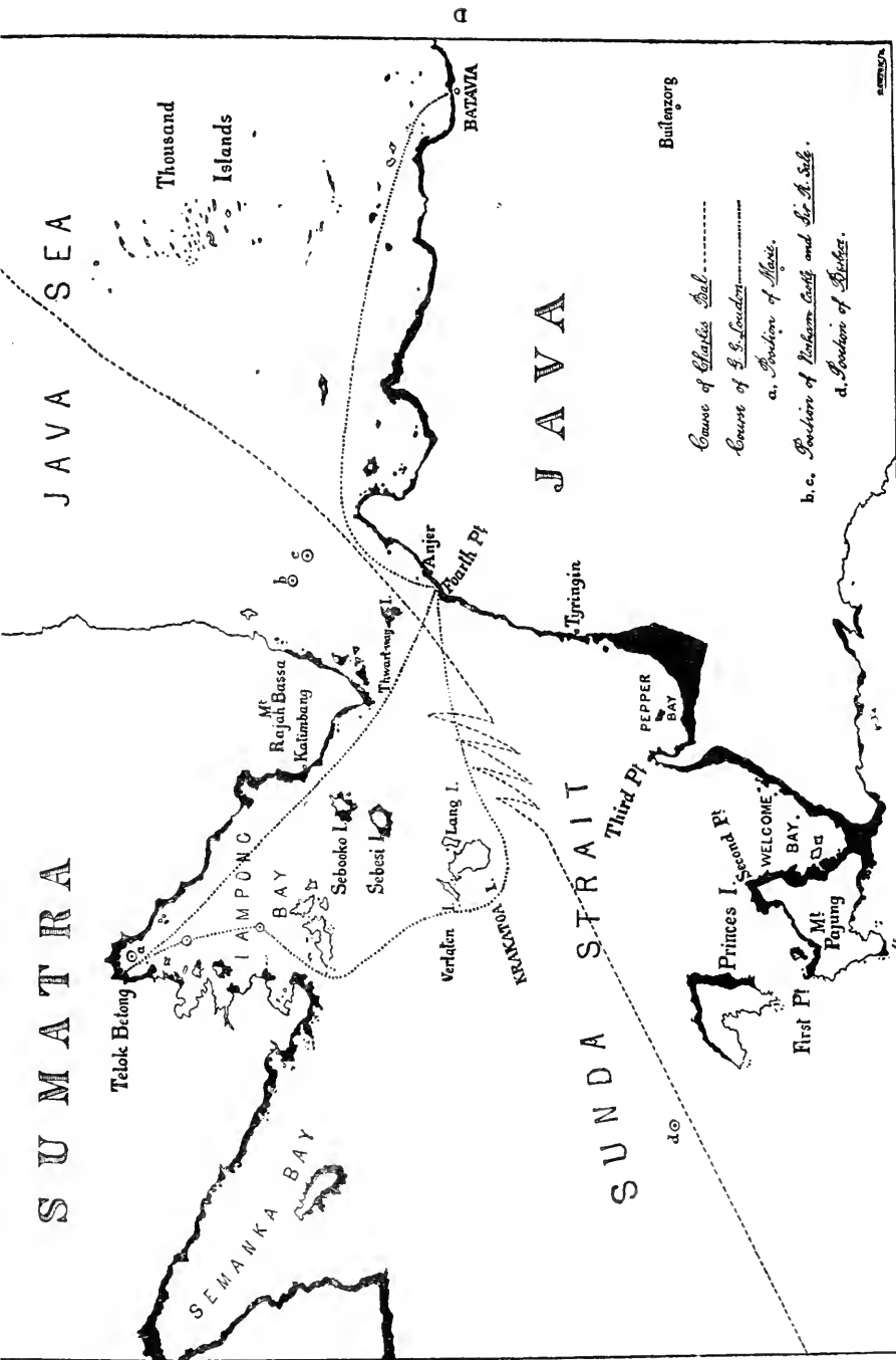
Fig. 26.—SHOWING COASTS INVADED BY THE GREAT SEA-WAVES FROM KRAKATOA. (From the Royal Society's Reports.)
