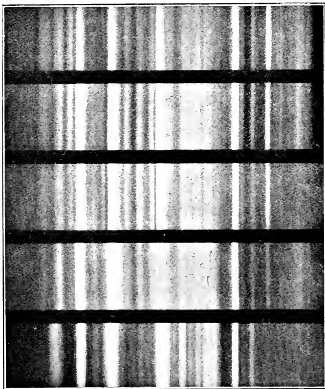
Fig. 54.—SPECTRUM OF NOVA PERSEI (1901).
