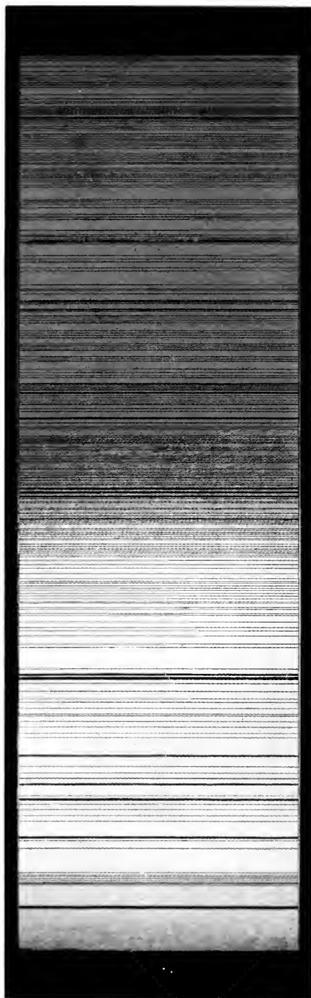
THE SOLAR SPECTRUM.
