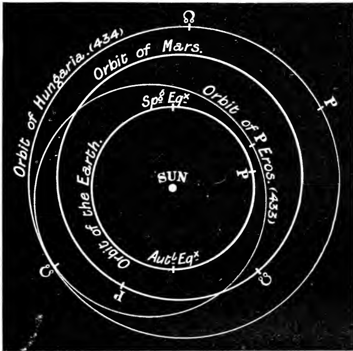
Fig. 49.—ORBITS OF EARTH, EROS AND MARS.
