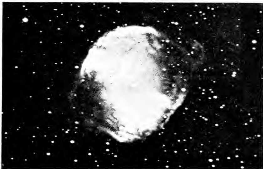
Fig. 7.—THE DUMB-BELL NEBULA (Lick Observatory, California).
