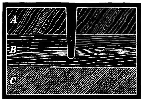
Fig. 23.—AT THE BOTTOM OF THE GREAT BORE.
