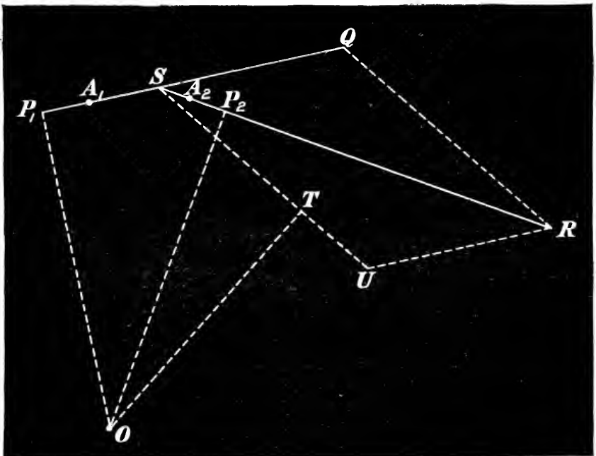
Fig. 62.—ACCELERATION OF MOMENTUM EQUALS MOMENT OF FORCE.
