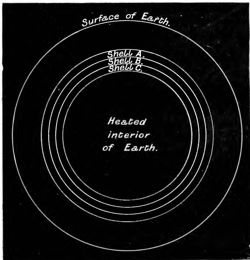
Fig. 24.—THREE CONSECUTIVE SHELLS OF THE EARTH'S CRUST.
