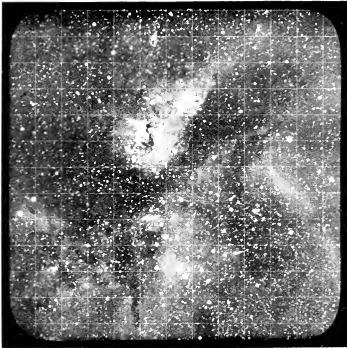
Fig. 17.—ARGO AND THE SURROUNDING STARS AND NEBULOSITY.
