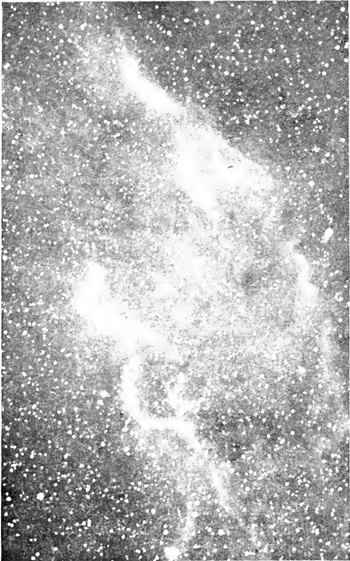
Fig. 2.—A FAINT DIFFUSED NEBULOSITY (n.g.c. 1499; in Perseus).
