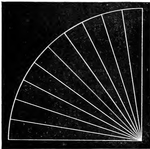
Fig. 47.—A RIGHT ANGLE DIVIDED INTO TEN PARTS.
