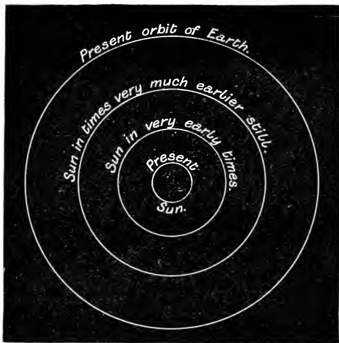
Fig. 19.—To ILLUSTRATE THE HISTORY OF THE SUN.
