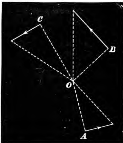
Fig. 36.—TO ILLUSTRATE MOMENT OF MOMENTUM.
