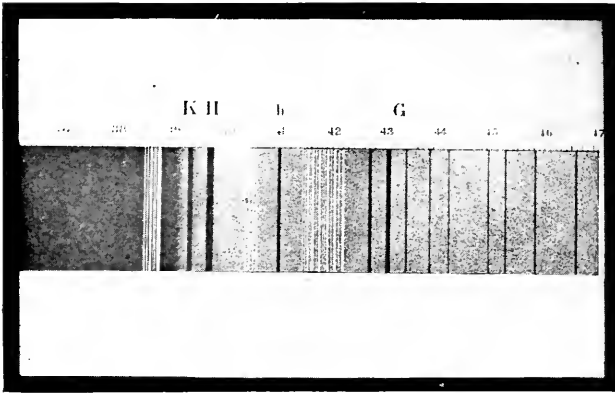
Fig. 43.—SPECTRUM OF COMET SHOWING CARBON LINES.
