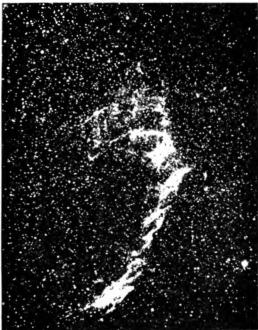
Fig. 51.—AN ELONGATED IRREGULAR NEBULA (n.g.c. 6992; in Cygnus).
