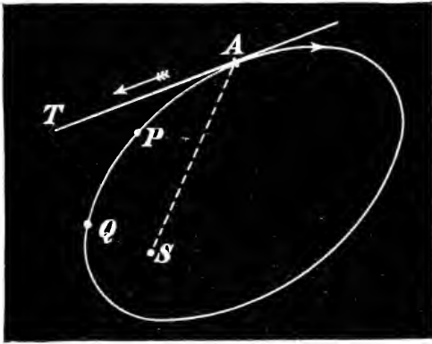
Fig. 46.—THE PLANE OF A PLANET'S ORBIT.
