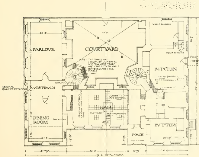
GROUND PLAN
