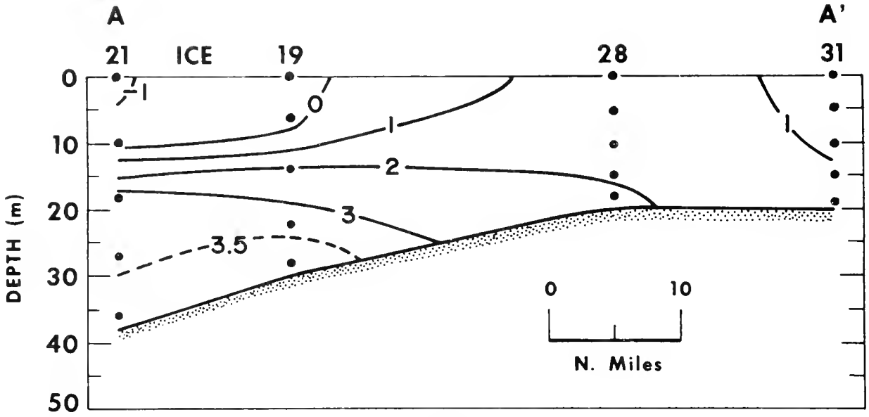
Figure 37.—Vertical profile of temperature ( ^{\circ}\text{C} ) along section A-A' (location shown in Figure 2), 1-5 October 1970, during WEBSEC-70.
