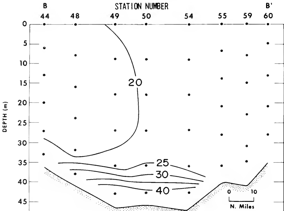
Figure 45.—Vertical profile of dissolved inorganic silicate ( \mu\text{g-at/l} ) along section B-B' (location shown in Figure 2), 8-11 October 1970, during WEBSEC-70.
