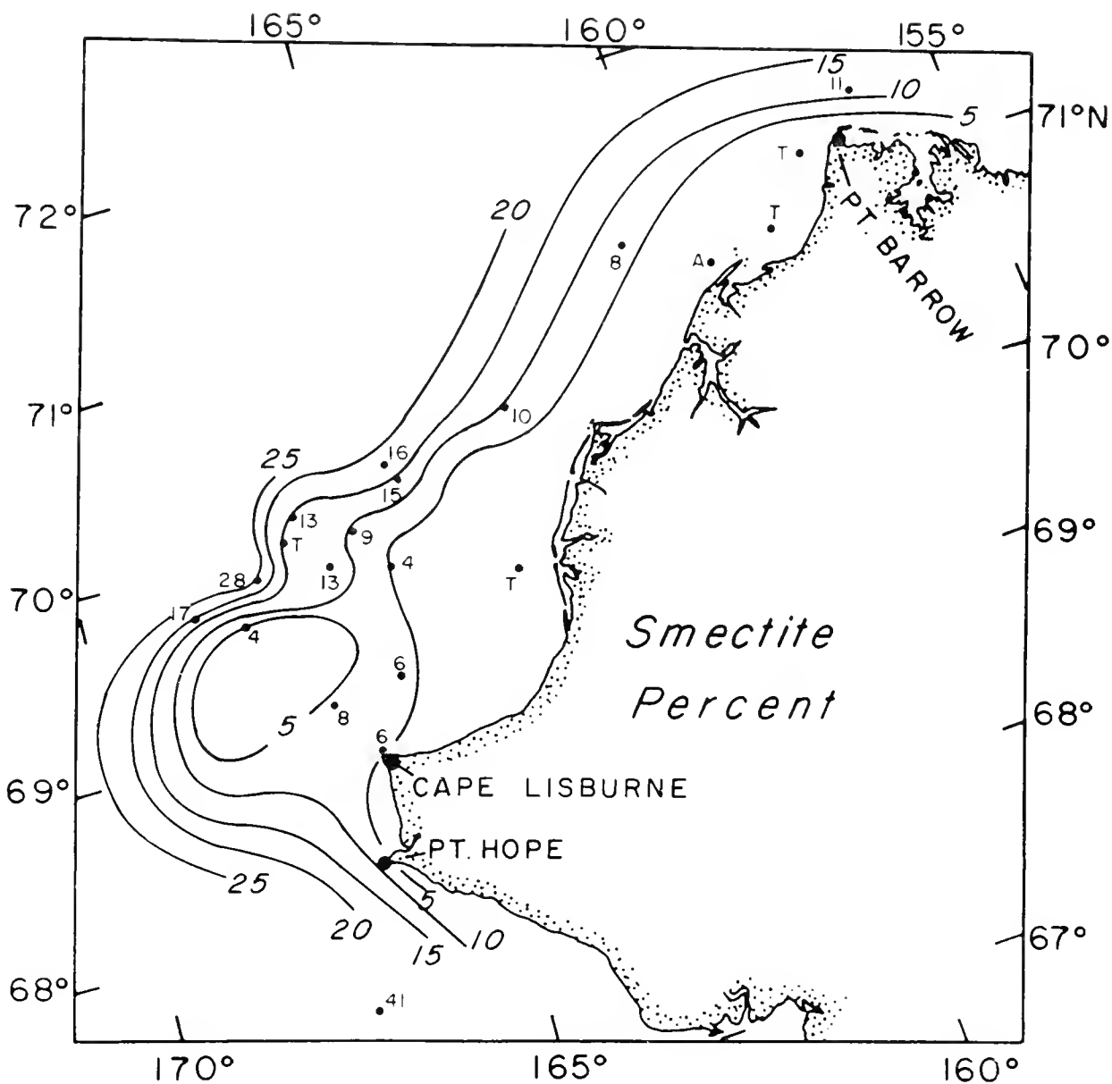
Figure 4.—Distribution of smectite concentration (%) in bottom sediments of the eastern central Chukchi Sea collected during WEBSEC-70.
