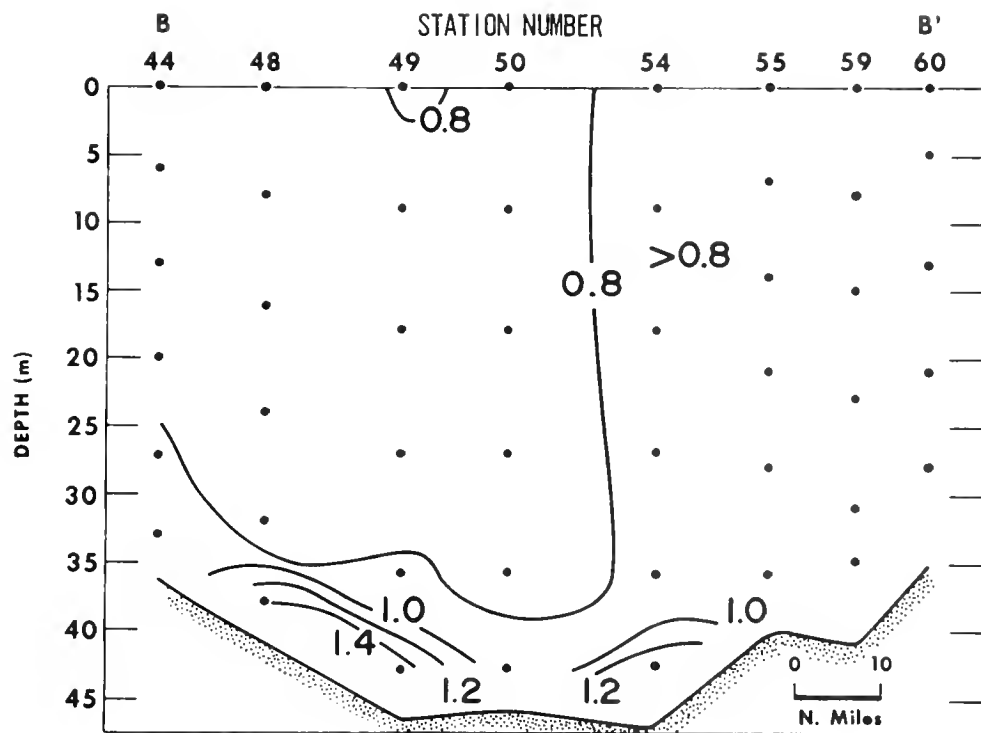
Figure 42.—Vertical profile of dissolved inorganic phosphate ( \mu\text{g-at/l} ) along section B-B' (location shown in Figure 2), 8-11 October 1970, during WEBSI C-70.
