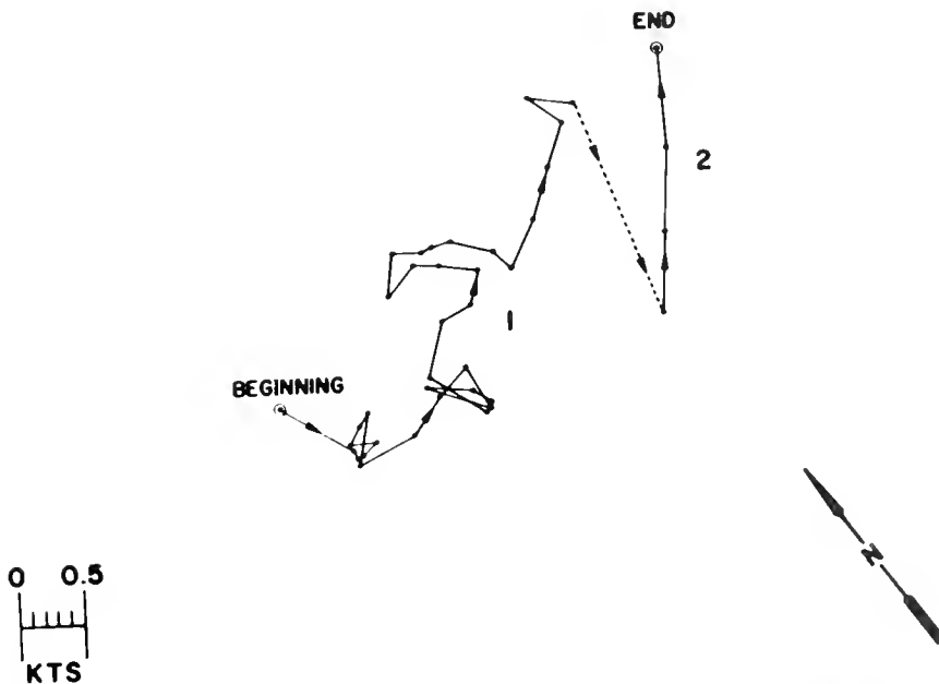
Figure 67.—Progressive vector diagram for currents at 10 m during a period of 126 minutes on station 54, WEBSEC-70, 10 October 1970. Record was digitized at 3.5-minute intervals.
