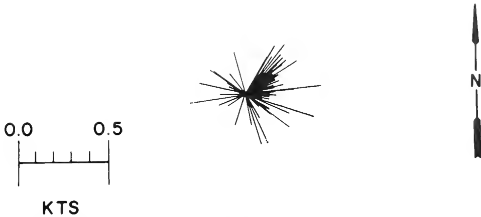
Figure 54.—Histogram of current velocities measured at 10 m during a period of 385 minutes on station 55, WEBSEC-70, 10 October 1970. Vectors are directed away from the center of the array. Record was digitized at 3.5-minute intervals.
