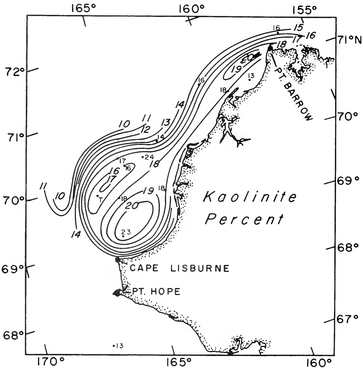
Figure 7.—Distribution of kaolinite concentration (%) in bottom sediments of the eastern central Chukchi Sea collected during WEBSEC-70.
