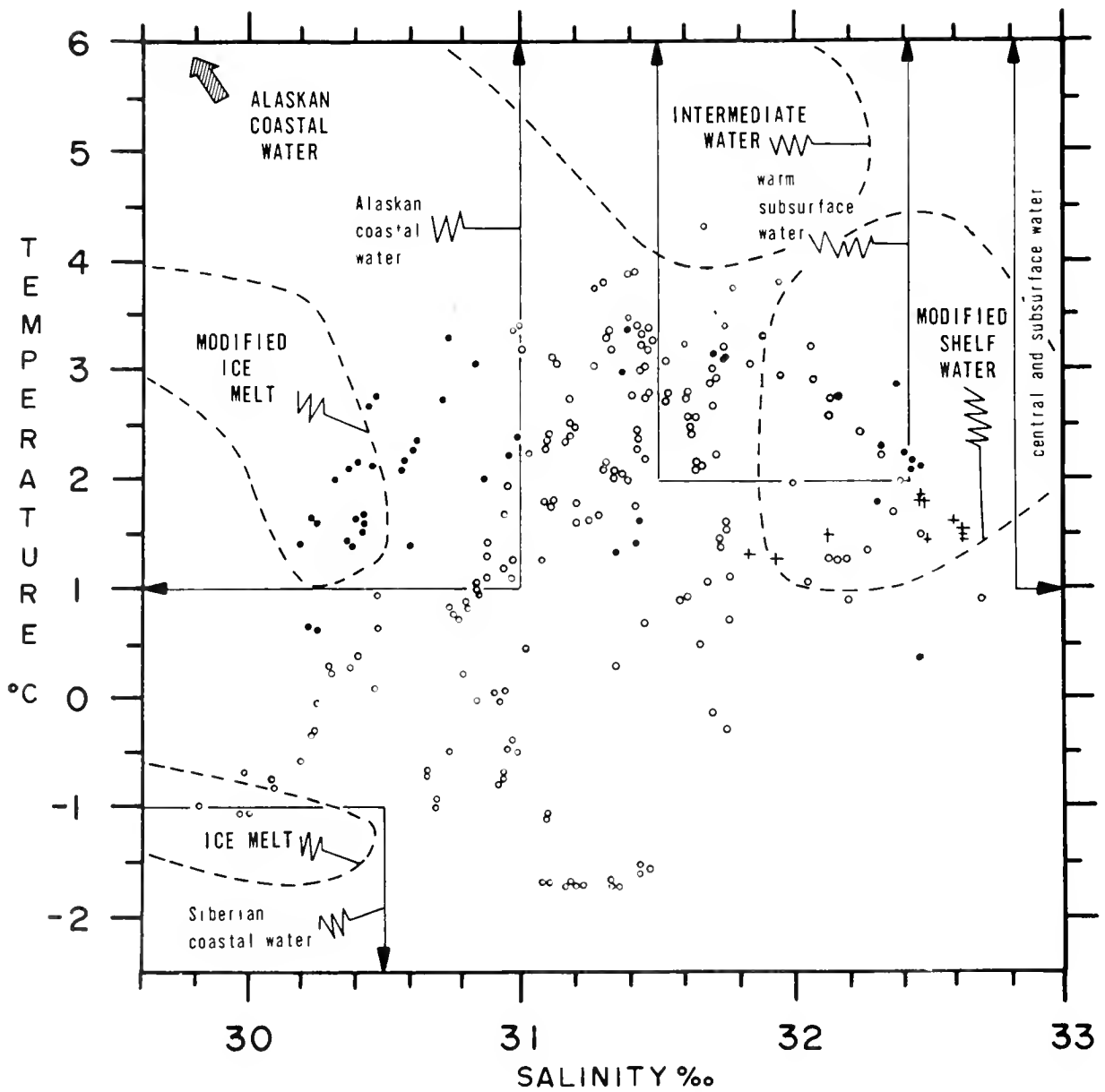
Figure 33.—Observed temperature ( ^{\circ}\text{C} )-salinity ( \text{‰} ) values during WEBSEC-70 September–October 1970 (indicated by o), and NORTHWIND, October 1962 (indicated by • for Cape Lisburne-Icy Cape and + for Bering Strait >20 m) compared with water mass classifications of previous investigators (Saur, et al., 1954 indicated ----- and capital letters, and Aagaard, 1964 indicated by ——— and lower case letters).
