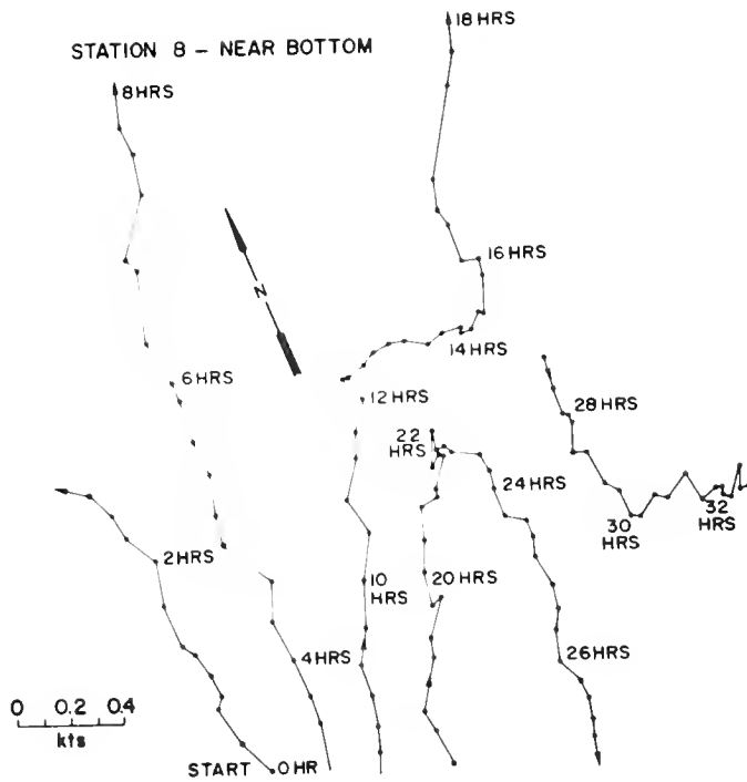
Figure 74.—Progressive vector diagram for currents near bottom during a period of 33 hours on station 8, WEBSEC-70, 25 September 1970. Vectors represent 15-minute averages.
