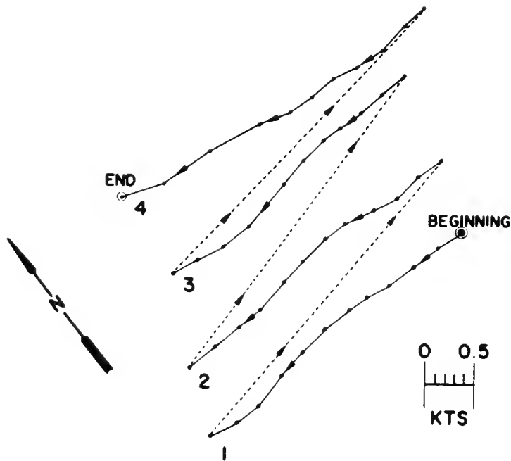
Figure 65.—Progressive vector diagram for currents at 10 m during a period of 164 minutes on station 49, WEBSEC-70, 9 October 1970. Record was digitized at 3.5-minute intervals.
