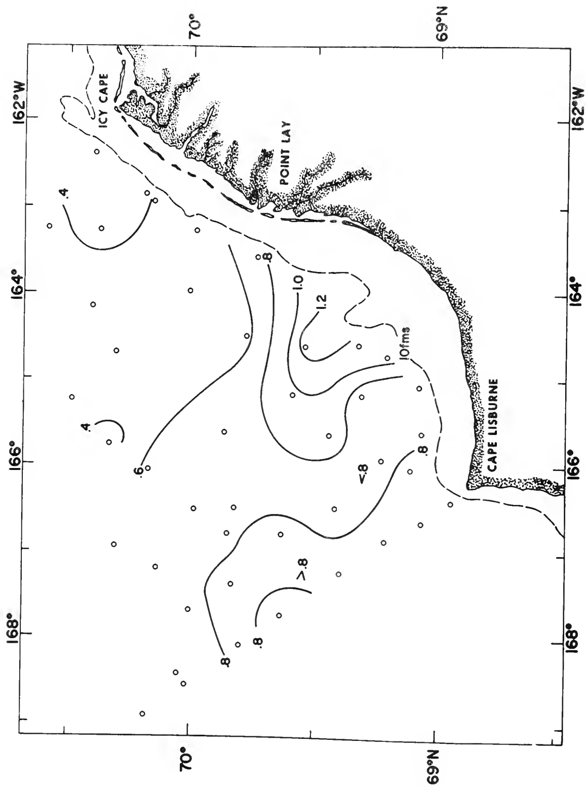
Figure 19.—Concentration of dissolved inorganic phosphate ( \mu\text{g-at/l} ) at the sea surface during WEBSEC-70, 25 September-17 October 1970.
