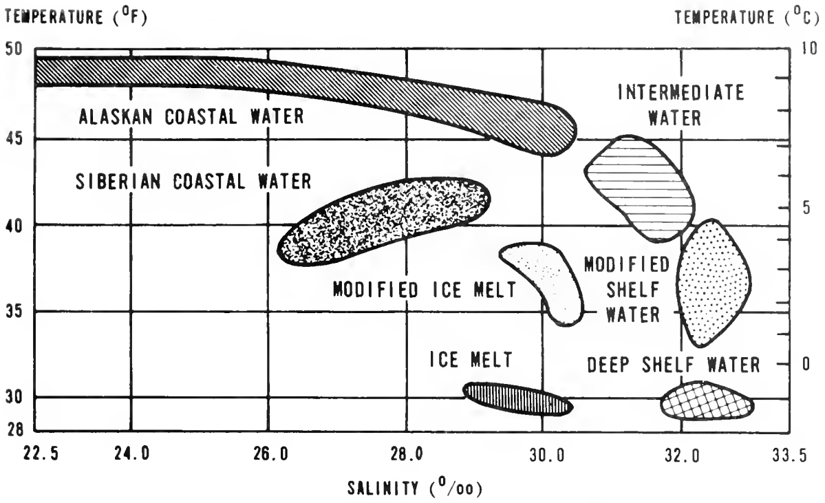
Figure 34.—Water mass classifications for the eastern Bering and Chukchi seas (from Saur, et al., 1954).
