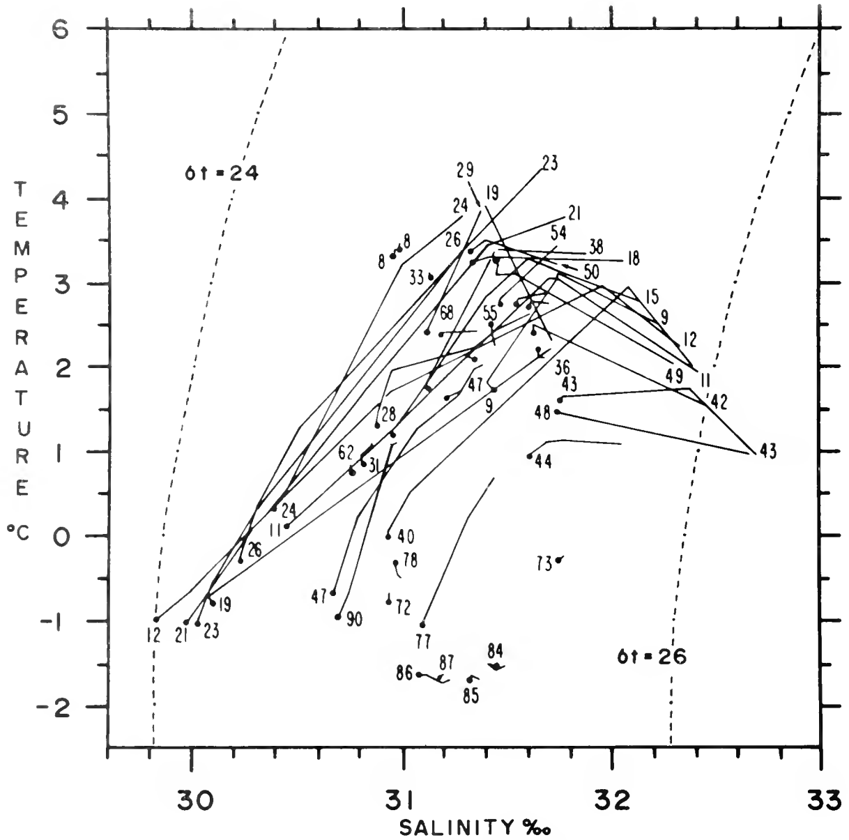
Figure 35.—Temperature (°C)—salinity (‰) regressions from WEBSEC-70 observations (25 September–17 October, 1970). Dots indicate surface values. Numbers are station numbers.
