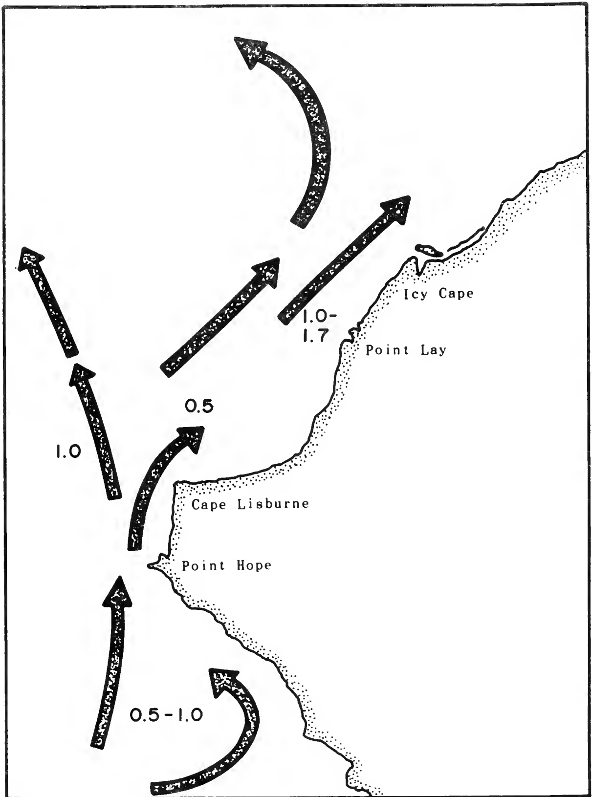
Figure 4.—Average surface current velocities (from USNHO Oceanographic Atlas of the Polar Seas—Part II, 1968).
