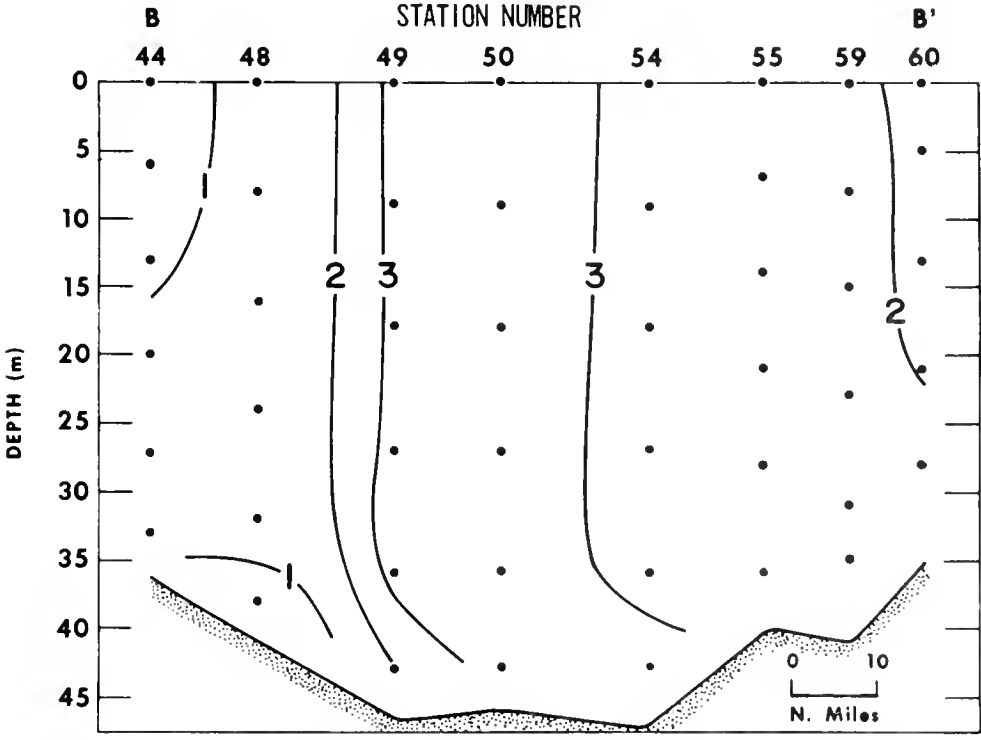
Figure 39.—Vertical profile of temperature (°C) along section B-B' (location shown in Figure 2), 8-11 October 1970, during WEBSEC-70.
