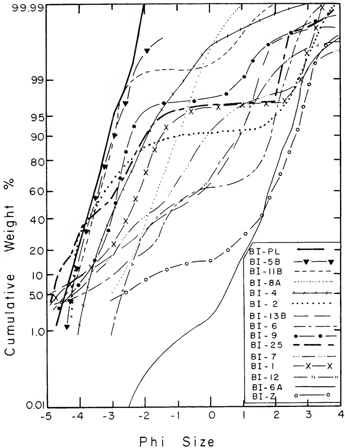
Figure 3.—Size distribution of barrier beach sediments collected at Point Lay on 25 September 1970 during WEBSEC-70.
