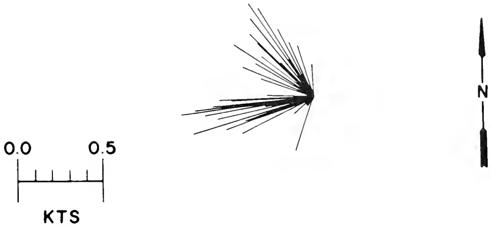
Figure 58.—Histogram of current velocities measured at 10 m during a period of 206 minutes on station 73, WEBSEC-70, 14 October 1970. Vectors are directed away from the apex of the array. Record was digitized at 3.5-minute intervals.
