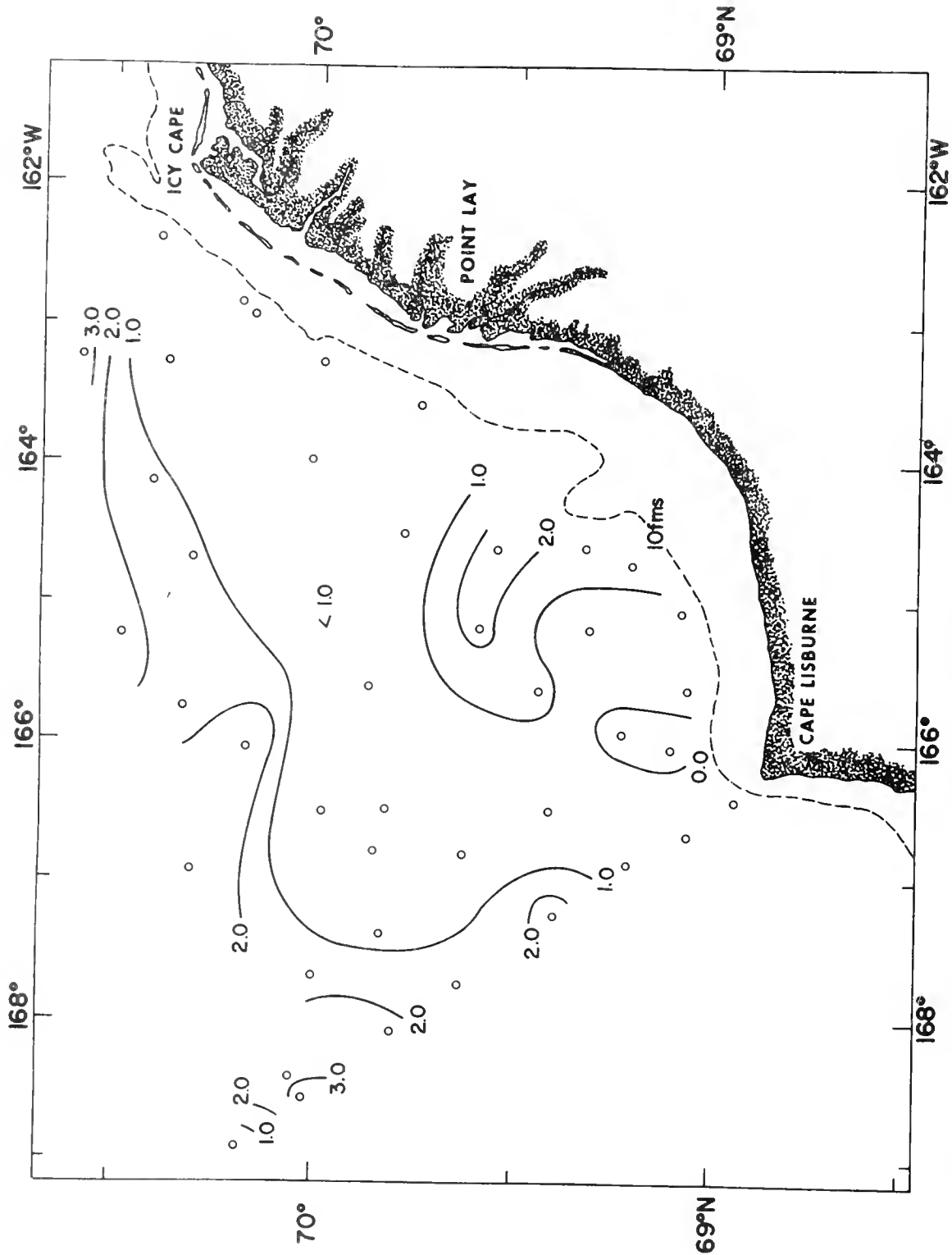
Figure 27.—Concentration of dissolved nitrite ( \mu\text{g-at/l} ) near bottom during WEBSEC-70, 25 September-17 October 1970.
