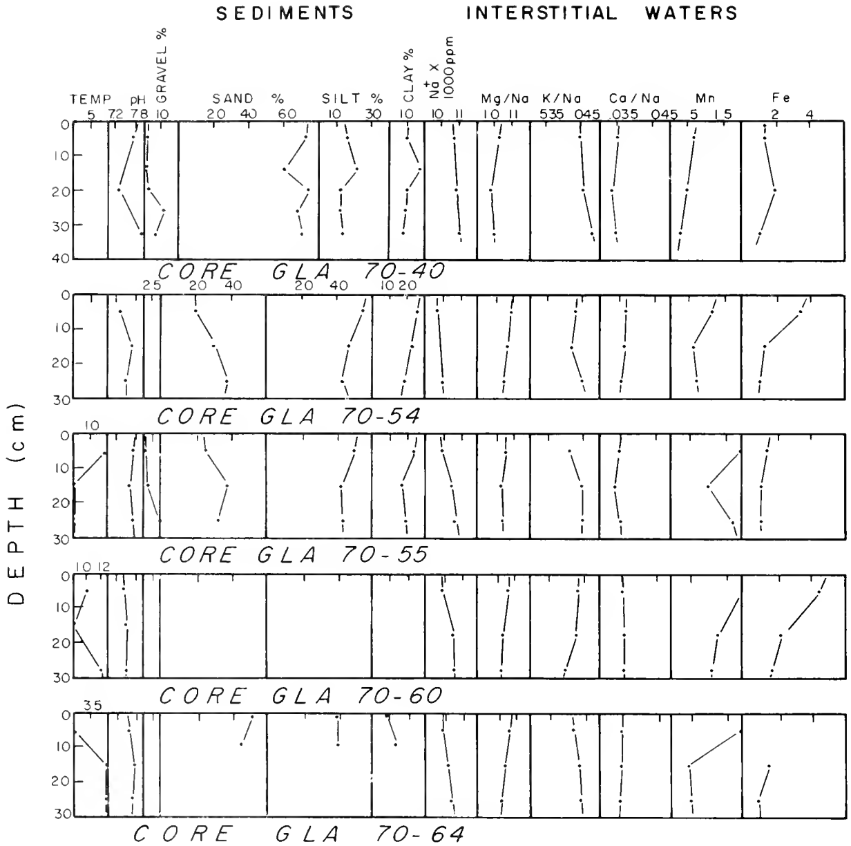
Figure 9.—Relationship between the concentrations of metal ions in interstitial waters and the pH, temperature, and texture of bottom sediments of the eastern central Chukchi Sea collected during WEBSEC-70, stations 40, 54, 55, 60 and 64.
