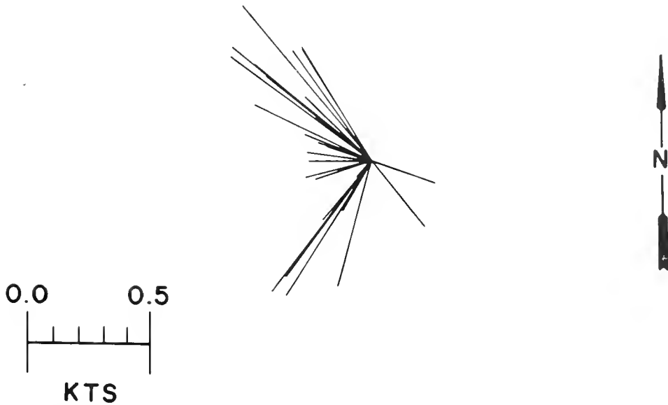
Figure 55.—Histogram of current velocities measured at 10 m during a period of 123 minutes on station 59, WEBSEC-70, 11 October 1970. Vectors are directed away from the apex of the array. Record was digitized at 3.5-minute intervals.
