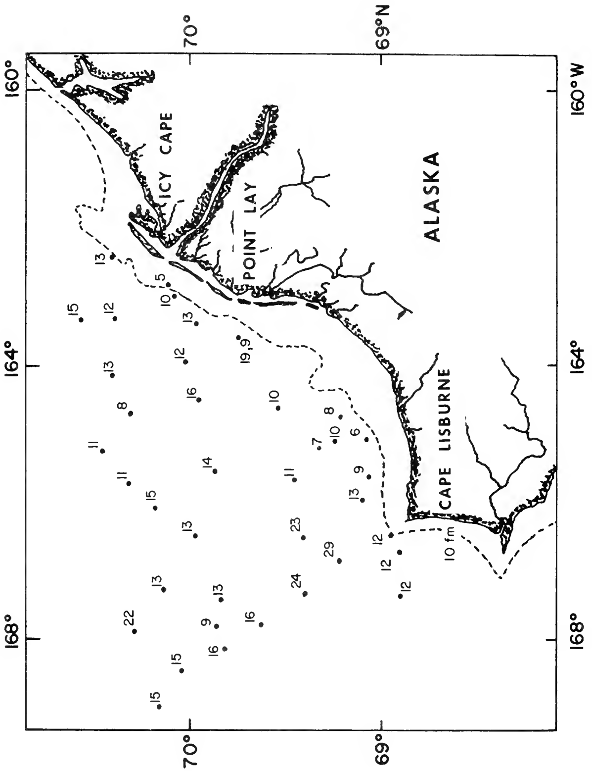
Figure 2.—Number of zooplankton species collected at each station by vertical net tows during WEBSEC-70.
