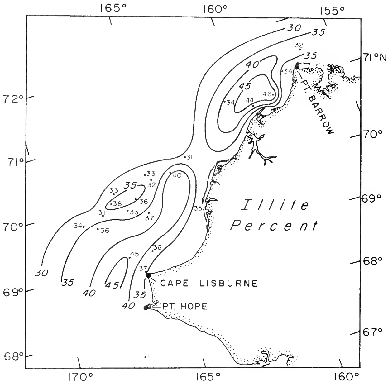
Figure 5.—Distribution of illite concentration (%) in bottom sediments of the eastern central Chukchi Sea collected during WEBSEC-70.
