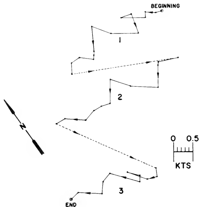
Figure 69.—Progressive vector diagram for currents at 10 m during a period of 123 minutes on station 59, WEBSEC-70, 11 October 1970. Record was digitized at 3.5-minute intervals.
