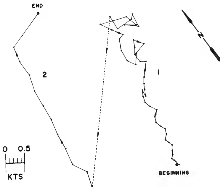
Figure 63.—Progressive vector diagram for currents at 10 m during a period of 210 minutes on station 29, WEBSEC-70, 4 October 1970. Record was digitized at 3.5-minute intervals.
