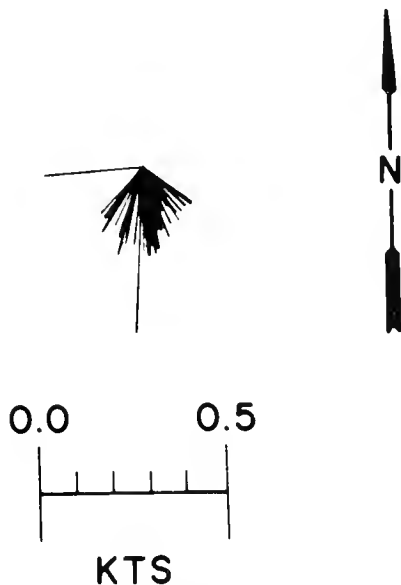
Figure 47. —Histogram of current velocities measured at 10 m during a period of 308 minutes on station 26, WEBSEC-70, 3 October 1970. Vectors are directed away from the apex of the array. Record was digitized at 3.5-minute intervals.
