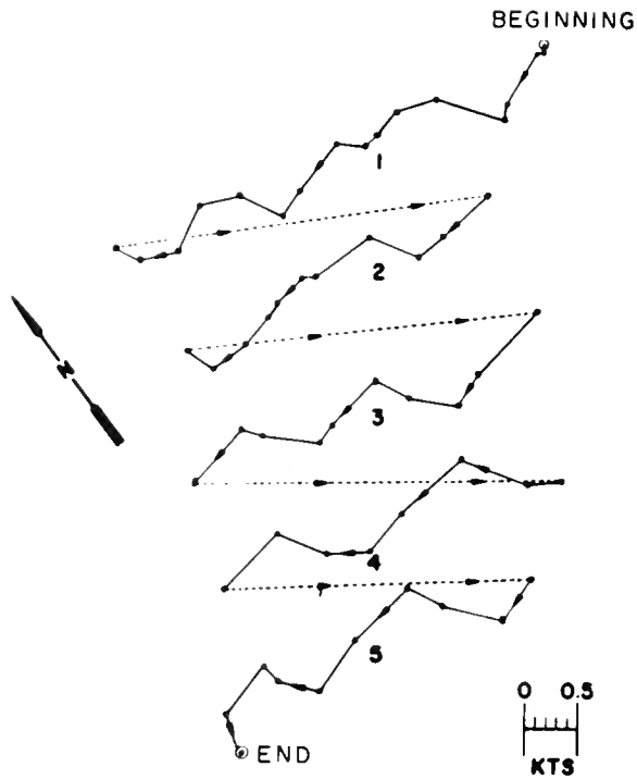
Figure 72.—Progressive vector diagram for currents at 10 m during a period of 206 minutes on station 73, WEBSEC-70, 14 October 1970. Record was digitized at 3.5-minute intervals.
