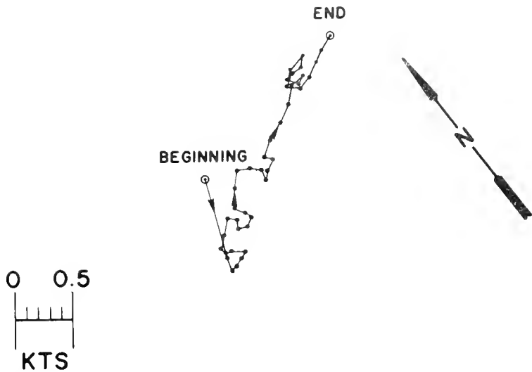
Figure 62.—Progressive vector diagram for currents at 10 m during a period of 165 minutes on station 28, WEBSEC-70, 4 October 1970. Record was digitized at 3.5-minute intervals.
