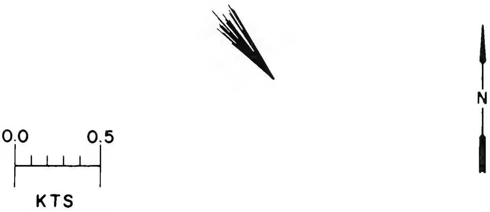
Figure 59.—Histogram of current velocities measured at 10 m during a period of 144 minutes on station 90, WEBSEC-70, 17 October 1970. Vectors are directed away from the apex of the array. Record was digitized at 3.5-minute intervals.
