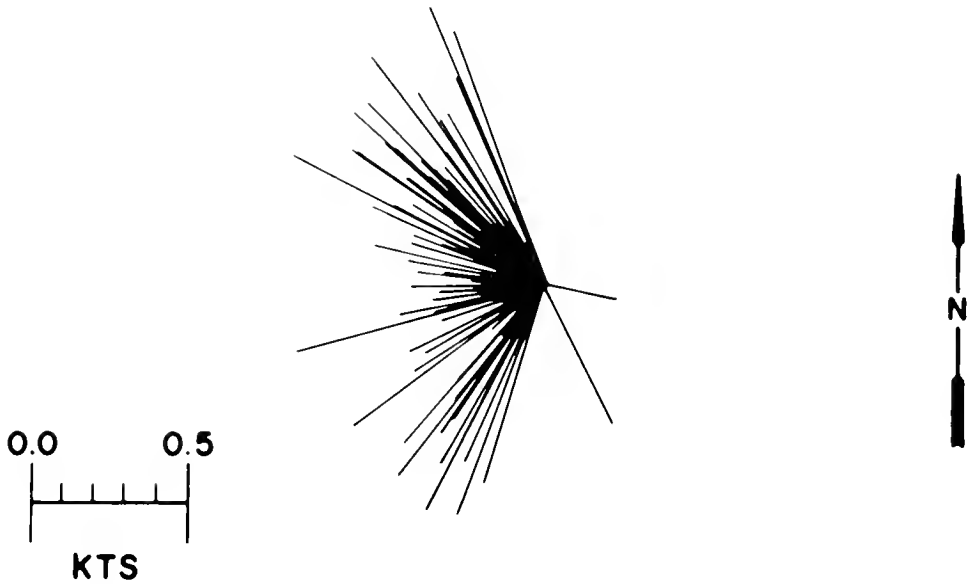
Figure 56.—Histogram of current velocities measured at 10 m during a period of 329 minutes on station 60, WEBSEC-70, 11 October 1970. Vectors are directed away from the apex of the array. Record was digitized at 3.5-minute intervals.
