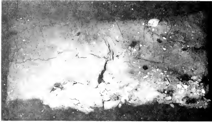
Figure 7a. —Radiograph of 1-cm thick slab of box core from station 79. Note worm tubes, rounded pebbles and shell material. The bottom of the core has higher sand and gravel content. The distance across the core is 30 cm.
