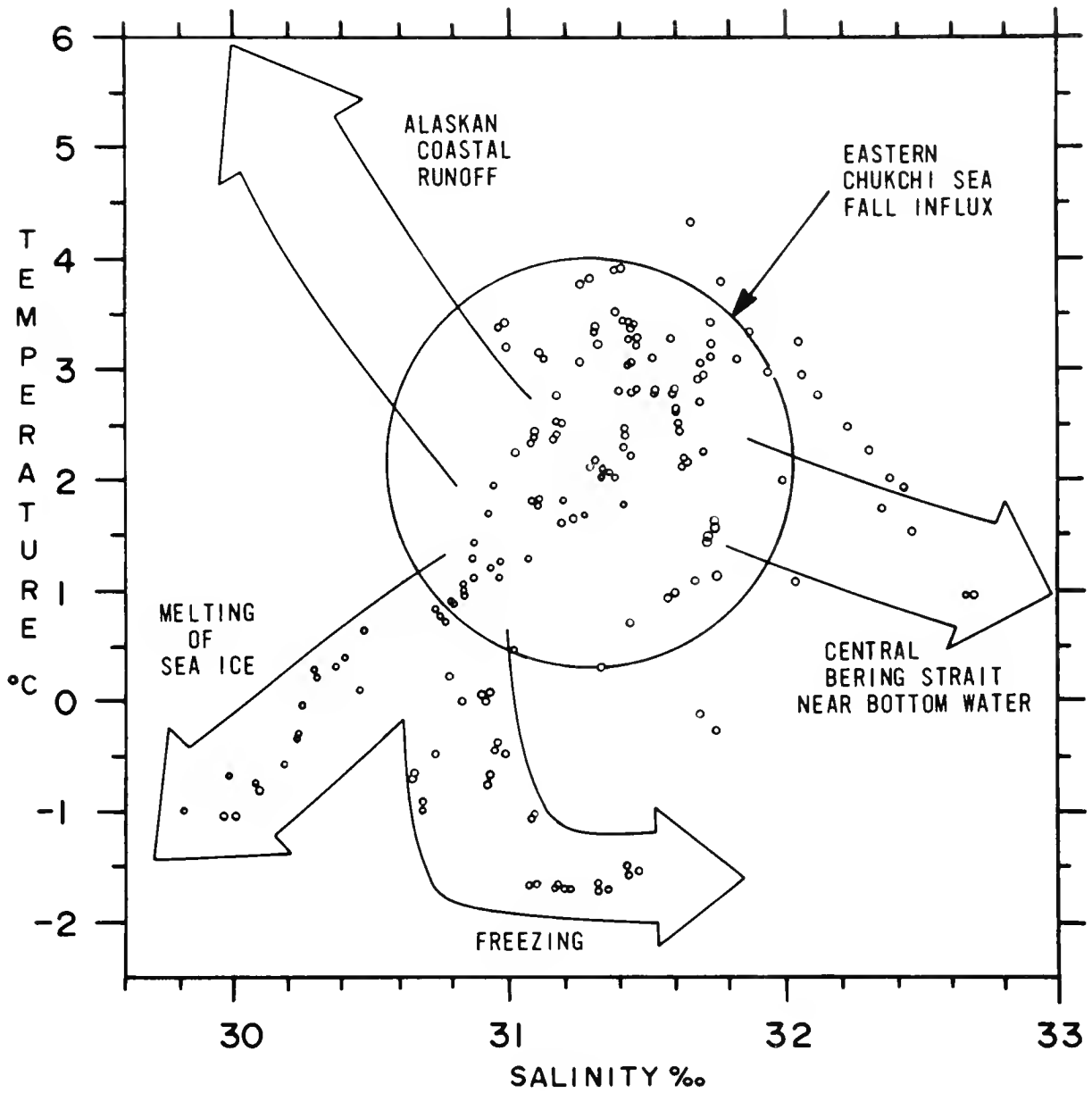
Figure 36.—Observed temperature (°C)-salinity (‰) values during WEBSEC-70, September-October 1970 and processes or water masses influencing the properties of Eastern Chukchi Sea Fall Influx.
