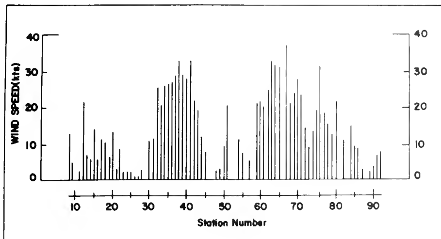
Figure 32.—Surface wind velocity during WEBSEC-70, 25 September-17 October 1970.
