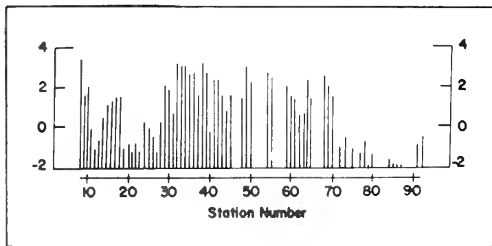
Figure 7.—Sea surface temperature (°C) during WEBSEC-70, 25 September-17 October 1970.
