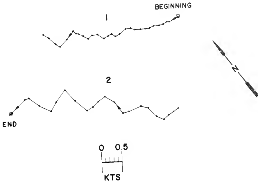
Figure 66.—Progressive vector diagram for currents at 10 m during a period of 200 minutes on station 50, WEBSEC-70, 9 October 1970. Record was digitized at 3.5-minute intervals.
