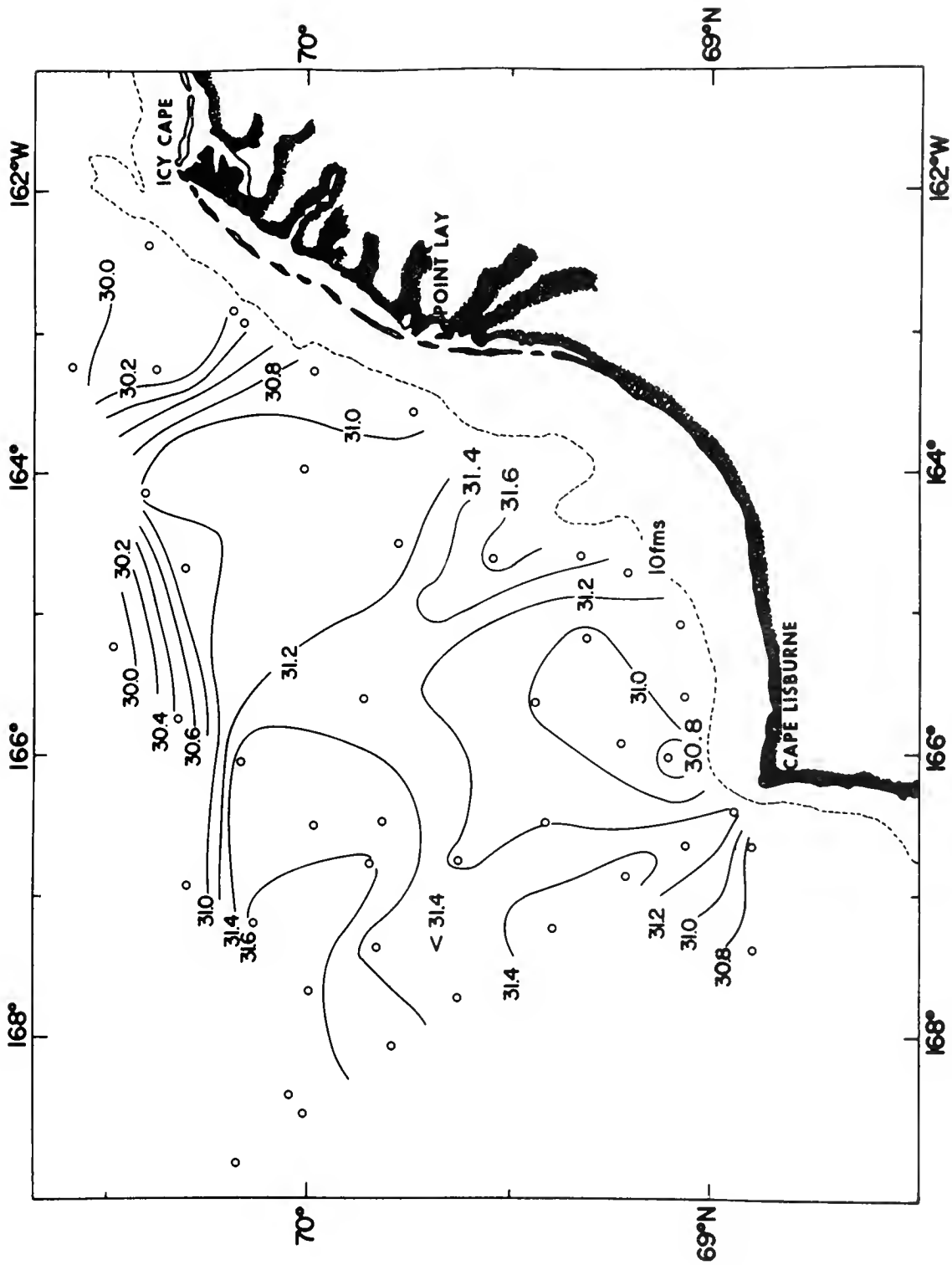
Figure 10.—Sea surface salinity (‰) during WEBSEC-70, 25 September–17 October 1970.
