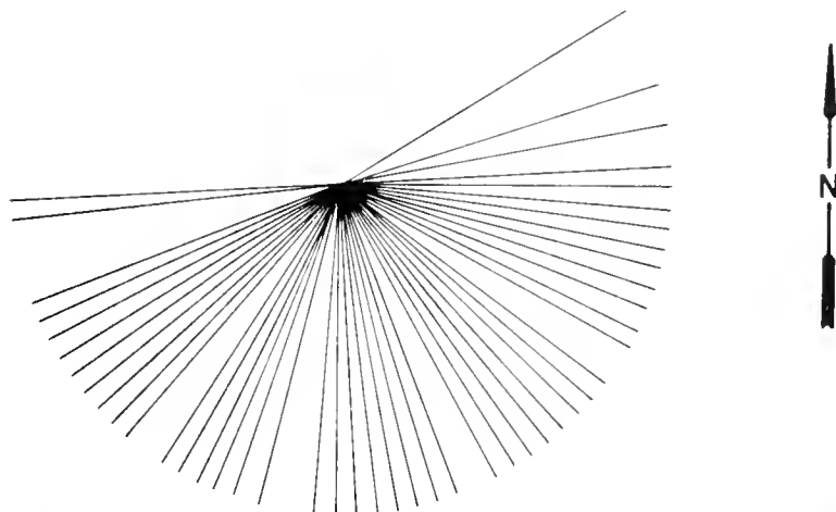
Figure 46. —Histogram of current direction measured at 10 m during a period of 31 hours on station 8, WEBSEC-70, 25 September 1970. The speed record proved to be unreliable on that station, so an arbitrary, constant speed has been assigned for display purposes. Vectors are directed away from the center of the array. Because of the length of the record, it was digitized only at 17.5-minute intervals.
