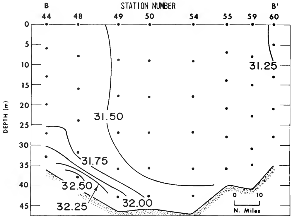
Figure 40.—Vertical profile of salinity (‰) along section B-B' (location shown in Figure 2), 8-11 October 1970, during WEBSEC-70.
