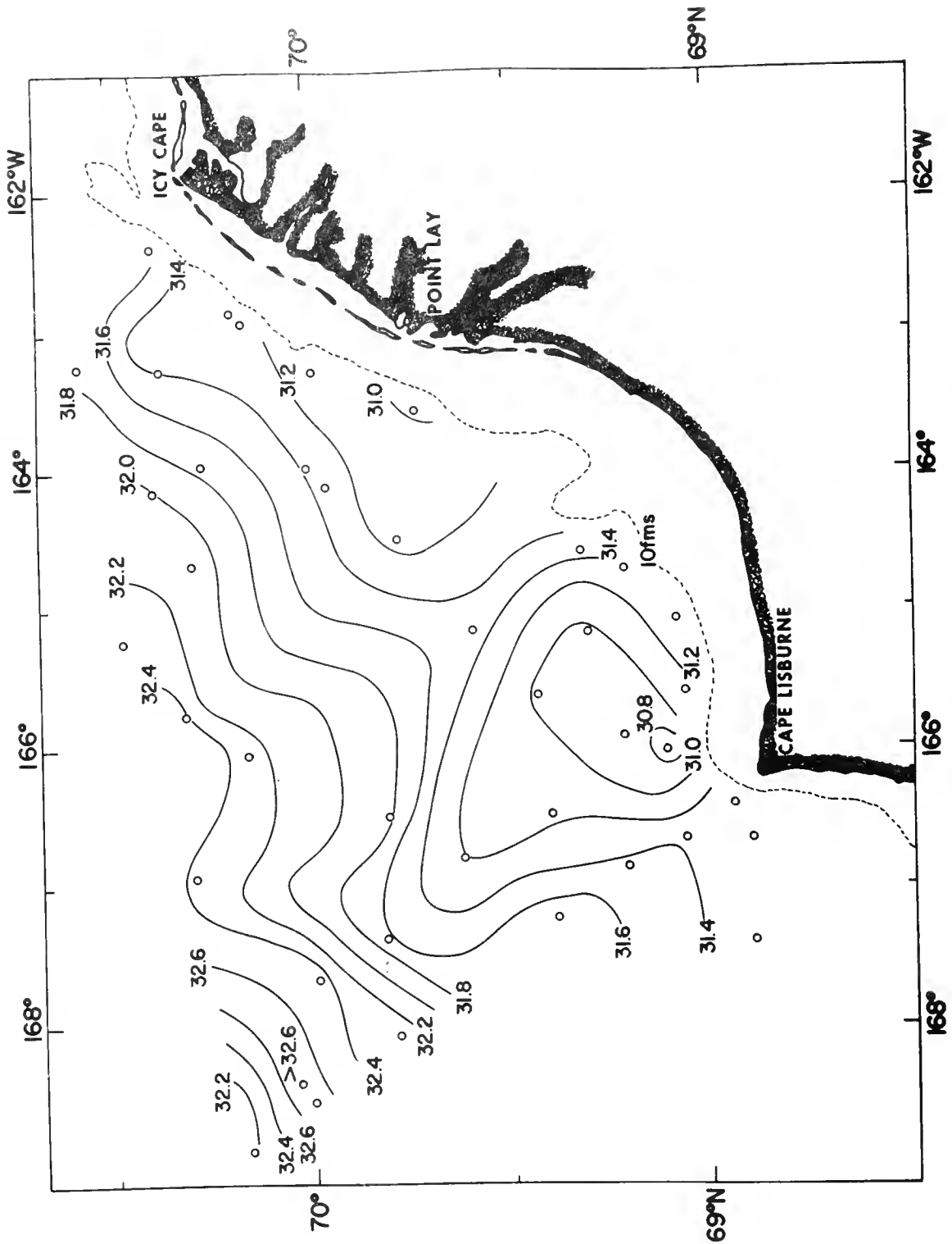
Figure 12.—Near-bottom salinity (‰) during WEBSEC-70, 25 September–17 October 1970.
