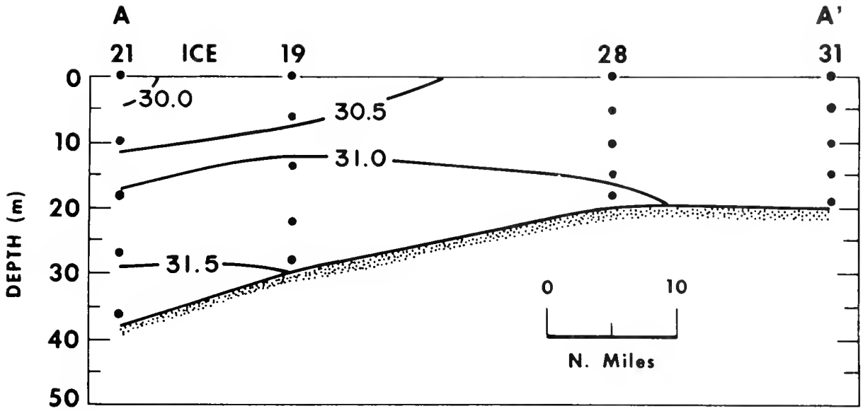
Figure 38.—Vertical profile of salinity (‰) along section A-A' (location shown in Figure 2), 1-5 October 1970, during WEBSEC-70.
