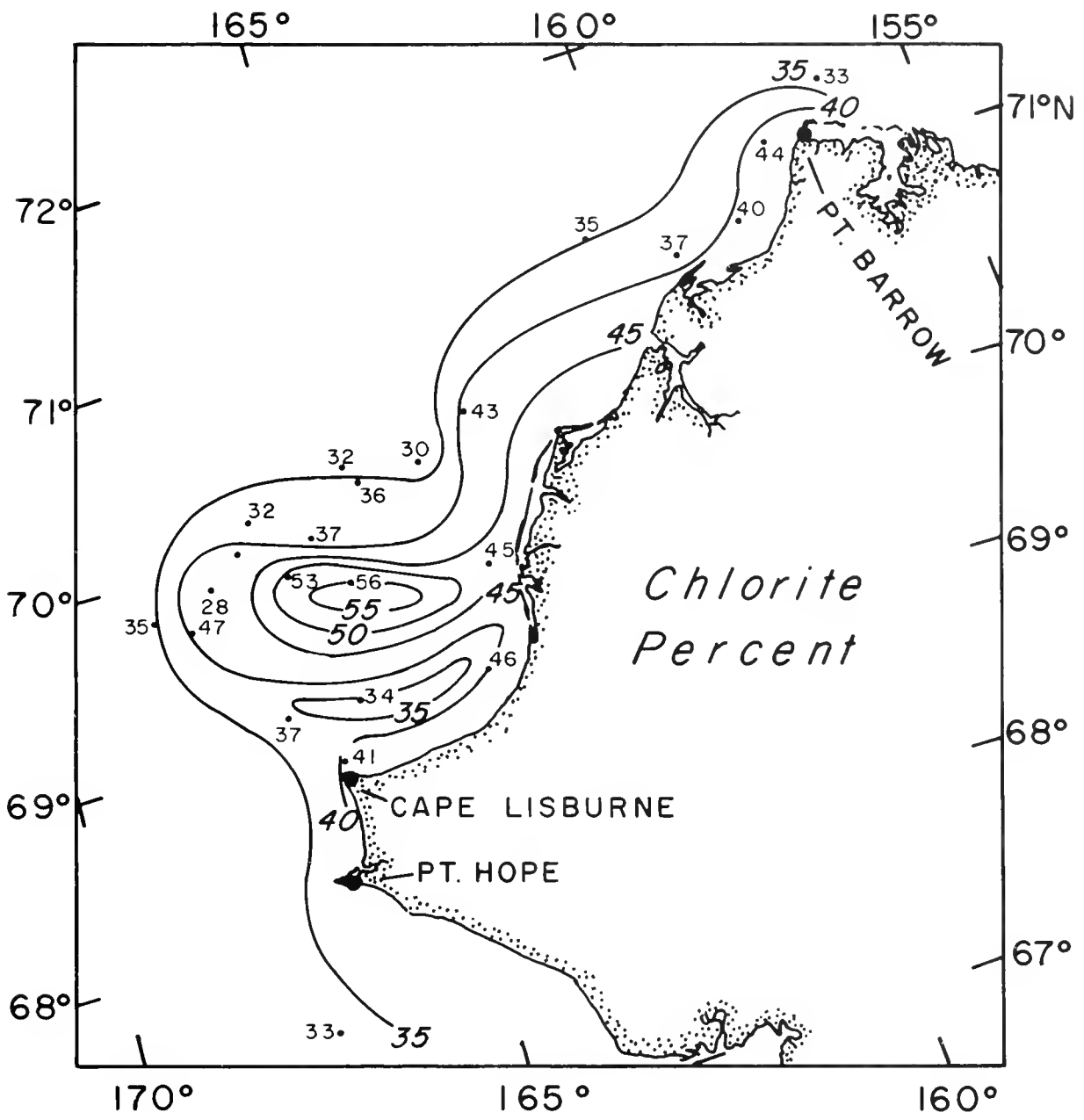
Figure 6.—Distribution of chlorite concentration (%) in bottom sediments of the eastern central Chukchi Sea during WEBSEC-70.
