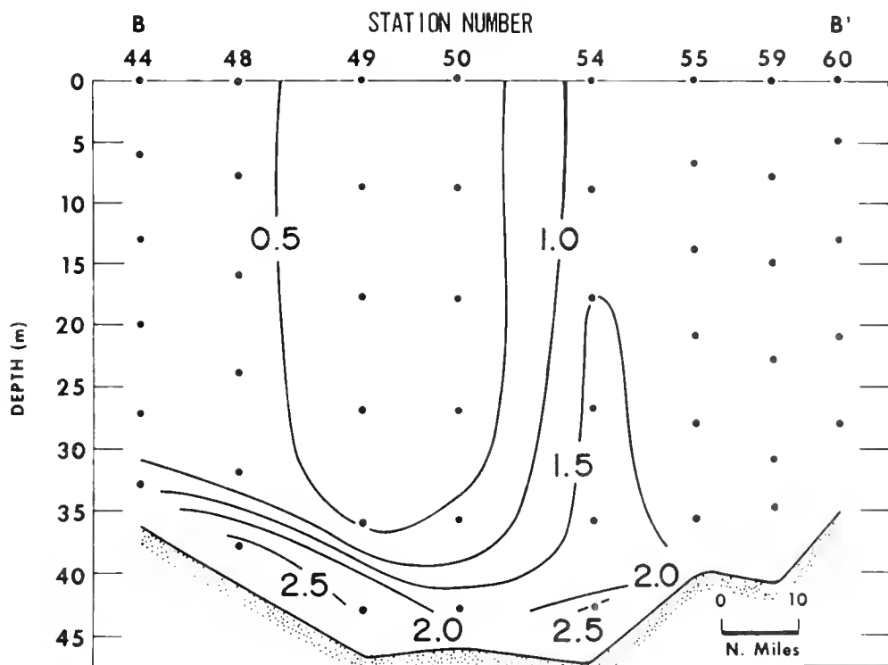
Figure 43.—Vertical profile of dissolved inorganic nitrate ( \mu\text{g-at/l} ) along section B-B' (location shown in Figure 2), 8-11 October 1970, during WEBSEC-70.
