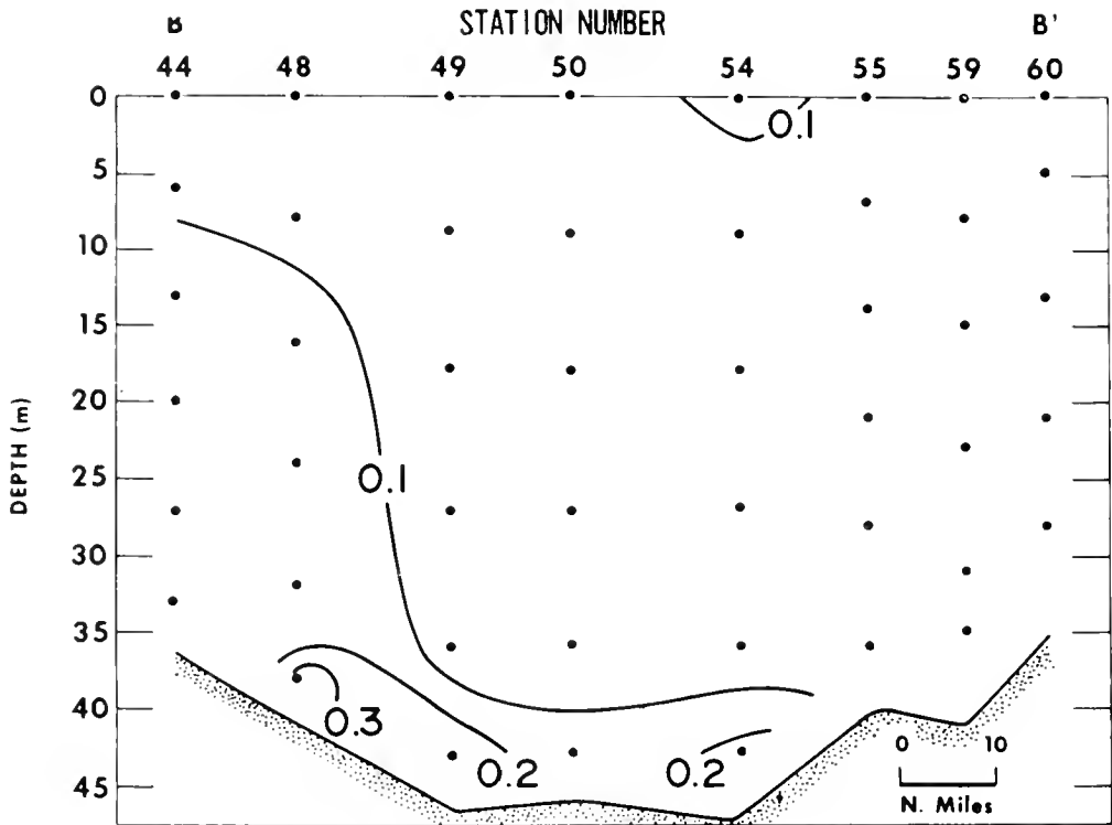
Figure 44.—Vertical profile of dissolved inorganic nitrite ( \mu\text{g-at/l} ) along section B-B' (location shown in Figure 2), 8-11 October 1970, during WEBSEC-70.
