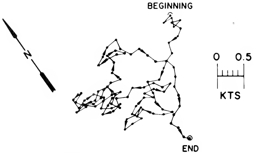
Figure 60.—Progressive vector diagram for currents at 10 m during period of 31 hours on station 8, WEBSEC-70, 25 September 1970. The speed record proved to be unreliable on that station, so an arbitrary, constant speed has been assigned for display purposes. Because of the length of the record, it was digitized only at 17.5-minute intervals.
