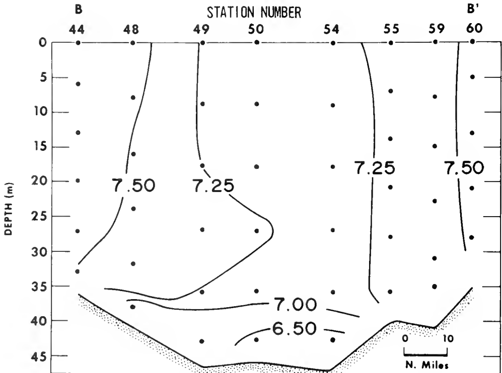
Figure 41.—Vertical profile of dissolved oxygen (ml/l) along section B-B' (location shown in Figure 2), 8-11 October 1970, during WEBSEC-70.
