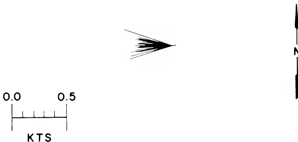
Figure 51.—Histogram of current velocities measured at 10 m during a period of 164 minutes on station 49, WEBSEC-70, 9 October. Vectors are directed away from the apex of the array. Record was digitized at 3.5-minute intervals.
