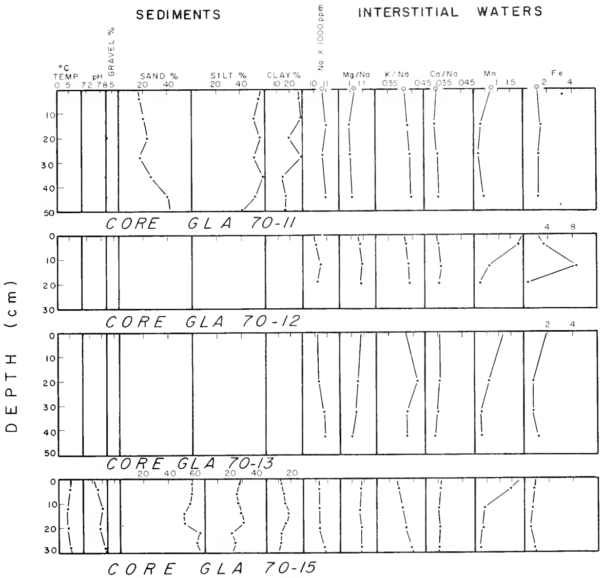
Figure 8.—Relationship between the concentrations of metal ions in interstitial waters and the pH, temperature, and texture of bottom sediments of the eastern central Chukchi Sea collected during WEBSEC-70, stations 11, 12, 13 and 15.
