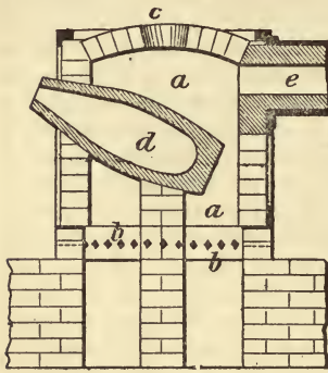
FIG. 157.—REFINING RETORT.
