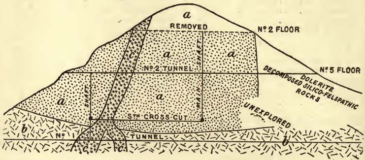
FIG. 125.—GOLD DEPOSITS, MOUNT MORGAN.
