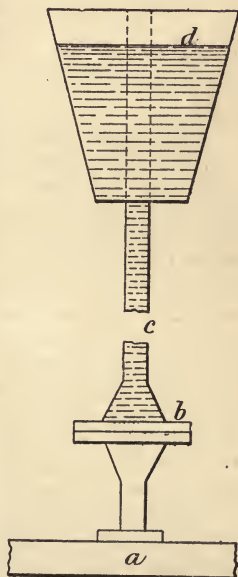
FIG. 15.—AIR VALVE FOR SIPHON.
