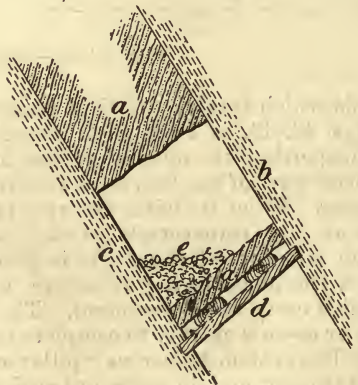
FIG. 47. STEEP COAL VEIN: GOOD ROOF.
