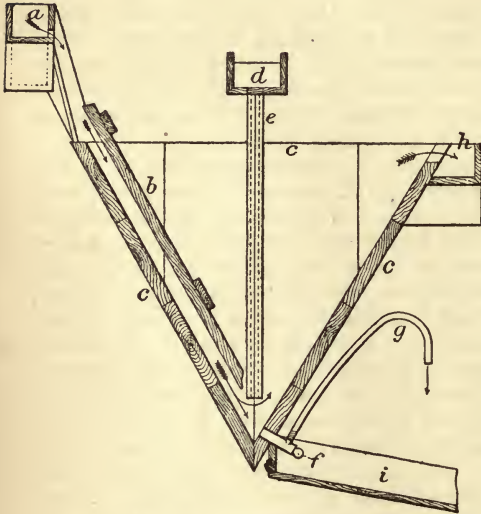
FIG. 72.—POINTED BOX.
