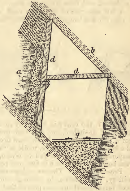
FIG. 48.—TIMBERING ROAD-WAY IN COAL.
