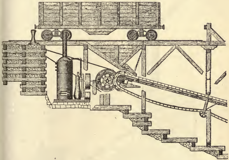
FIG. 62.—COAL CONVEYOR.
