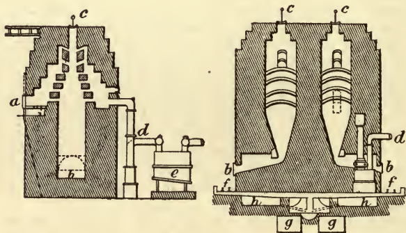
FIG. 162.—KNOX FURNACE.
