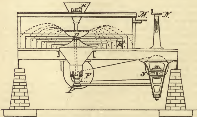
FIG. 78.—CLARKSON-STANFIELD CONCENTRATOR.
