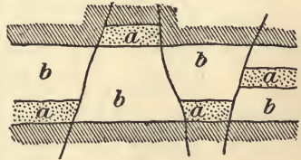
FIG. 169.—SILVER DEPOSITS: SILVER REEF, UTAH.
