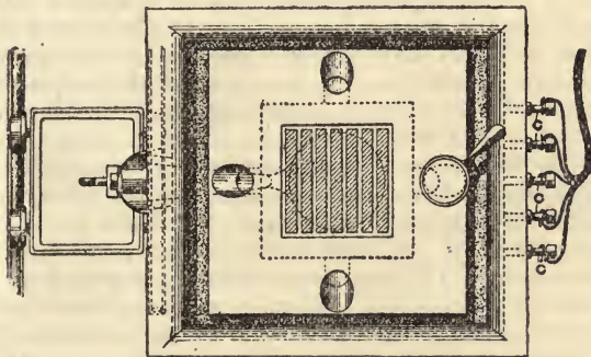
FIGS. 106, 107.—HEROULT ALUMINIUM FURNACE.
