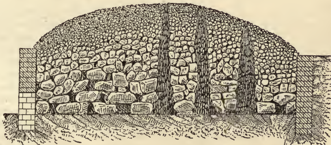
FIG. 100.—ORDINARY CALCARONE.
