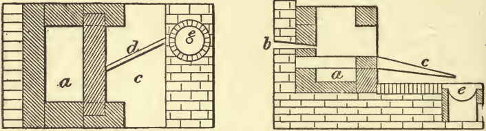
FIG. 153.—SCOTCH ORE HEARTH.
