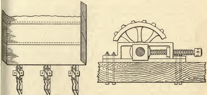
FIGS. 64, 65.—DETAILS OF COAL CONVEYOR.
