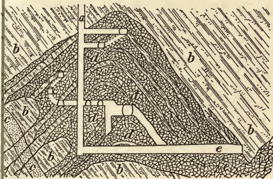
FIG. 132.—GOLD DEPOSITS, MOSQUITO.
