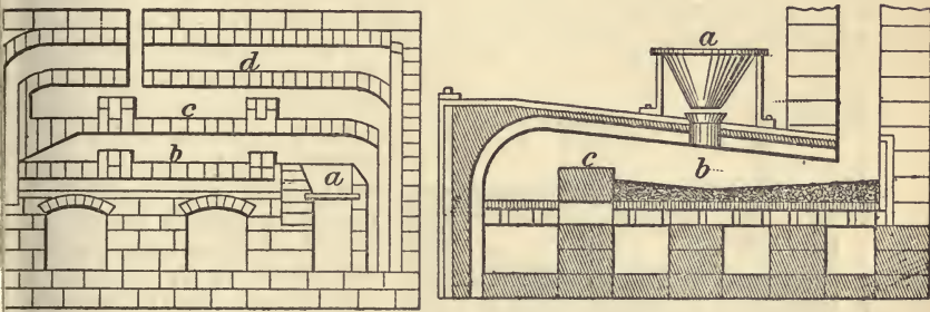
FIGS. 149, 150.—FREIBERG REVERBERATORIES.
