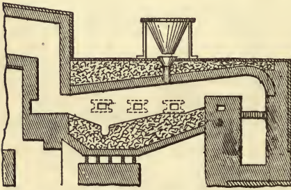
FIG. 151.—FRENCH REVERBERATORY.
