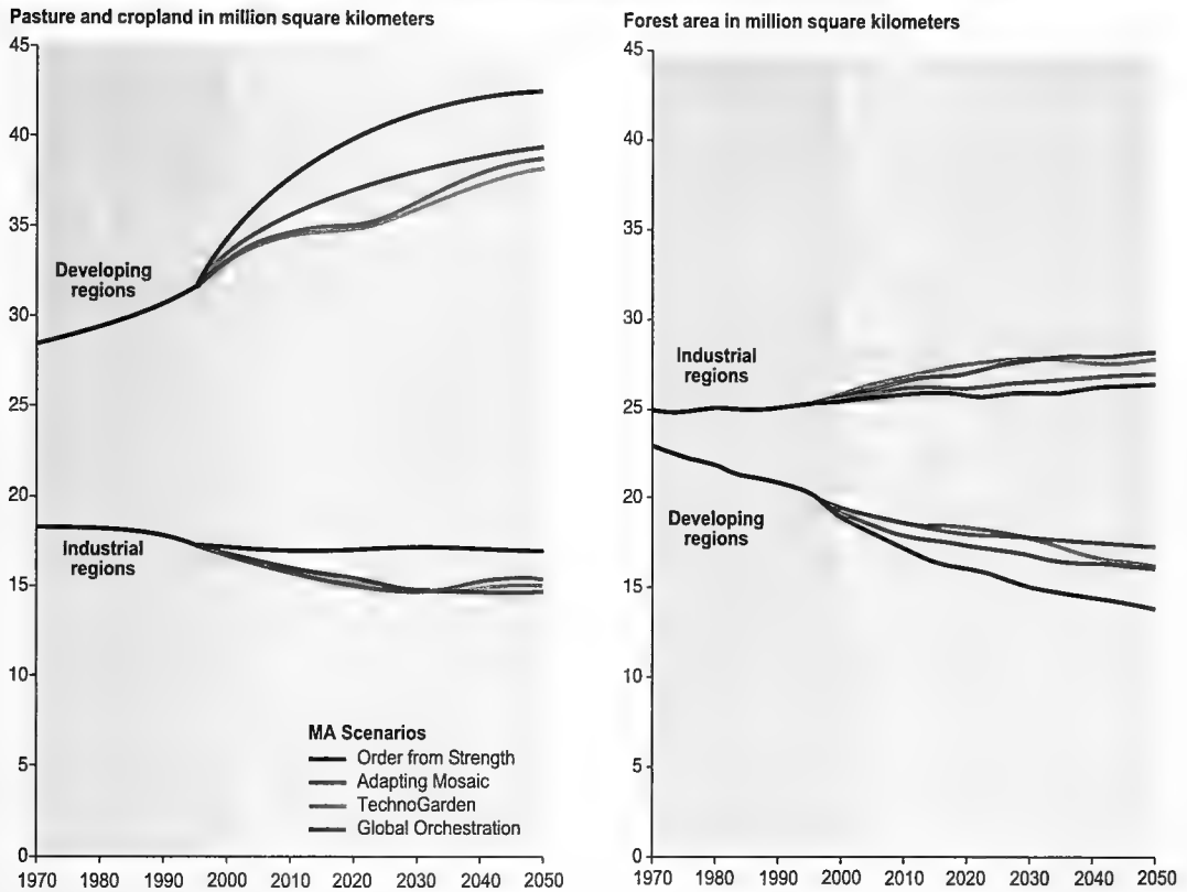
Figure 4.5. FOREST AND CROPLAND/PASTURE IN INDUSTRIAL AND DEVELOPING REGIONS UNDER THE MA SCENARIOS (S9 Fig 9.15)
