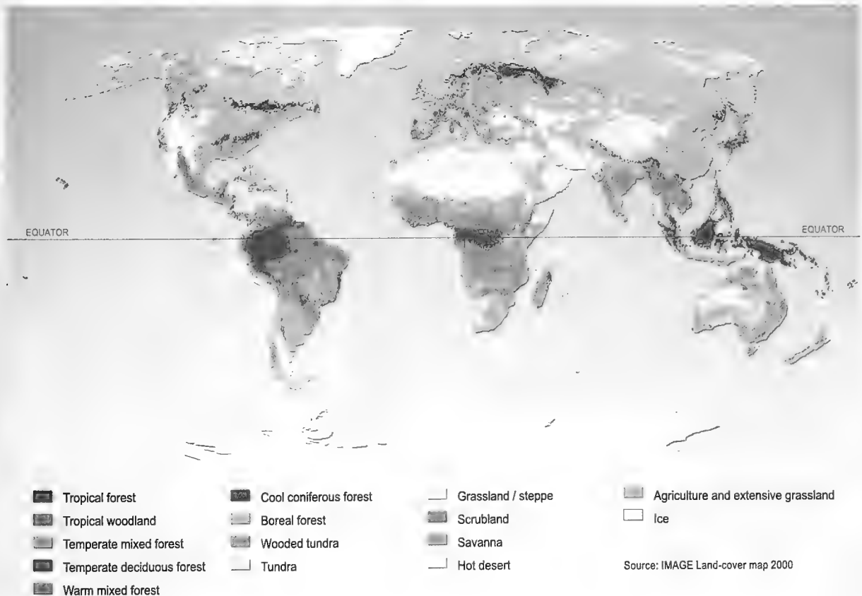
Figure 4.3. IMAGE LAND-COVER MAP FOR THE YEAR 2000 (S6)
