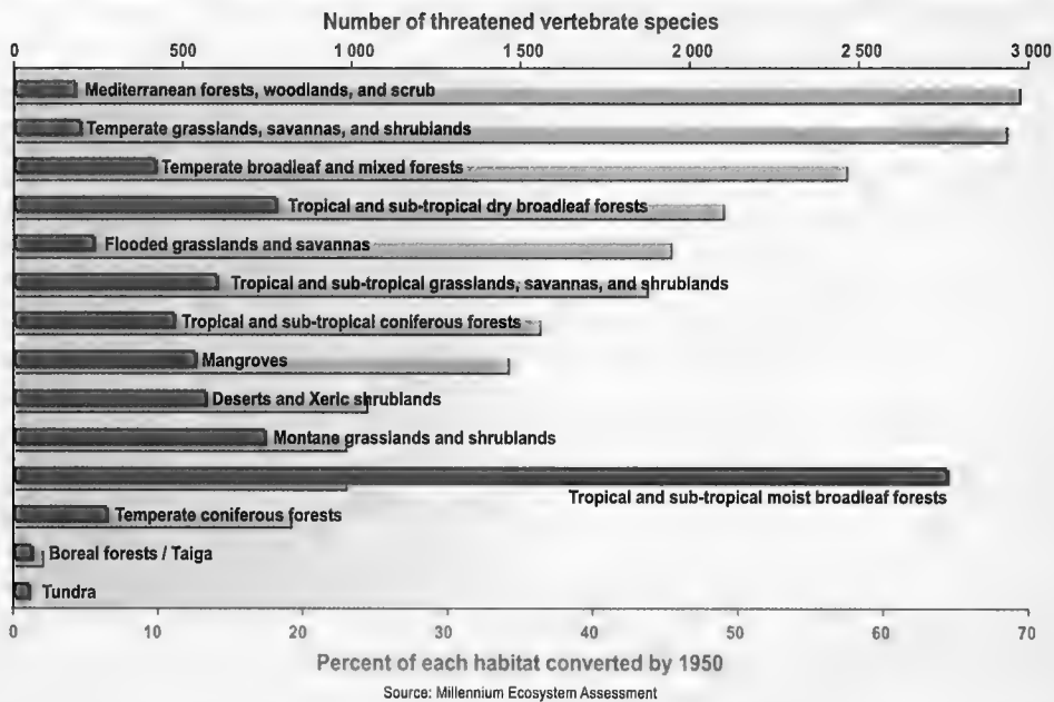
Figure 3.6. THREATENED VERTEBRATES IN THE 14 BIOMES, RANKED BY THE AMOUNT OF THEIR HABITAT CONVERTED BY 1950 (C4)
