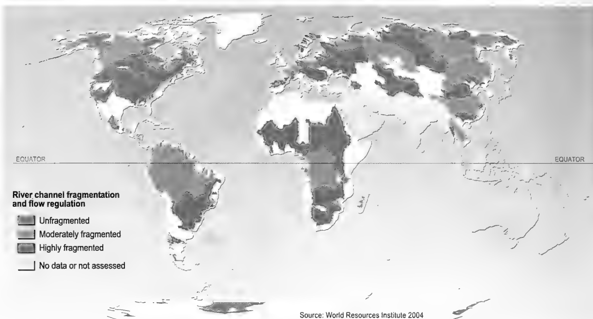
Figure 3.16. FRAGMENTATION AND FLOW IN MAJOR RIVERS (C20)
