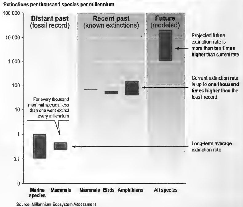
Figure 3.3. SPECIES EXTINCTION RATES (Adapted from C4 Fig 4.22)
