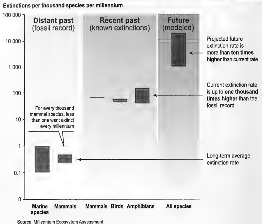
Figure 1. SPECIES EXTINCTION RATES (adapted from C4 Fig 4.22)
