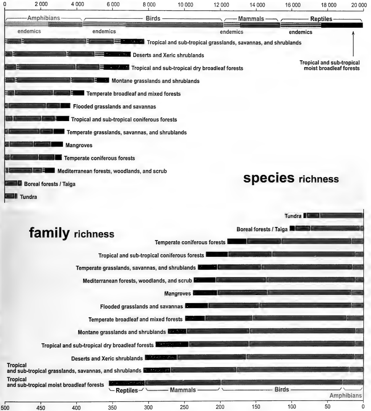
Figure 1.2. COMPARISONS FOR THE 14 TERRESTRIAL BIOMES OF THE WORLD IN TERMS OF SPECIES RICHNESS, FAMILY RICHNESS, AND ENDEMIC SPECIES (C4 Fig 4.7)
