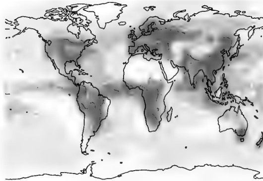
Figure 3.19. ESTIMATED TOTAL REACTIVE NITROGEN DEPOSITION FROM THE ATMOSPHERE (WET AND DRY) IN 1860, EARLY 1990S, AND PROJECTED FOR 2050 (milligrams of nitrogen per square meter per year) (R9 Fig 9.2)
