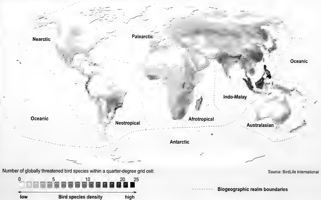
Figure 3.5. DENSITY DISTRIBUTION MAP OF GLOBALLY THREATENED BIRD SPECIES MAPPED AT A RESOLUTION OF QUARTER-DEGREE GRID CELL (C4 Fig 4.25)
