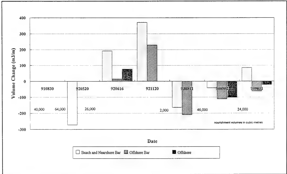
Figure 27. Profiles (beach and offshore) for R22
