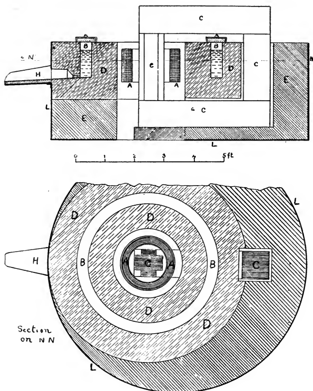
Fig. 24.—The Kjellin Steel Furnace.
