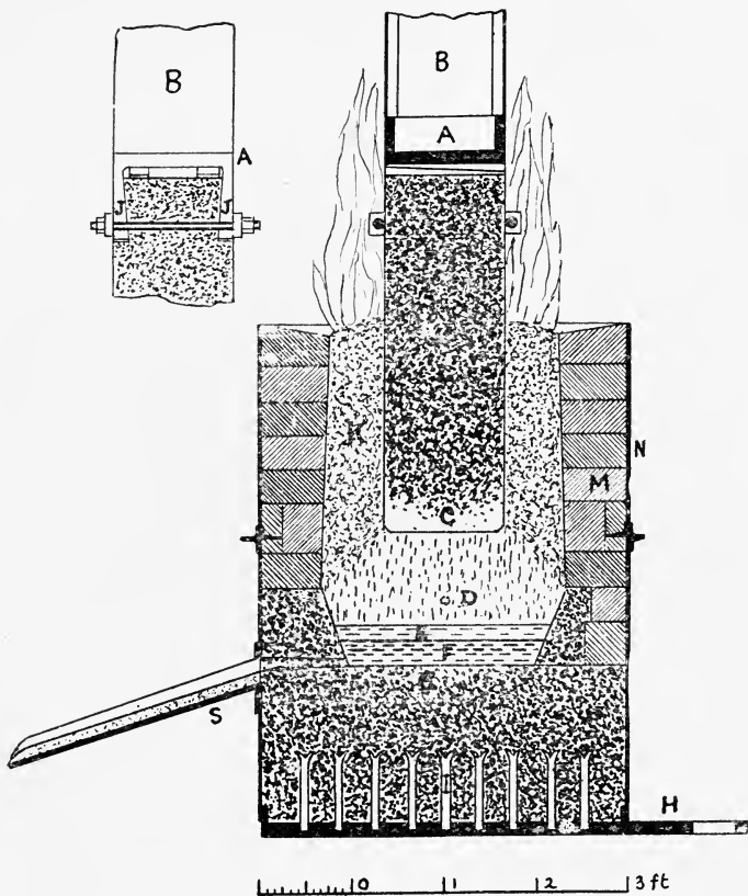
Fig. 29.—Heroult Ore-smelting Furnace.
