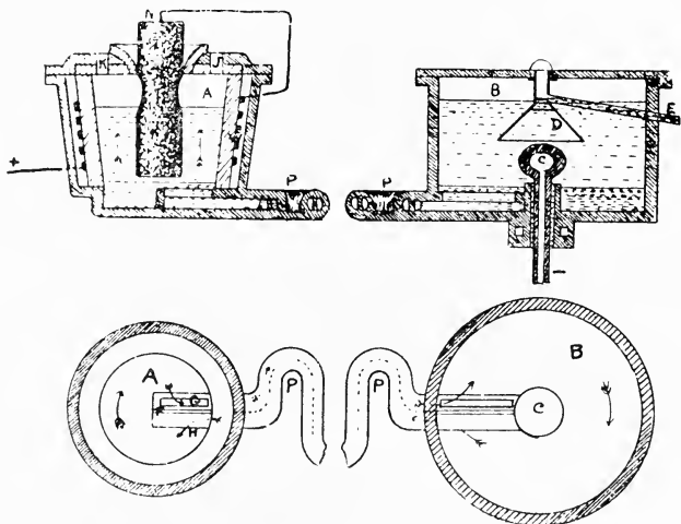
Fig. 51.—Ashcroft's Sodium Furnace.
