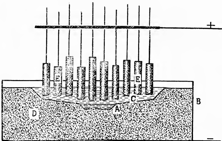
Fig. 52.—Aluminium Furnace.
