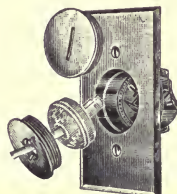
Floor outlet
