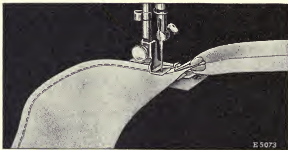
FIG. 160.—The binder
