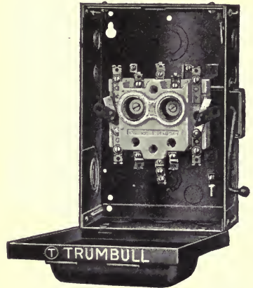
FIG. 94.—Modern service entrance switch
