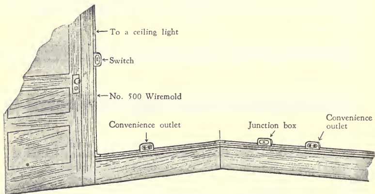
FIG. 89.—Surface metal raceway extension
