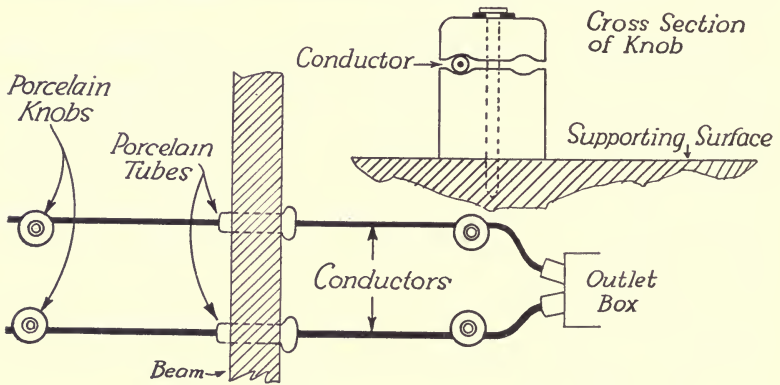
FIG. 277.—Knob-and-tube wiring
