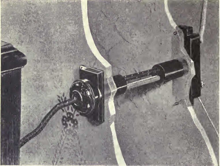
FIG. 173.—Suggested arrangement of radio aerial and ground wires. The lightning arrester is installed on outside wall of house. (Shown at right) (Woodruff)
