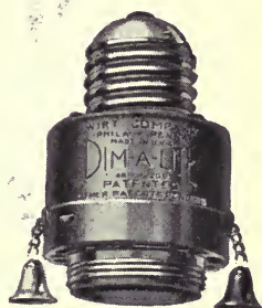
FIG. 68.—“Dim-A-Lite” used for changing intensity of light from an ordinary bulb
