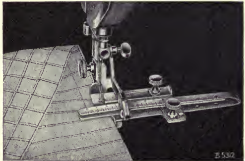
FIG. 163.—The tucker
