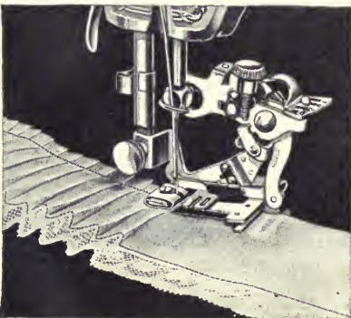
FIG. 165.—The ruffler used for plaiting
