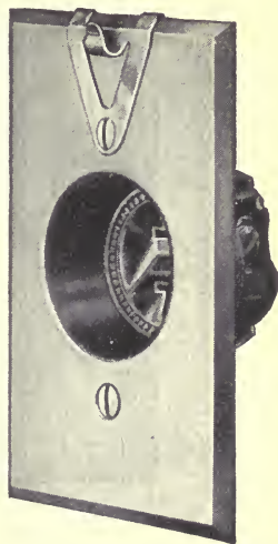
FIG. 17.—A special outlet for a wall clock, provides a hook and requires a short connecting cord. With hook removed it has other uses
