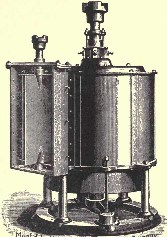
A typical vertical turbine
