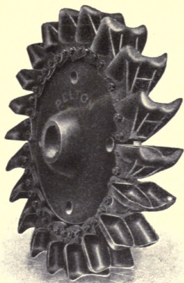
Runner of Pelton wheel, showing peculiar shape of the buckets
