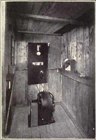
A rough-and-ready farm electric plant, supplying two farms with light, heat and power; and a Ward Leonard-type circuit-breaker for charging storage batteries
