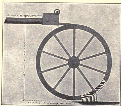
The Fitz overshoot wheel
