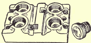
Porcelain cut-out and plug fuse
