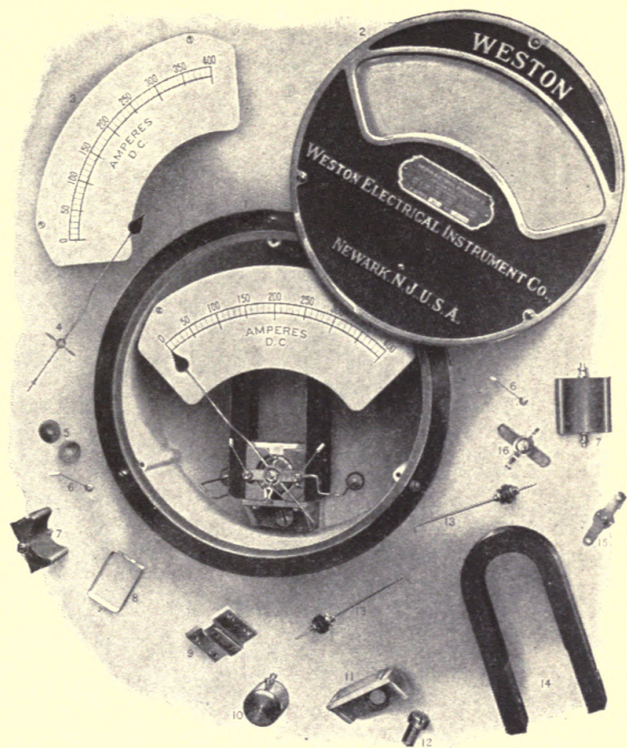
Details of voltmeter or ammeter
