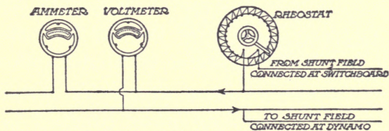
Connecting switchboard instruments
