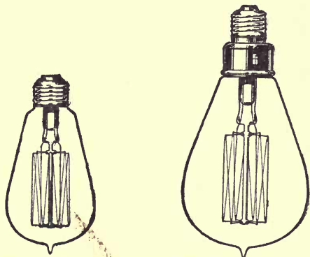
60 and 100 watt Mazda tungsten lamp. These lamps may be had in sizes from 10 to 500 watts ( \frac{1}{4} scale)
