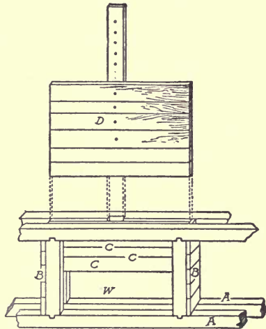
AA - MUD SILLS - SUNK FLUSH WITH BED OF RACE BB - END PLANKING CC - PLANKING HALFWAY DOWN INSIDE OF GATE SLOT D - GATE W - WATER CHANNEL
