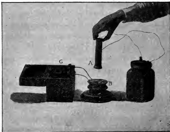
FIG. 85.—MUTUAL INDUCTION.
