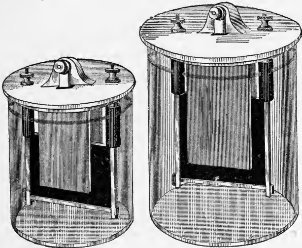
FIG. 13.—EDISON-LALANDE CELLS.
