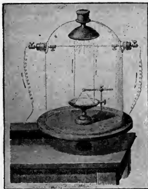
FIG. 3. TRANSMISSION OF HEAT THROUGH A VACUUM.
