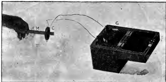
FIG. 87.—MAGNETO-ELECTRIC INDUCTION.
