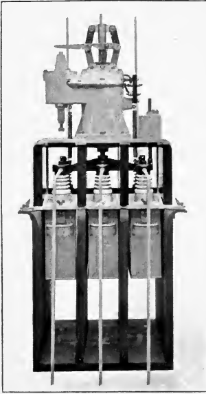
PLATE 14A.—Ferranti 1500 Ohm, 10,000 Volt, Three Phase, Oil Enclosed, Electrically Operated Switch, with Switch closed, but with Case open.
