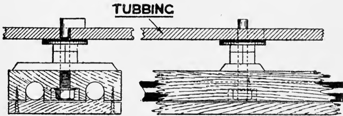
FIG. 96.—Showing Messrs. Callender's Cable Cleat, for two Cables, for bolting to the Brickwork of a Shaft.
