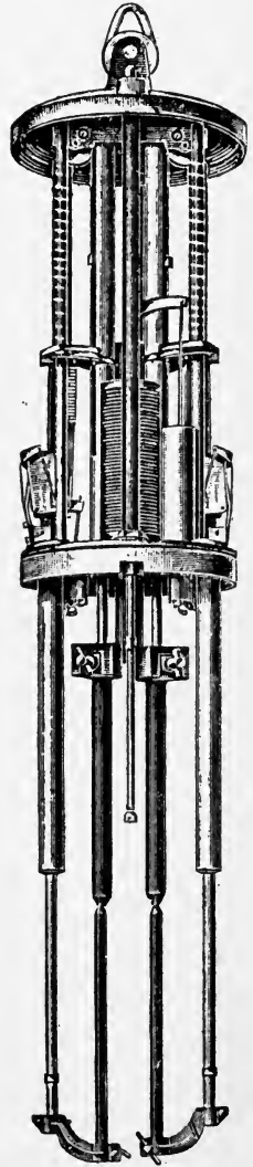
FIG. 29.—"Angold" Open-type Double- carbon Arc Lamp.
