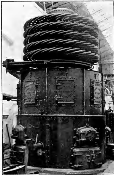
PLATE 1B.—“Climax” Boiler as made by Messrs. B. Rowlands. The Coil at the Top is a Portion of the Boiler Tubes.
