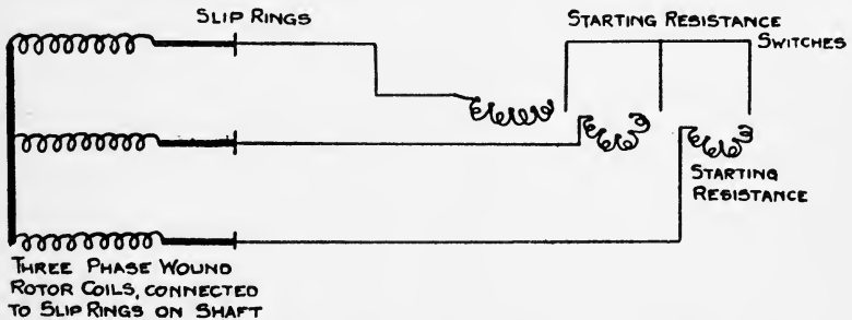
FIG. 124.—Diagram of Connections for starting Three-phase Motors with Wound Rotors.
