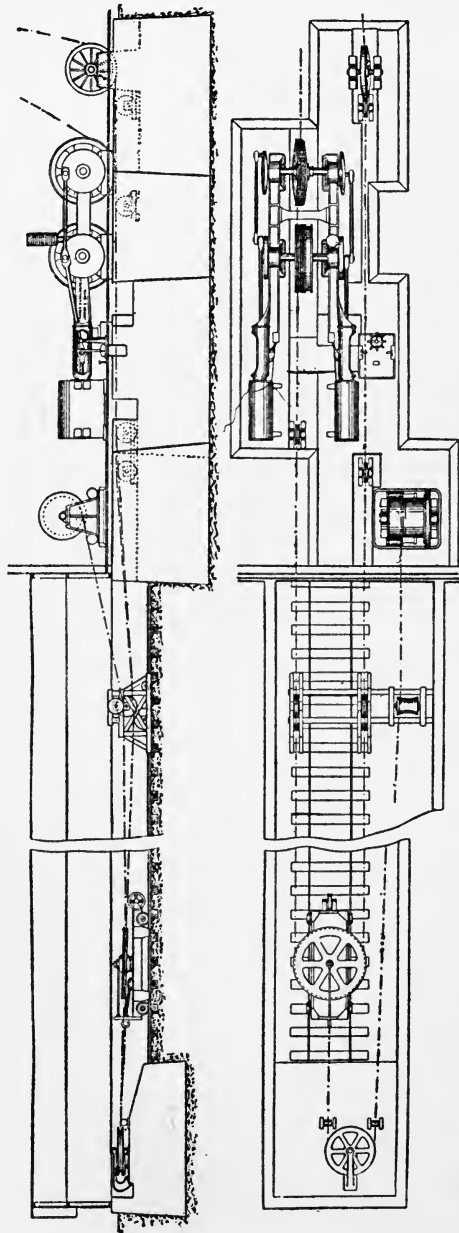
FIG. 145.—Plan showing the Whiting System of Winding from Deep Shafts of Metalliferous Mines, enabling the "Skip" to be stopped at any Level. The Rope is led back round the Pulley shown behind the Engine, and this Pulley is moved forward or backward, according to the Depth of the Level the "Skip" is to stop at.
