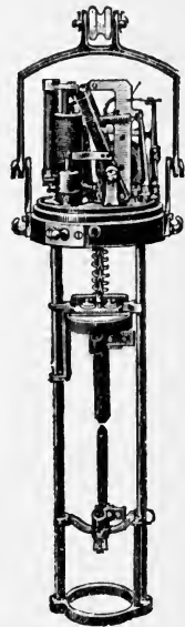
FIG. 23.—Showing the Mechanism of one of the Union Electrical Co.'s Open Arc Lamps.
