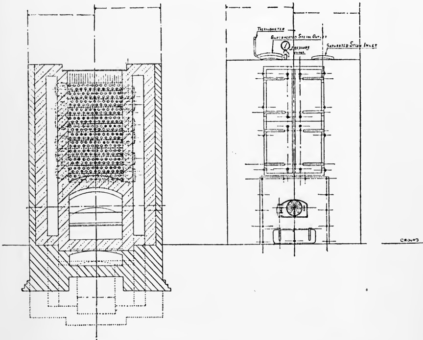
FIG. 68.—Transverse Section and Diagram of the Front of Messrs. Davey, Paxman, & Co.'s Separately Fired Superheater.
