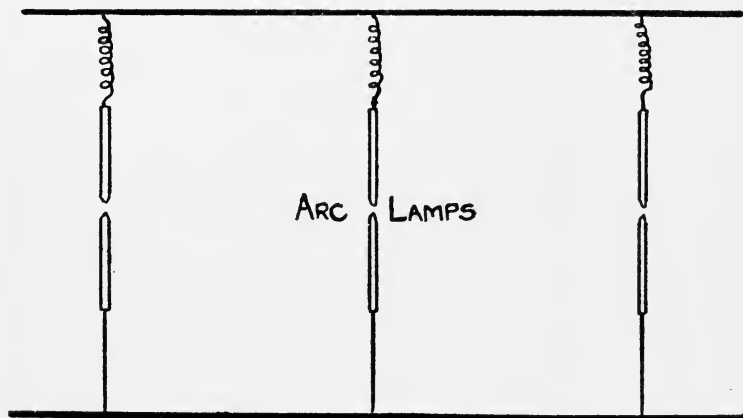
FIG. 36.—Diagram of Connections of Arcs in Parallel across a 65 or 100 Volt Service. Each Arc has its own Resistance as shown. This is the Arrangement that would be employed where Current was taken for the Lighting Service, from the Power Service, through a Motor Generator.
