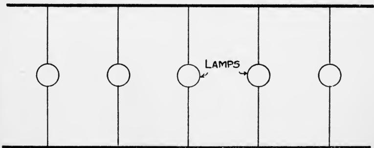
FIG. 2.—Diagram showing Parallel-connections. The Lamps shown are connected in Parallel, the Current passing through all of them together.
