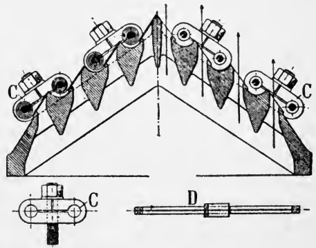
FIG. 134.—Arrangement of Gutermuth Valves on an ordinary Ram Pump. The Number of Small Valves take the Place of a Single Mushroom Valve.
