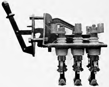
PLATE 17D.—Messrs. Reyrolle's High Tension, Three Phase, Oil Enclosed Switch, with Oil Tank removed, showing Contacts.
