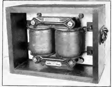
PLATE 17B.—Potential Transformer for Switchboards, shown in Fig. 38.
