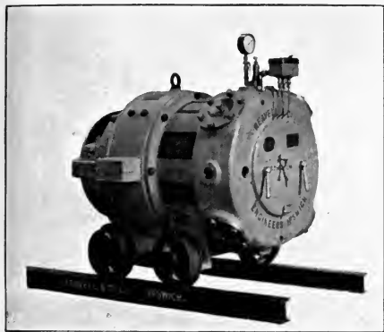
PLATE 31A.—Reavell's Air Compressor with Electric Motor. Portable Form, arranged for placing anywhere in by.
