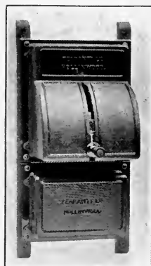
PLATE 18D.—Ferranti Triple Hole Overload, and no Voltage Circuit Breaker, with Cover, not Gas-tight.
