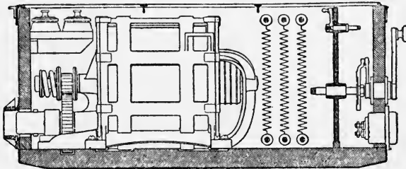
FIG. 152.—Three-phase Motor Case to be used with Siemens' Electric Drills.
