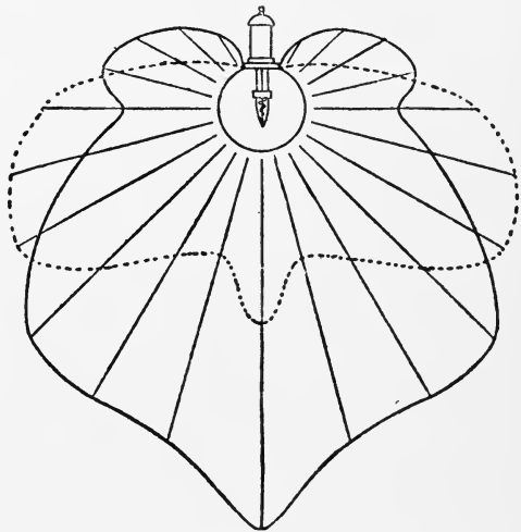
FIG. 52.—Curves showing the Distribution of Light with Nernst Lamp when enclosed in Pointed and Round Holophone Globes. The Full Curve is with the Pointed Globe, and the Dotted Curve with the Round. It will be noticed that the Light is more distributed with the Pointed than the other. The Lengths of the Lines meeting the Curves give the Proportional Intensity of Light at the Different Points.
