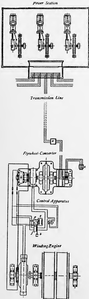
FIG. 141.—Diagram of General Arrangement of Siemens-Igner System of Electric Winding, showing the Power Station, Transmission Line, Flywheel Converter, Winding Motor and Drum, with Control Apparatus.
