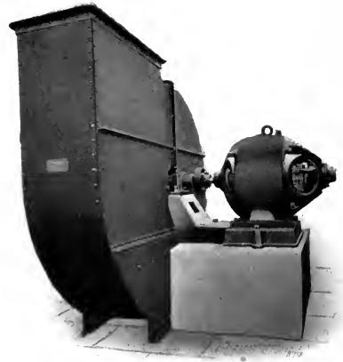
PLATE 30B.—Heenan & Froude's Fan, in Case, with evasé Chimney, driven by an Electric Motor.
