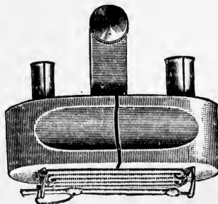
FIG. 47.—Another Form of Heating-coil for Nernst Lamp. It is seen above the "Glower."
