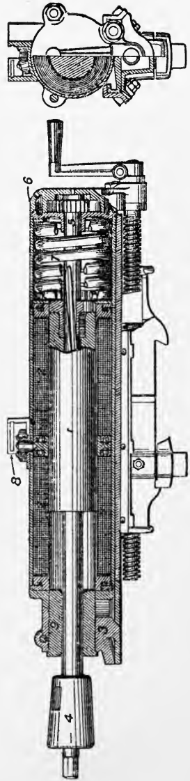
FIG. 155.—Sections of Marvin Sandicroft Electric Drill.
