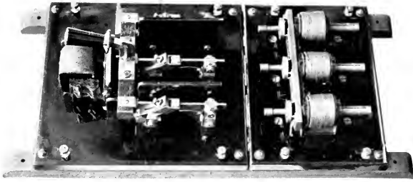
PLATE 13C. — Ferranti Triple-pole Overload, and no Voltage Circuit Breaker. Cover removed.
