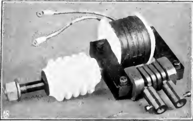
PLATE 17A.—Current Transformer for use with High Tension Switchboards, as made by Messrs. Elliott Bros.
