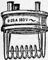
FIG. 46.—"Glower" and Heating-coil of Nernst Lamp, with the Porcelain Supporting Disc. The "Glower" is the Straight Portion inside the Coil.
