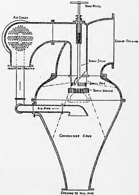
FIG. 75.—Section of Worthington Central Condenser.
