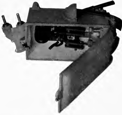
PLATE 15C.—Messrs. Dorman & Smith's Gas Proof and Fool Proof Mining Switch. The Case cannot be opened if the Switch is closed. The connections are led through the Glands shown.
