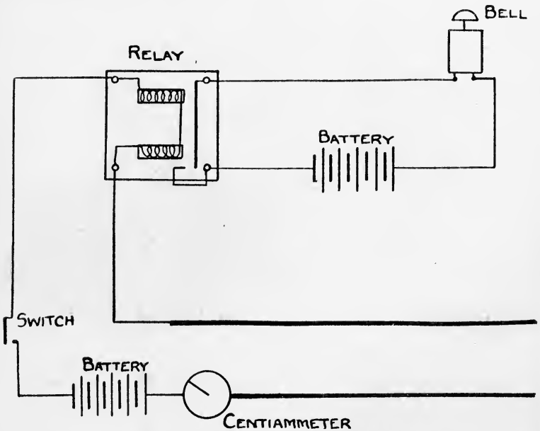
FIG. 18.—Diagram of the Connections of a Two-wire Engine-road Signal, with Relay, two Batteries, Switch, and Centiammeter.
