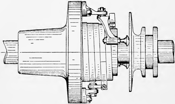
FIG. 136.—Coil Clutch.
