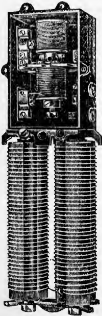
FIG. 37. — Automatic Cutout for Continuous Current Arc Lamp, with the Resistance that is to take the Place of the Arc, as made by the General Electric Co., London.
