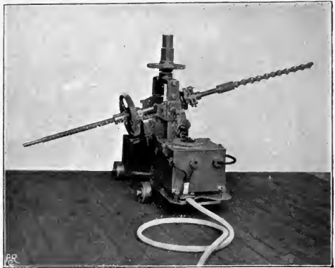
PLATE 22D.—Diamond Electric Rotary Drill.
