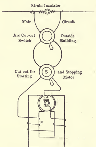
FIG. 69. — CONNECTIONS OF CONSTANT-CURRENT SERIES MOTOR.
