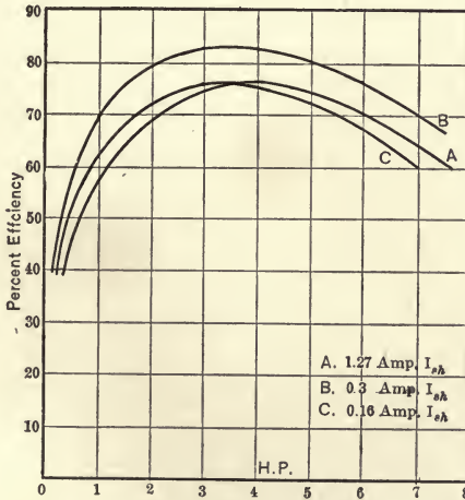
FIG. 26.—EFFICIENCY CURVES OF A 6-H.P. ADJUSTABLE-SPEED "INTERPOLE" MOTOR.
