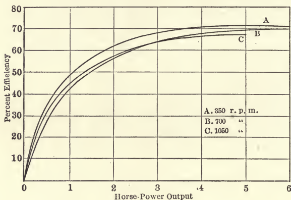
FIG. 10. — EFFICIENCY CURVES OF 5-H.P. BULLOCK MOTOR AT SPEEDS OF 350, 700 AND 1050 R.P.M.
