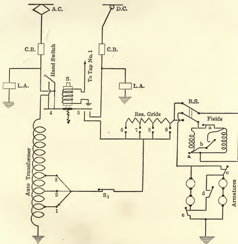
FIG. 151. — CONNECTIONS FOR OPERATING SERIES MOTOR ON MIXED SERVICE.
