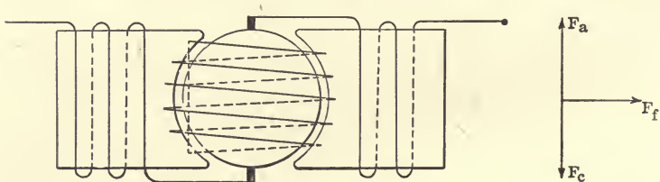
FIG. 150. — SERIES MOTOR WITH COMPENSATING TRANSFORMER (INDUCTIVE COMPENSATION).
