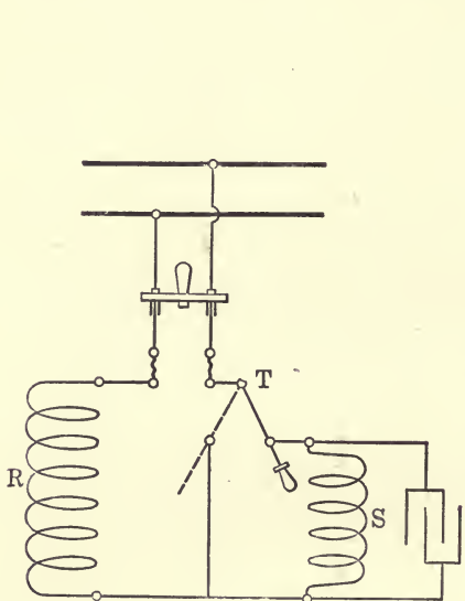
FIG. 136.—CONNECTIONS FOR STARTING SMALL SINGLE-PHASE INDUCTION MOTORS.
