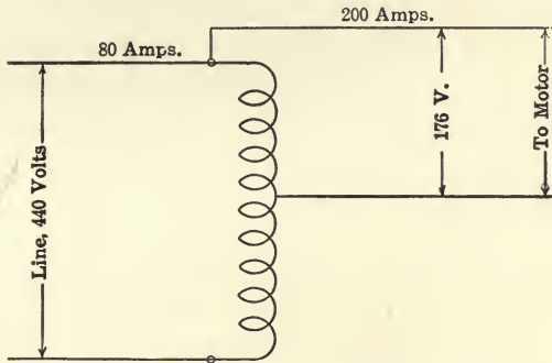
FIG. 114. — SIMPLE AUTO-TRANSFORMER CONNECTIONS.
