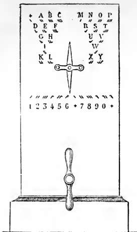
Fig. 66.—THE SINGLE NEEDLE TELEGRAPH.
