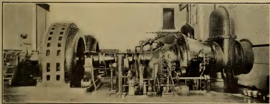
FIG. 183.—GREAT NORTHERN RAILWAY—CASCADE TUNNEL POWER PLANT EQUIPMENT.
