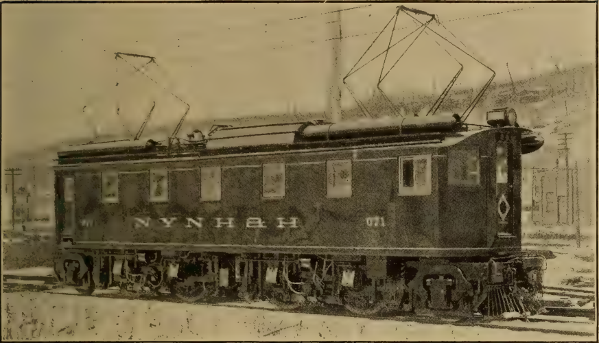
FIG. 139.—NEW YORK, NEW HAVEN AND HARTFORD GEARED FREIGHT LOCOMOTIVE, 1909. [
