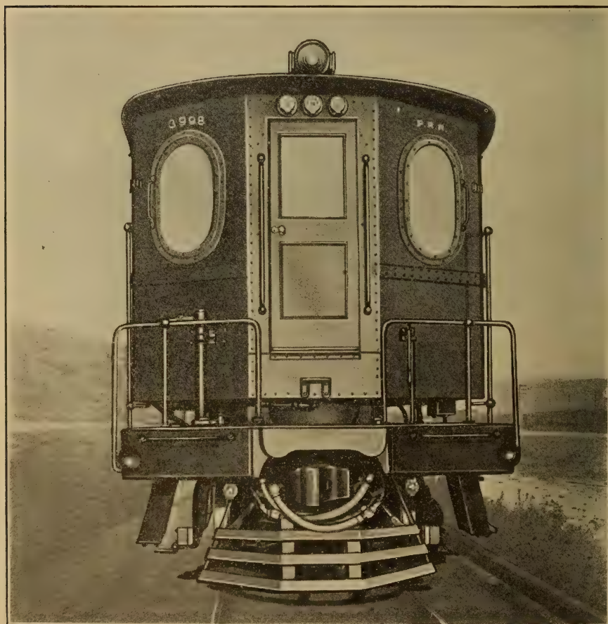
FIG. 104.—PENNSYLVANIA RAILROAD. FRONT ELEVATION OF LOCOMOTIVE.
