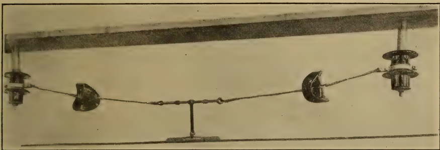
FIG. 175.—GREAT NORTHERN RAILWAY. INSULATOR SUPPORT IN CONCRETE ROOF OF TUNNEL, PARALLEL TO THE CONTACT LINE.
