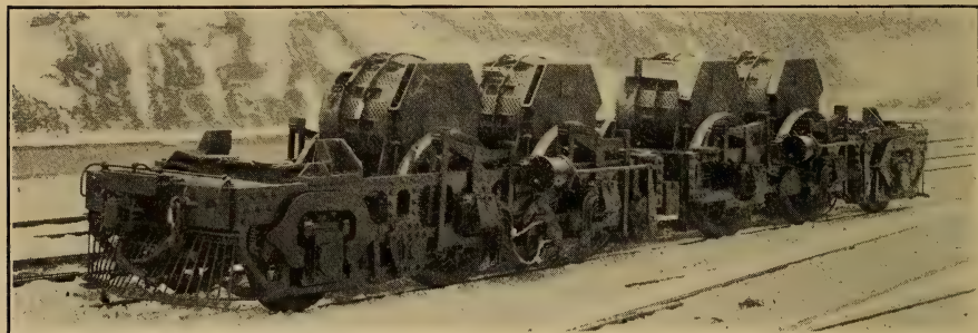
FIG. 142.—NEW YORK, NEW HAVEN AND HARTFORD GEARED FREIGHT LOCOMOTIVE, 1909. Motors and truck for locomotive number 071.
