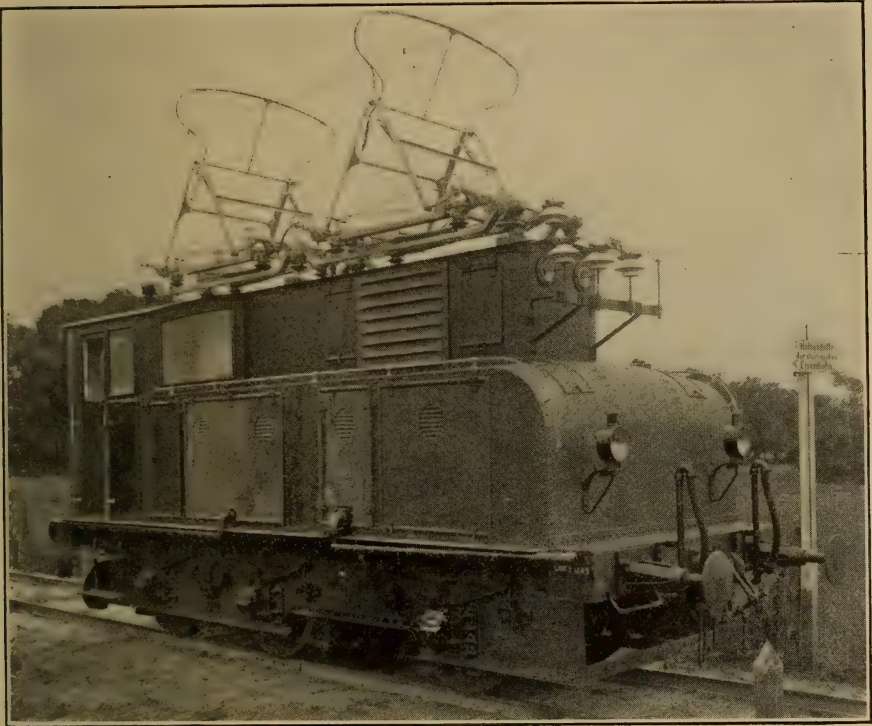
FIG. 149.—SWEDISH STATE RAILWAY. SIEMENS SINGLE-PHASE LOCOMOTIVE OF 1906.
