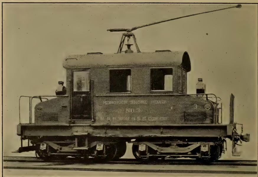
FIG. 90.—HOBOKEN SHORE FREIGHT SWITCHING LOCOMOTIVE. 64-ton, 400-h. p., Westinghouse unit used since 1906.
