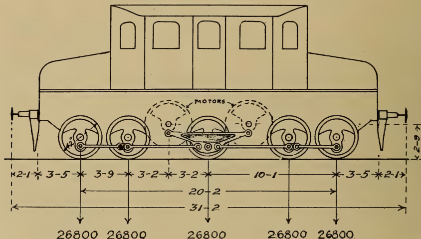
FIG. 119.—ITALIAN STATE RAILWAY LOCOMOTIVE. GIOVÌ LINE, 1903.
