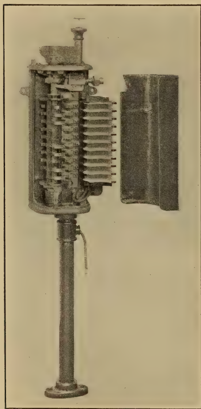
FIG. 66.—GENERAL ELECTRIC TRAIN CONTROLLER.
