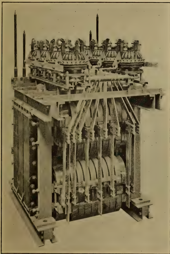
FIG. 164.—BERNESE ALPS RAILROAD. TRANSFORMER ON OERLIKON LOCOMOTIVE.
