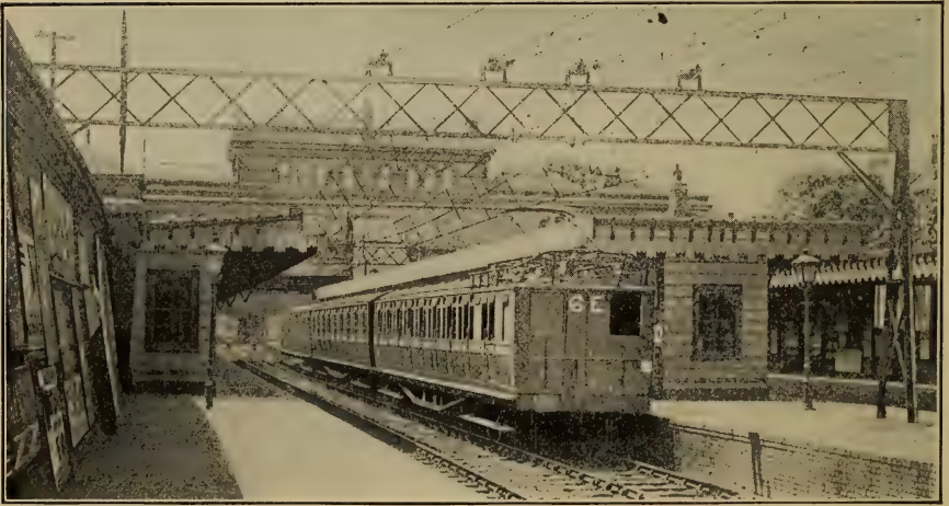
FIG. 65.—LONDON, BRIGHTON AND SOUTH COAST RAILWAY MOTOR-CAR TRAIN. The 6600-volt, 25-cycle, single-phase system. Four 115-h. p. motors per motor car; two 55-ton motor cars and one 35-ton coach per three-car train. Four 175-h. p. motors per motor car; two 60-ton motor cars and two 35-ton coaches per four-car train.
