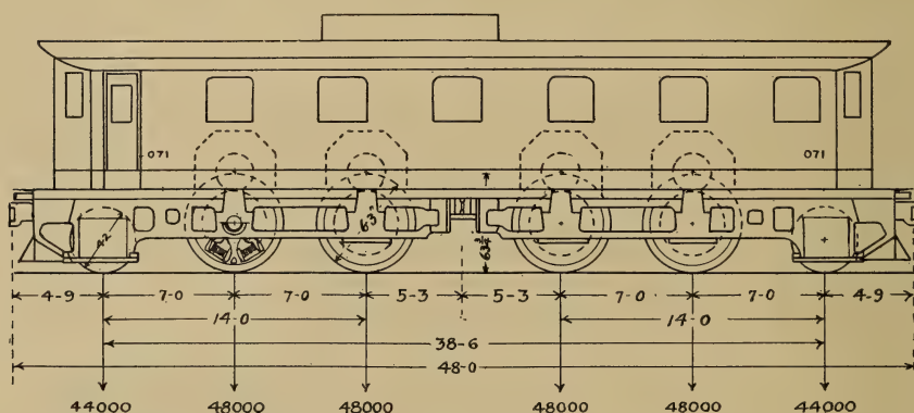
FIG. 141.—NEW YORK, NEW HAVEN AND HARTFORD GEARED FREIGHT LOCOMOTIVE, 1909. One used on New York Division. 140-ton, 1260-h. p., 1-phase, 25-cycle, 11,000-300-volts. Four geared motors. Gear ratio 2.32. Forced ventilation. Freight service.
