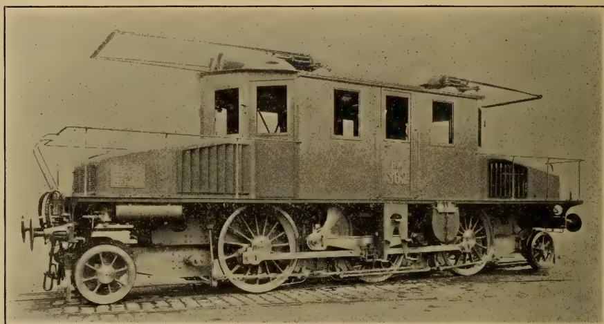
FIG. 116.—ITALIAN STATE RAILWAY,—VALTELLINA LOCOMOTIVE OF 1906.
