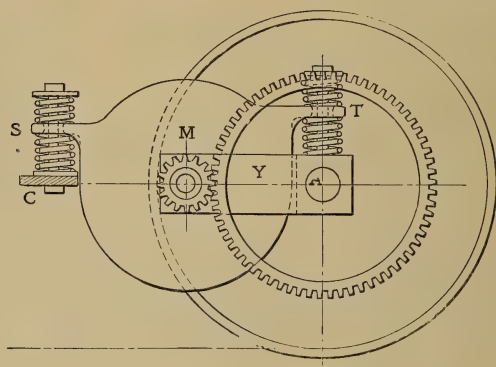
FIG. 46.—DIAGRAM OF WALKER METHOD OF MOTOR SUSPENSION.
