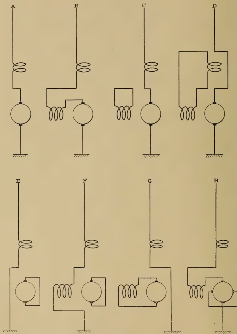
FIG. 32.—SIMPLEST TYPE OF SINGLE-PHASE RAILWAY MOTORS.
