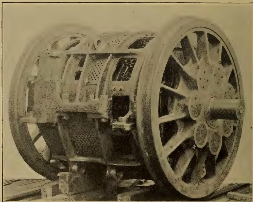
FIG. 44.—NEW YORK, NEW HAVEN AND HARTFORD RAILROAD PASSENGER LOCOMOTIVE MOTORS, 1906. Motor is quill mounted on axle and spring mounted in drivers.
