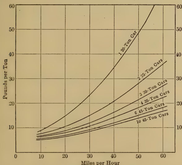
FIG. 167.—TRACTIVE RESISTANCE CURVES. One to ten electric motor-car passenger trains.
