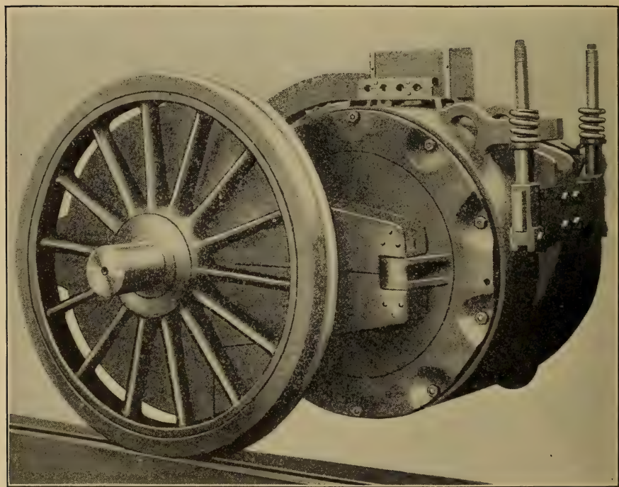
FIG. 38.—GRAND TRUNK RAILWAY LOCOMOTIVE MOTOR.
