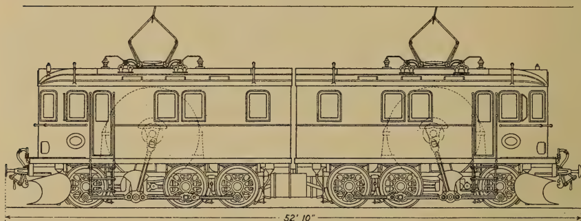
FIG. 151.—SWEDISH STATE RAILWAY. CRANK AND SIDE ROD FREIGHT LOCOMOTIVE. 18,000-volt, 15-cycle, single-phase, 2000-h. p. unit.
