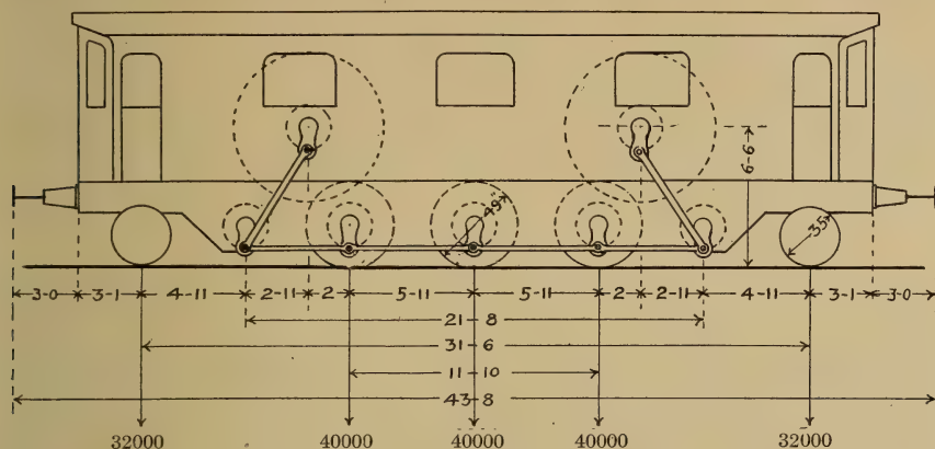
FIG. 153.—FRENCH SOUTHERN RAILWAY LOCOMOTIVE, 1910.
