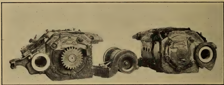
FIG. 42.—PENNSYLVANIA RAILROAD MOTOR EQUIPMENT AND FORCED DRAFT FAN. Used on motor-car trucks in New York-Long Island service. Axle centers 8 1/2 feet. Entire axle enclosed. Motors, direct-current, 215-h. p. each.
