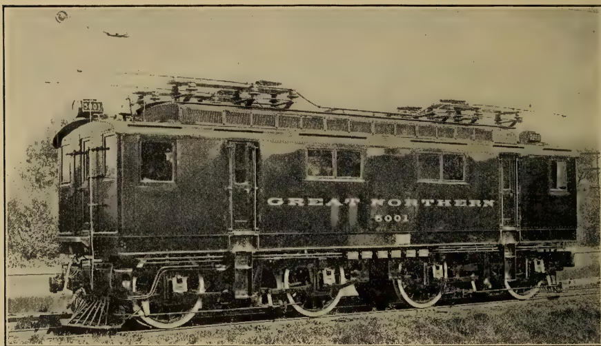
FIG. 124.—GREAT NORTHERN RAILWAY LOCOMOTIVE, 1909.
