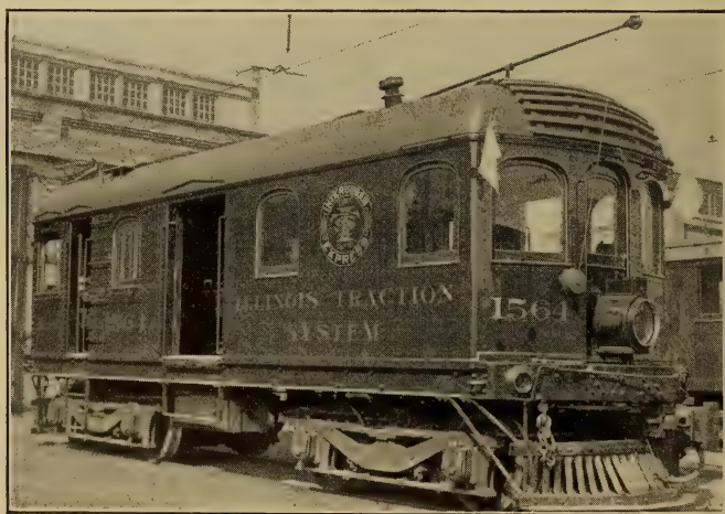
FIG. 110.—ILLINOIS TRACTION COMPANY LOCOMOTIVE OF 1910.
