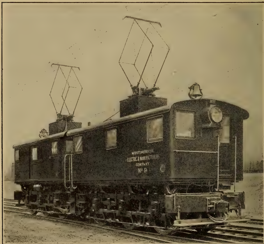
FIG. 126.—FIRST SINGLE-PHASE LOCOMOTIVE IN AMERICA, 1905.
