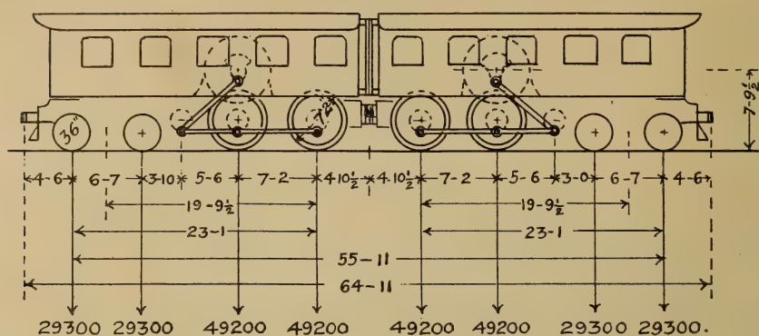
FIG. 103.—PENNSYLVANIA RAILROAD LOCOMOTIVE OF 1910.
