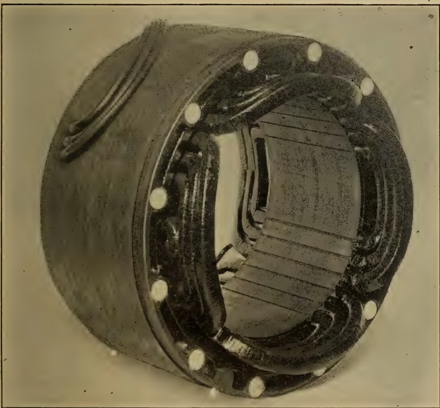
FIG. 39.—WINTER-EICHBERG SINGLE-PHASE RAILWAY MOTOR. Showing main magnetizing coils and commutating coils in stator.
