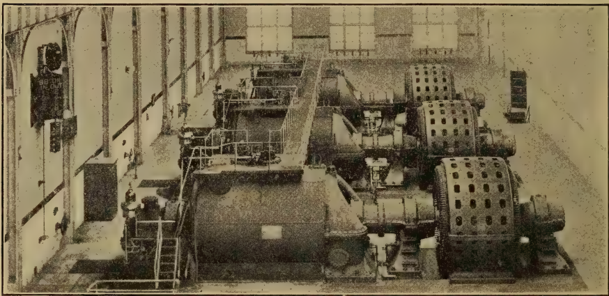
FIG. 180.—PENNSYLVANIA-LONG ISLAND RAILROAD POWER PLANT. Three 5,500-kilowatt Westinghouse turbines and 25-cycle, 3-phase, 11,000-volt alternators.
