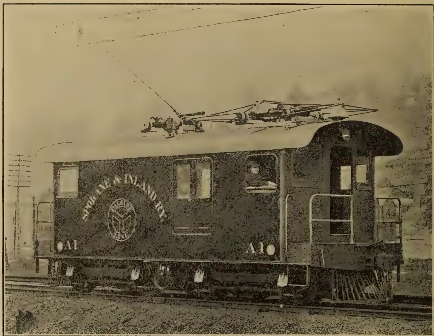
FIG. 130.—SPOKANE AND INLAND EMPIRE RAILROAD Locomotive, 1906.
