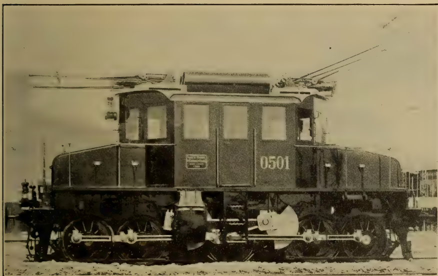
FIG. 118.—ITALIAN STATE RAILWAY LOCOMOTIVE. GIOVI LINE, 1909.
