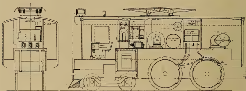
FIG. 128.—PENNSYLVANIA RAILROAD. EXPERIMENTAL LOCOMOTIVE, 1909.
