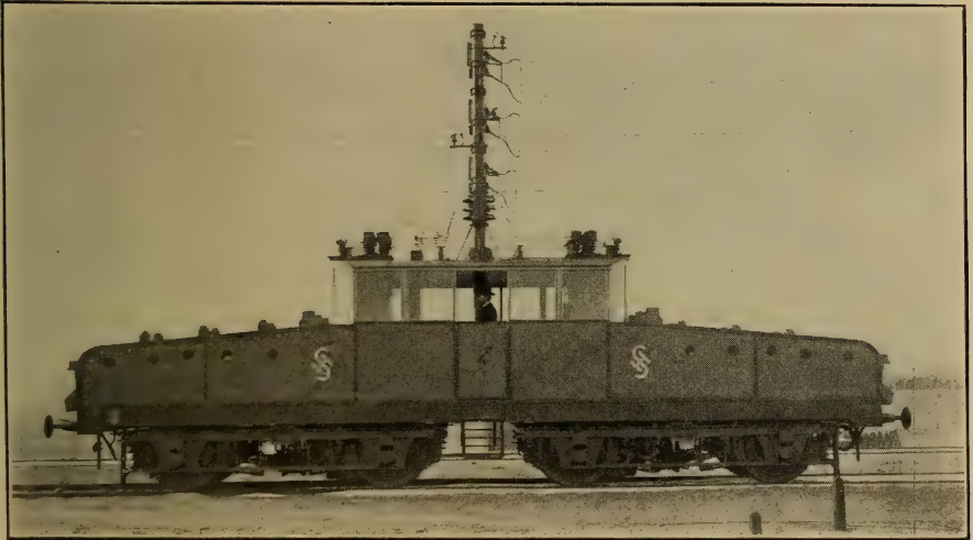
FIG. 115.—SIEMENS-SCHUCKERT LOCOMOTIVE OF 1904. Three-phase, 11,000- to 1000-volt, 1000-h. p., geared type.
