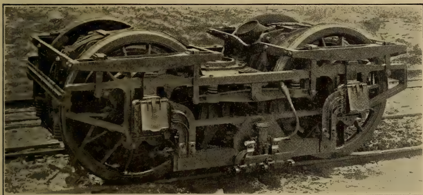
FIG. 134.—NEW YORK, NEW HAVEN AND HARTFORD. PASSENGER MOTOR TRUCK AND GEARLESS MOTOR.
