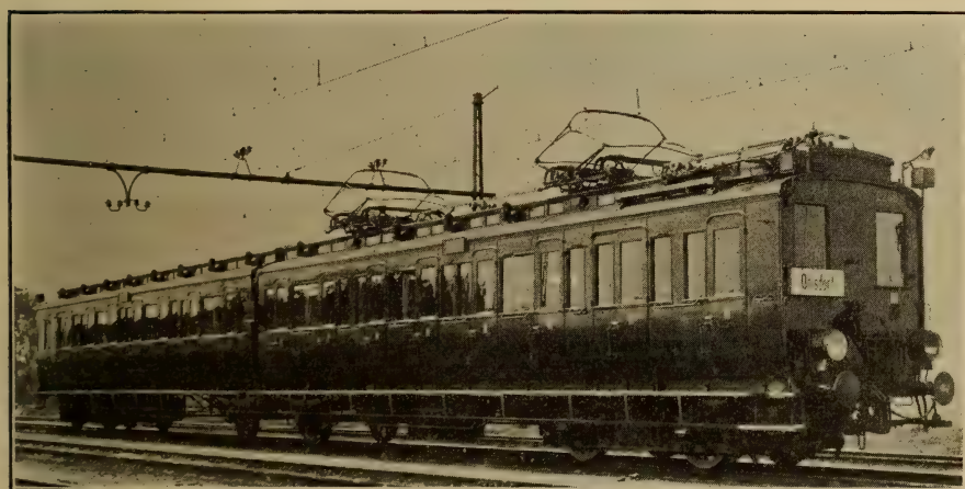
FIG. 80.—BLANKENESE-HAMBURG-OHLSDORF MOTOR-CAR TRAIN. Two 69-ton motor cars each with two 200-h. p., single-phase motors.
