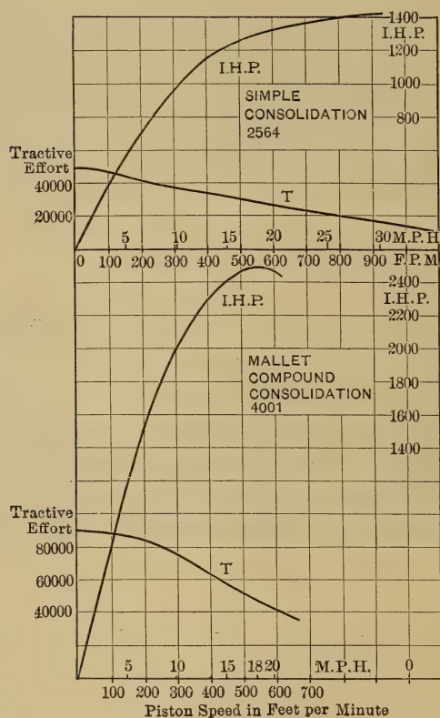
FIG. 26.—OPERATING CHARACTERISTICS OF SIMPLE AND MALLETT COMPOUND LOCOMOTIVES. SOUTHERN PACIFIC CO.
