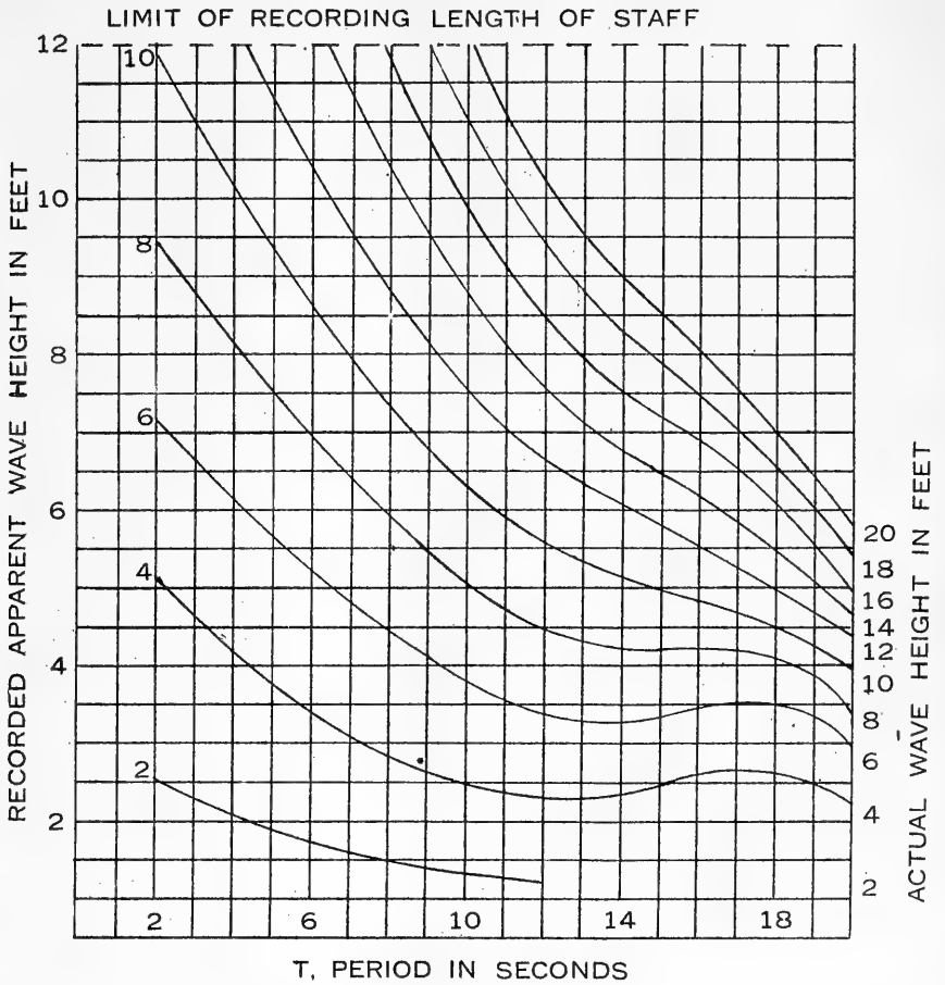
CALIBRATION CURVE - 50-FOOT DAMPING DISK SYSTEM
