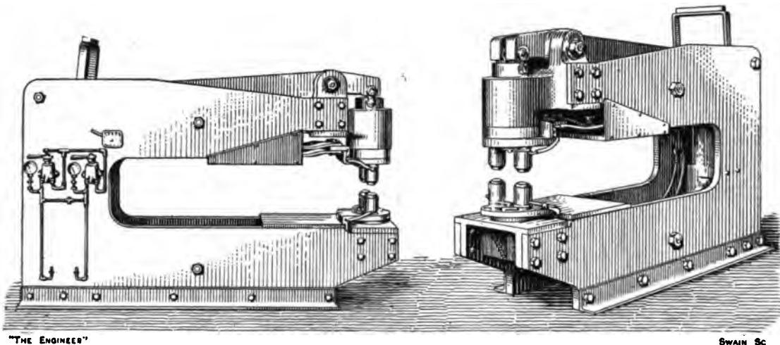
FIG. 60.—Large American Duplex Spot Welder.
