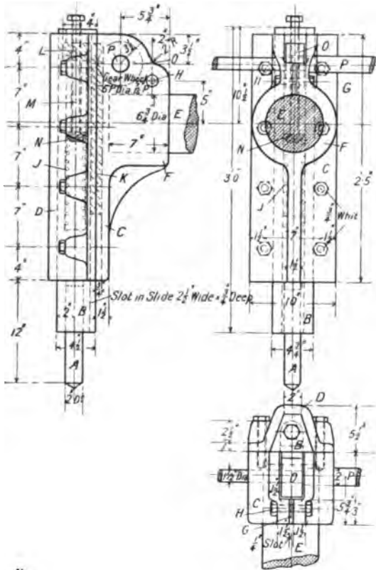
FIG. 71.—Arrangement of Electrode Slide.
