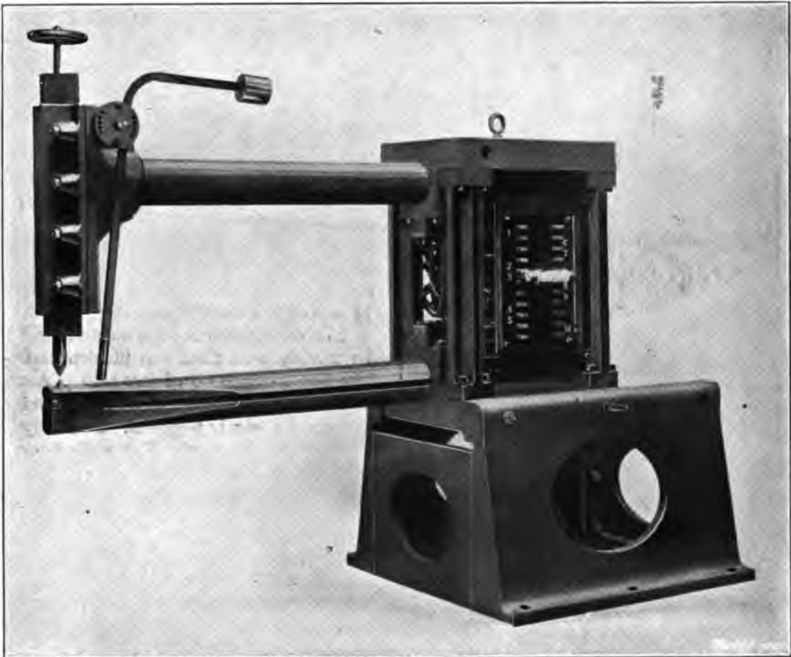
FIG. 68.—Pontelec Spot Welder, with Stakes arranged horizontally.
