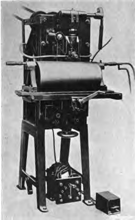
FIG. 22.—Typical Pontelec Seam Welder.
