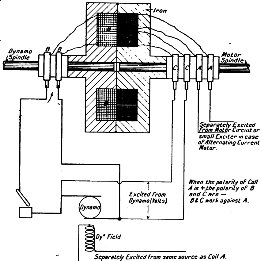
FIG. 43.—Diagram of Connections of Davies-Soames Clutch.
