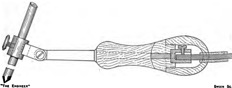
FIG. 3.—The Benardos Electrode Holder.
