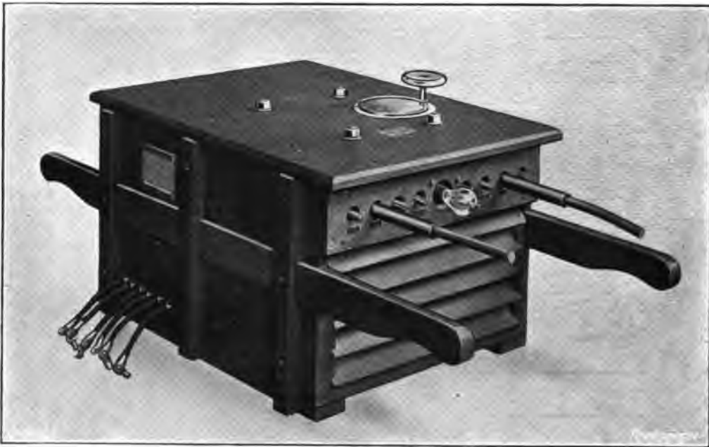
FIG. 81.—The A.C. Electric Welding and Cutting Machine.
