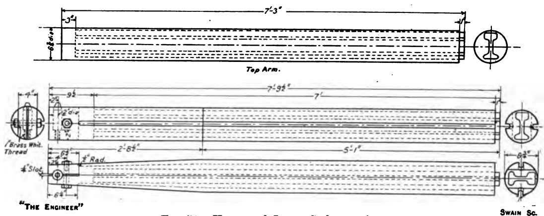
FIG. 70.—Upper and Lower Stakes or Arms.
