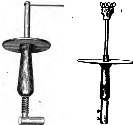
FIG. 53.—E. and E. Company Electrode Holders.
