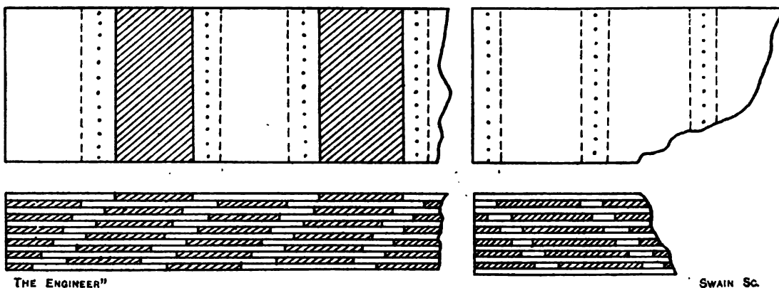
FIG. 7.—Suggested formation of Armour Plate.
