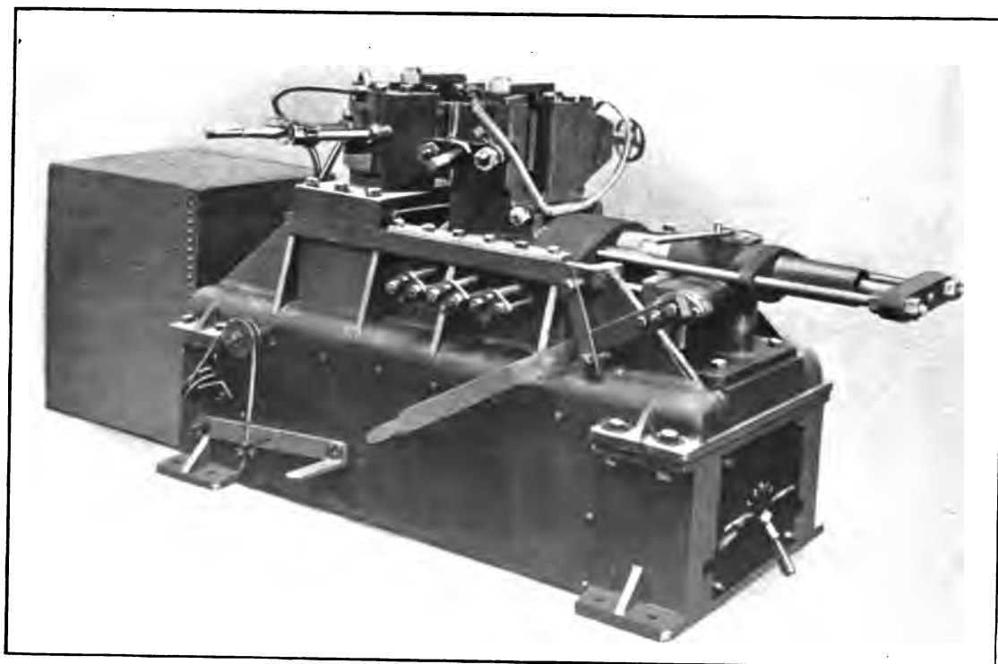
FIG. 55.—Electric Welding Co.—Butt Welder with Radial Welding Blocks.
