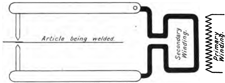
FIG. 9.—Diagram showing Principle of Spot Welding.
