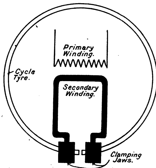
FIG. 11.—Diagram showing Butt Welding of Tyres.
