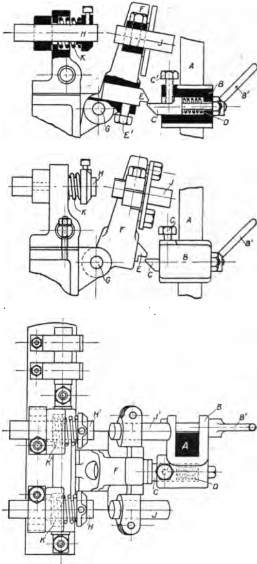
FIG. 63.—"A 1" Automatic Switch.
