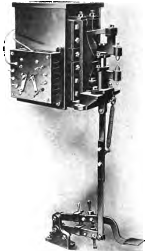
FIG. 20.—Spot Welder for Bench Work.
