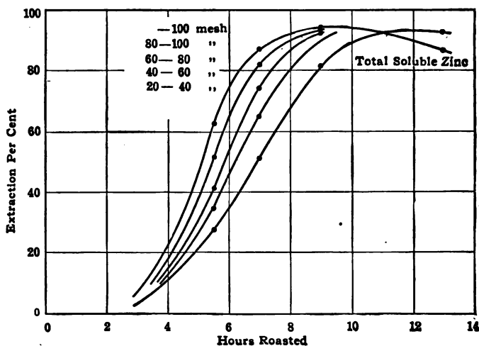
FIG. 3.—Daly-Judge concentrates roasted isothermally at 650° C. Effect of screen size
