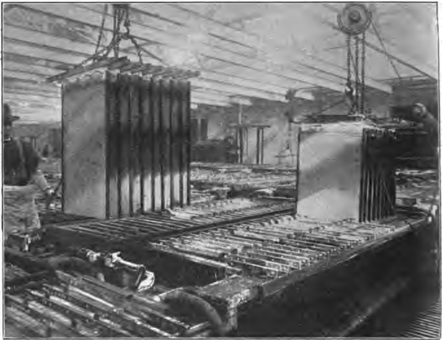
FIG. 20.—Gang-lifting of cathodes (Great Falls)
