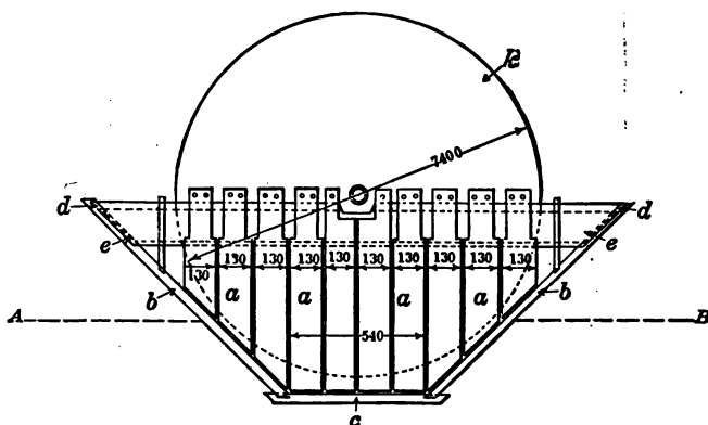
FIG. 23.—Elevation of one anode frame and anodes
