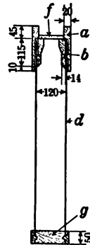
Section at CD
