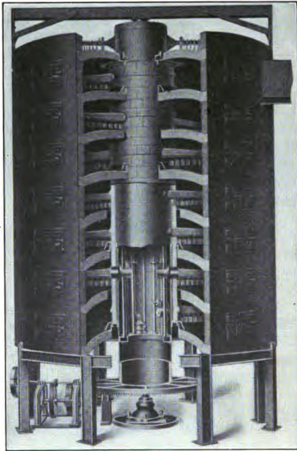
FIG. 1.—The Wedge zinc roaster
