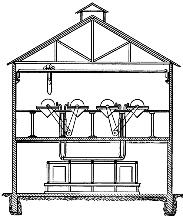
FIG. 36.—Hoepfner's plant at Fűrfurt (cross-section)
