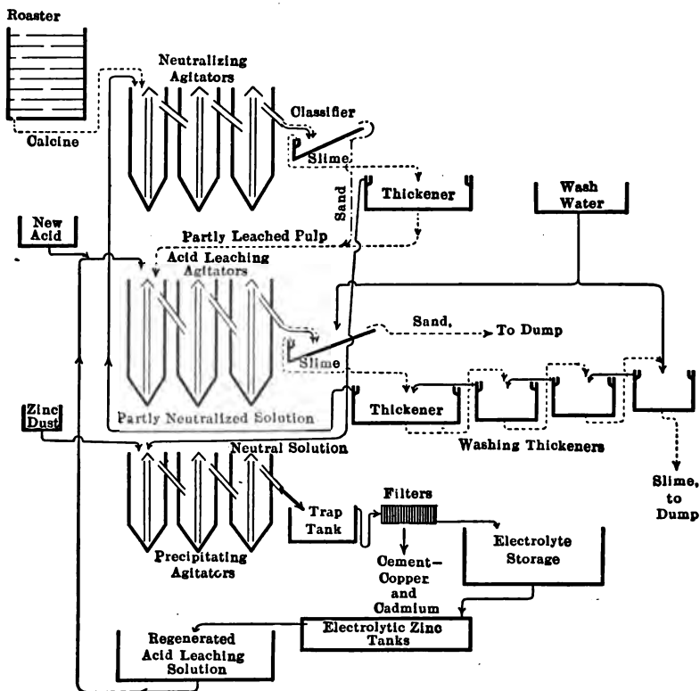
FIG. 8.—Idealized flow sheet of Electrolytic Zinc Plant at Trail, British Columbia
