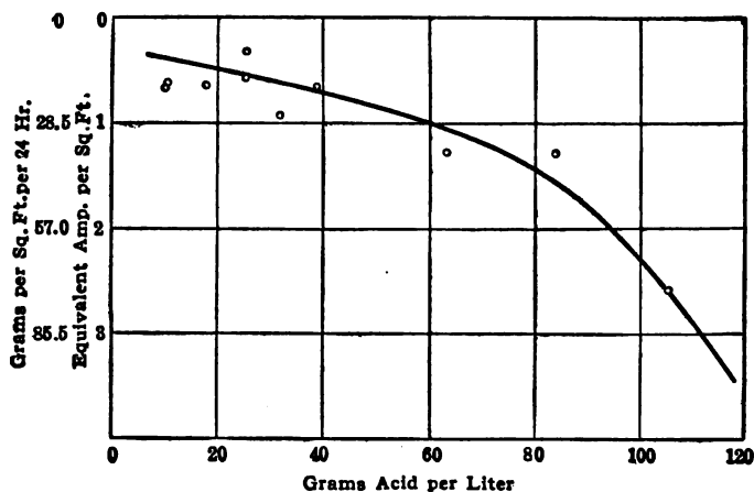
FIG. 9.—Corrosion of smooth cathodes, suspended in active cells, but insulated from bus bars. Bully Hill, March, 1915. (C. A. Hansen)
