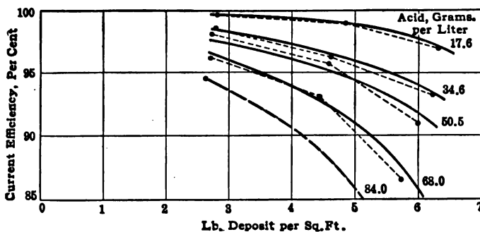
FIG. 11.—Bully Hill ores, June, 1915. (Hansen.) Current density, 15 amp. per sq. ft.
