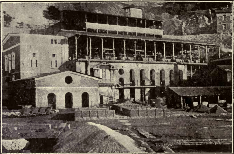
FIG. 69A.—CALAMINE DRESSING PLANT, MONTEPONI, SARDINIA.
