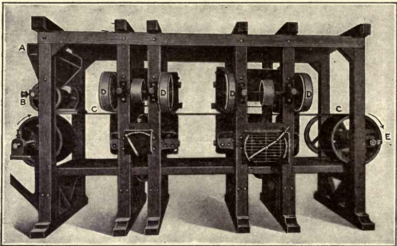
FIG. 33.—WETHERILL-ROWAND SEPARATOR.
