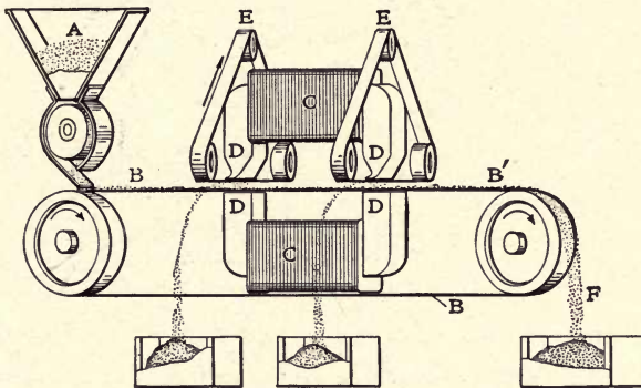
FIG. 32.—SKETCH SHOWING PRINCIPLE OF WETHERILL-ROWAND SEPARATOR.
