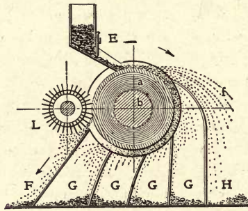
FIG. 2. Cross Section
