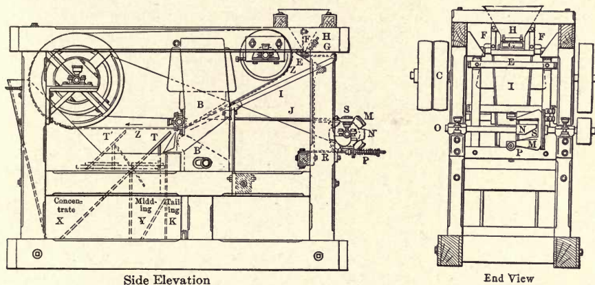
FIG. 30. — THE KNOWLES SEPARATOR.
