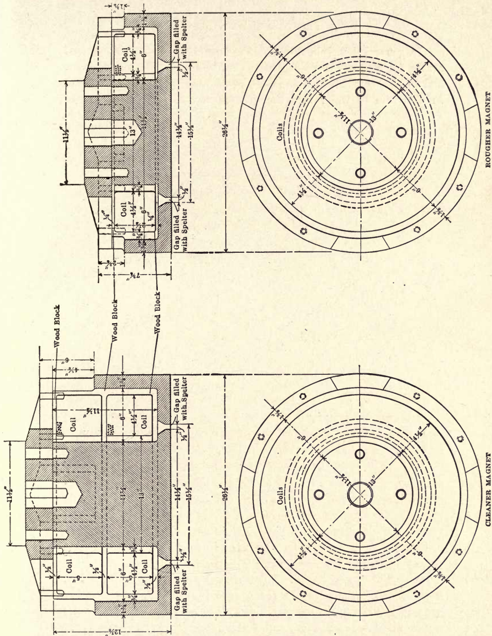
FIG. 21. — DETAIL OF MAGNETS, CLEVELAND-KNOWLES SEPARATOR.
