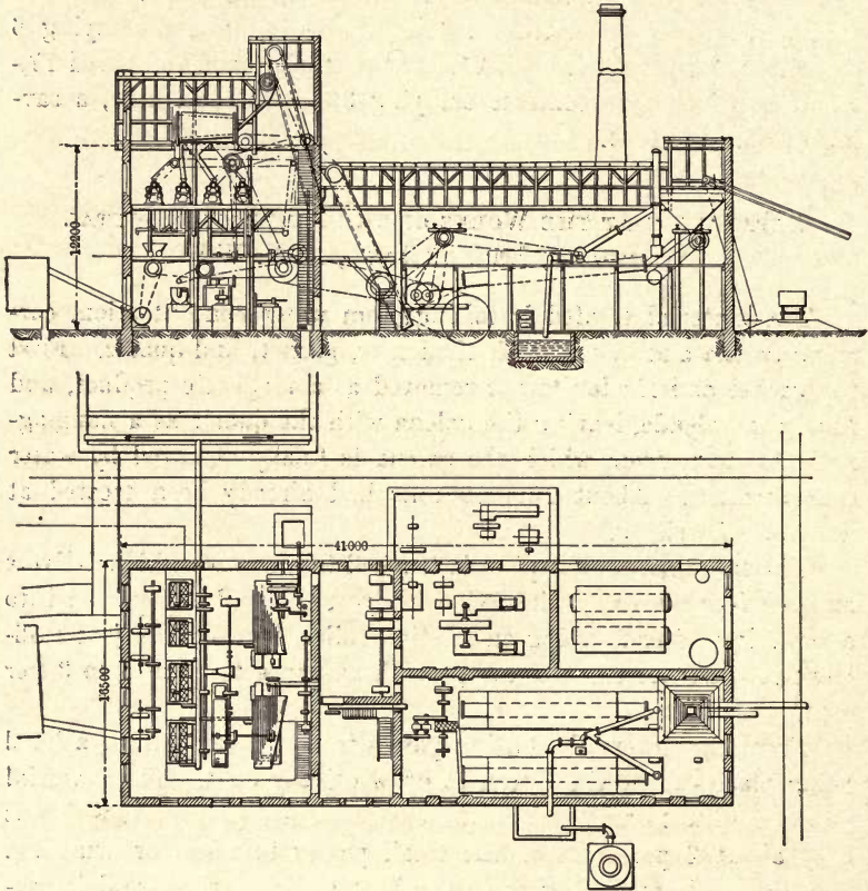
FIG. 81.—PLAN AND SECTION OF THE SEPARATION PLANT, AUSTRALIAN METAL CO.
