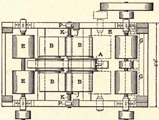
FIG. 49.—WETHERILL INCLINED SEPARATOR.
