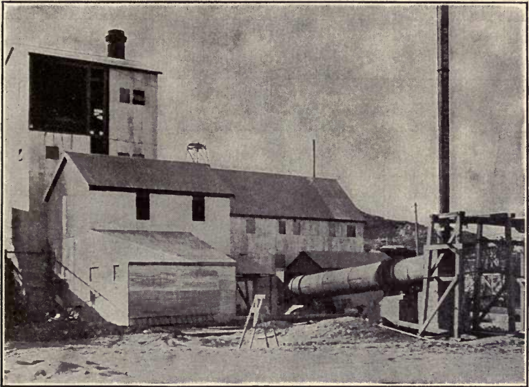
FIG. 76. — DRYING FURNACE, PLANT NO. 2, SULPHIDE CORPORATION.
