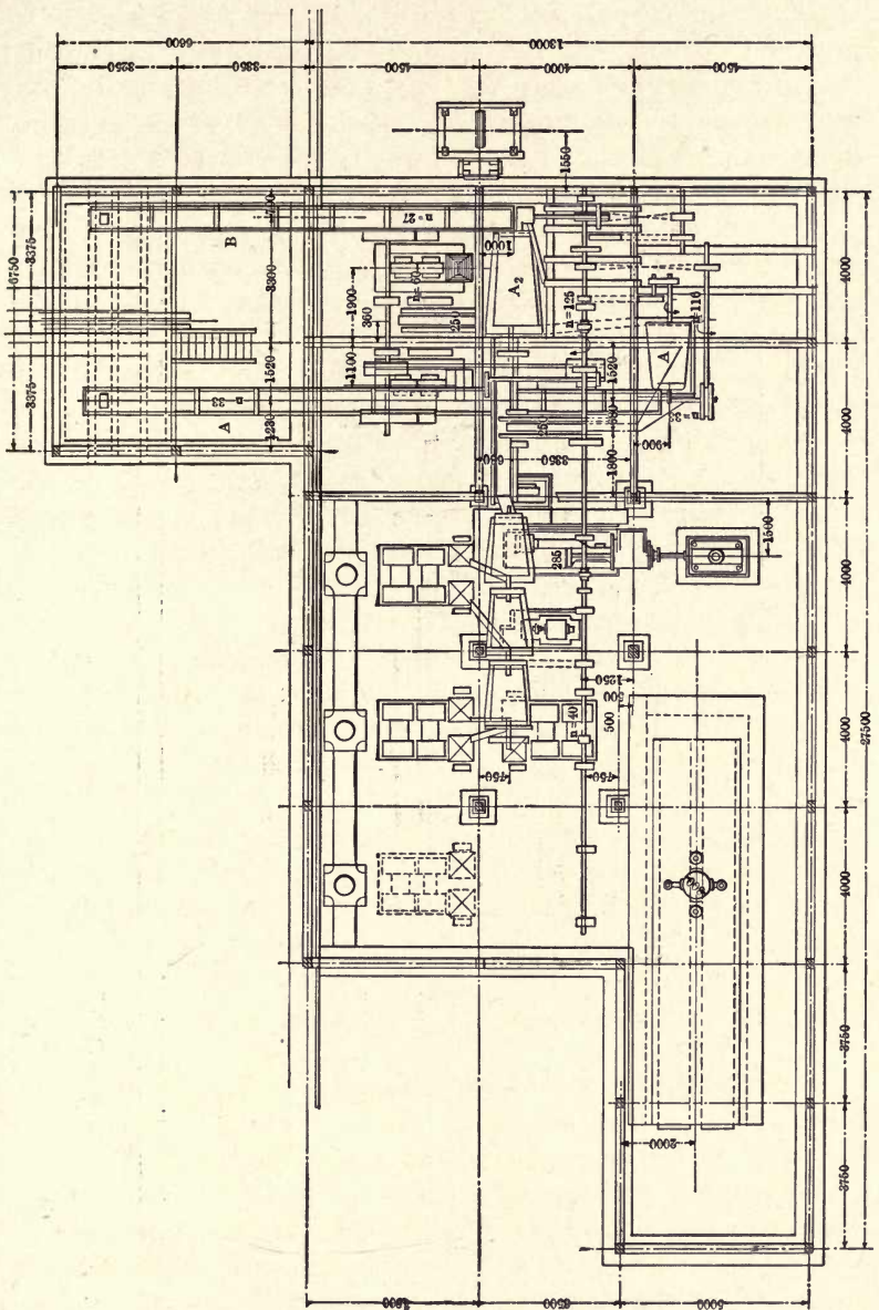
FIG. 63. — PLAN OF SEPARATION WORKS, NEUNKIRCHEN, GERMANY.
