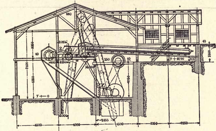
FIG. 65. — TRANSVERSE SECTION OF SEPARATION WORKS, NEUNKIRCHEN, GERMANY.
