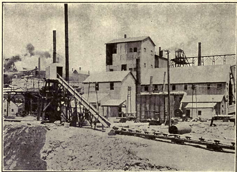
FIG. 75. — CONVEYOR FROM DUMP, PLANT NO. 2, SULPHIDE CORPORATION.
