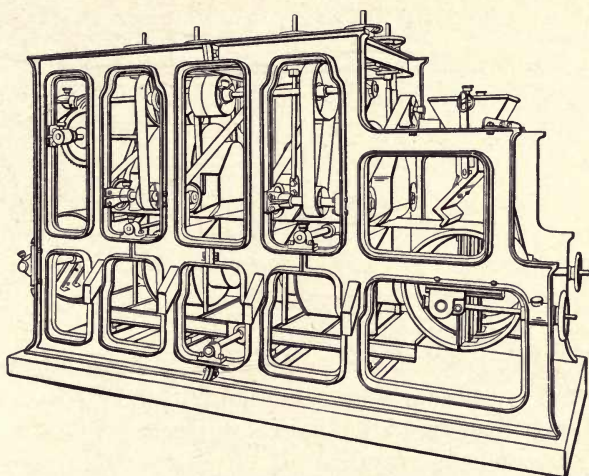
FIG. 35.—HUMBOLDT-WETHERILL CROSS-BELT SEPARATOR.
