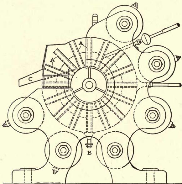
FIG. 22.—THE STERN-TYPE WET SEPARATOR. SIDE ELEVATION.
