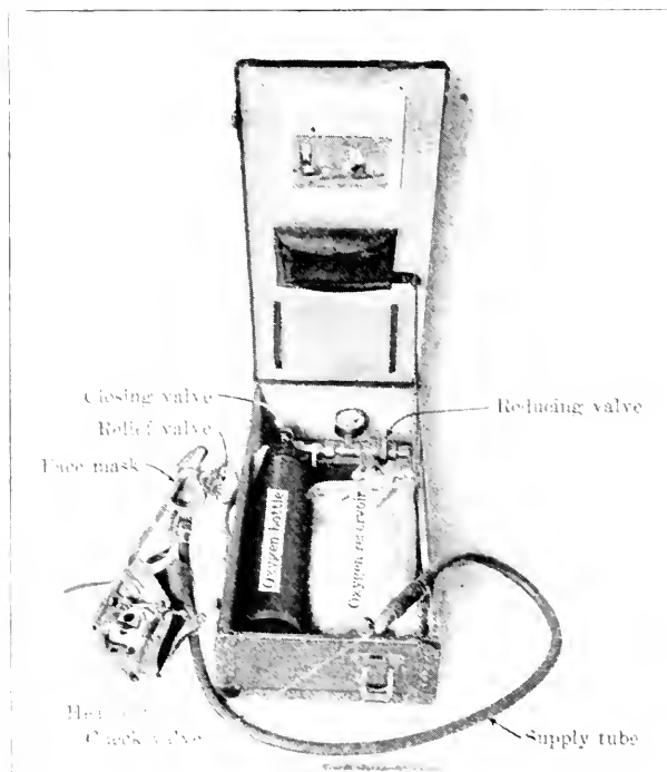
FIG. 61. Oxygen inhalator
