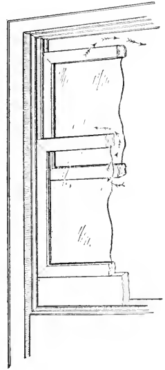
FIG. 52. Window ventilation in cold weather
