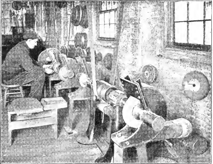
FIG. 53. Dust and safety hood
