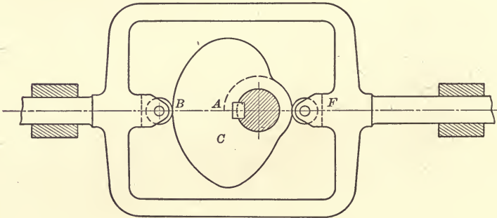
FIG. 9.—YOKE CAM
