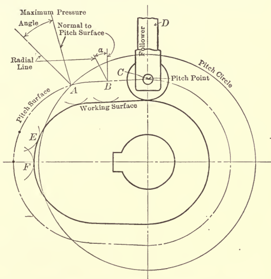
FIG. 20.—SHOWING NAMES OF SURFACES, LINES, AND POINTS OF A CAM
