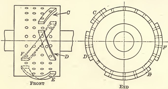
FIG. 11.—BARREL CAM
