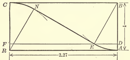
FIG. 23.—STRAIGHT-LINE COMBINATION CURVE
