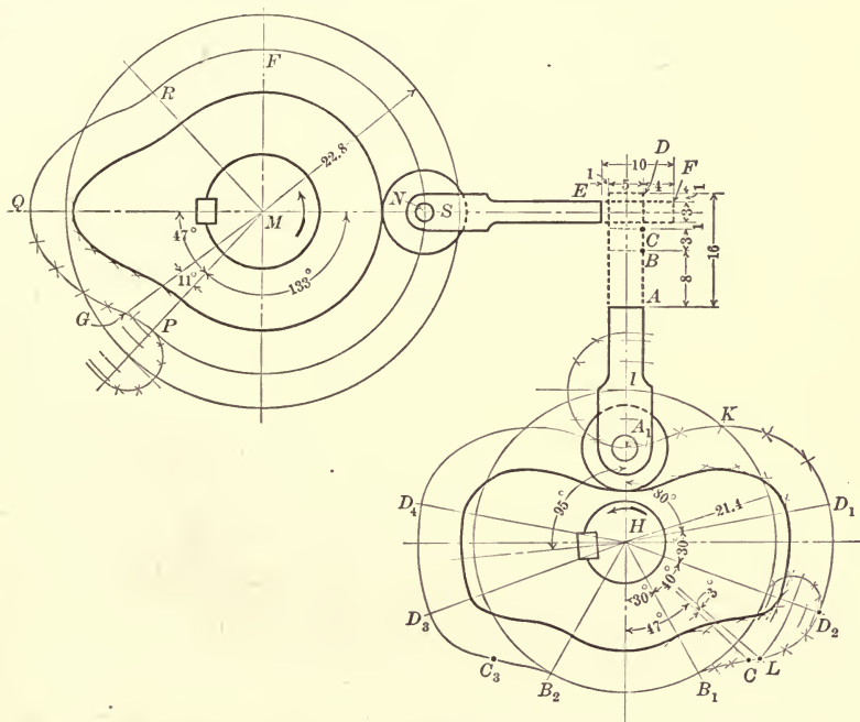
FIG. 64.—PROBLEM 17, DESIGN FOR DEFINITE TIMING AND NON-INTERFERENCE OF CAMS OPERATING IN SAME PLANE
