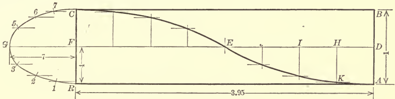
FIG. 26.—ELLIPTICAL CURVE
