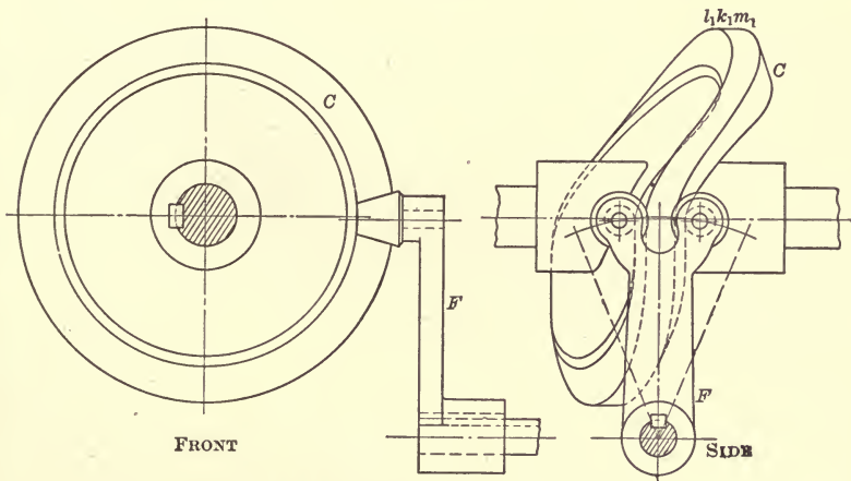
FIG. 10.—DOUBLE-END CAM
