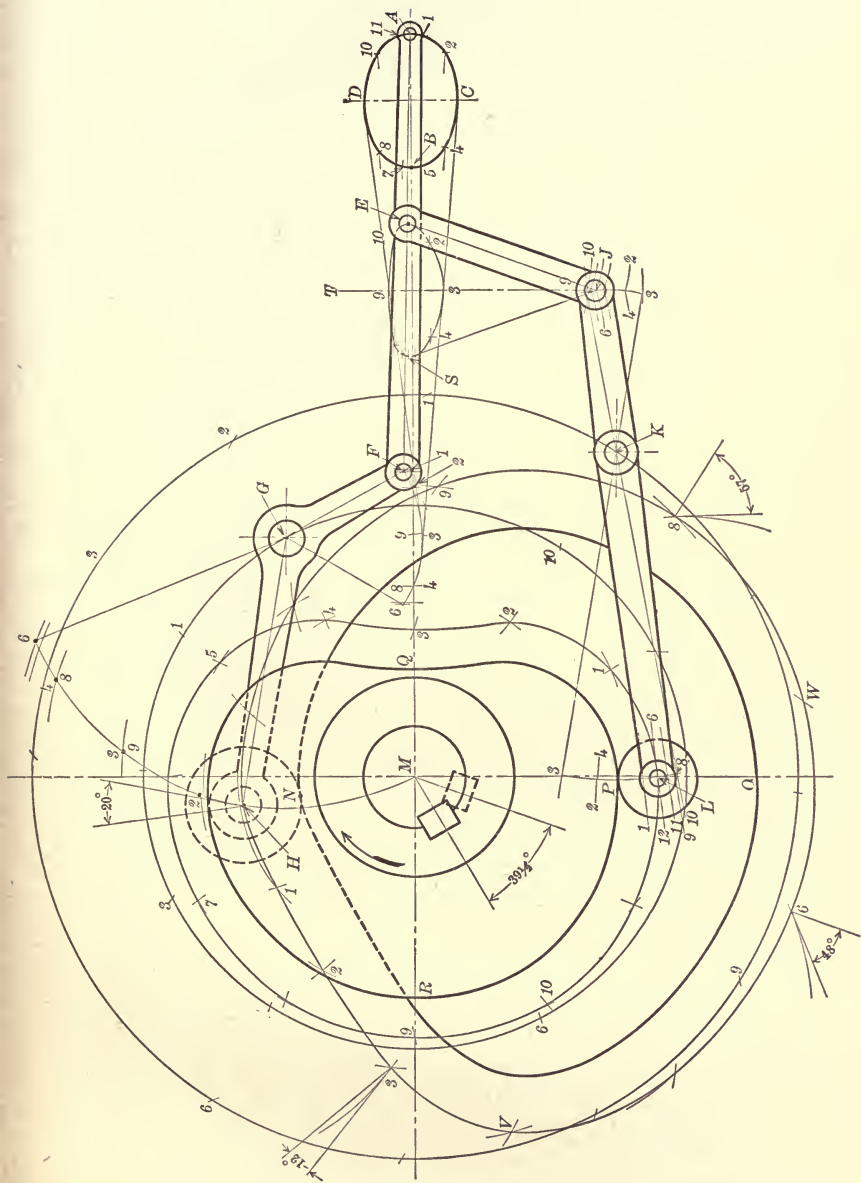
FIG. 66.—PROBLEM 18, CAM FOR DRAWING AN ELLIPSE
