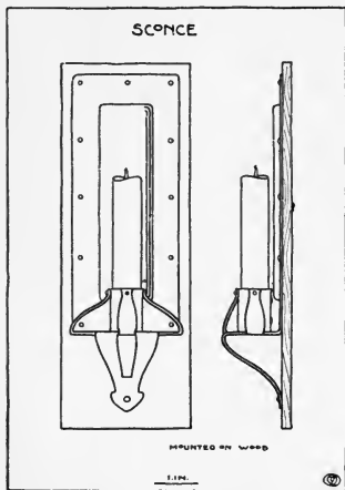
Design for a Copper Scence
