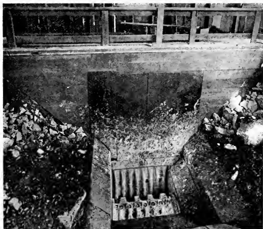
Courtesy of New York and New England Cement & Lime Co. Crusher Used in Breaking Cement Rock
