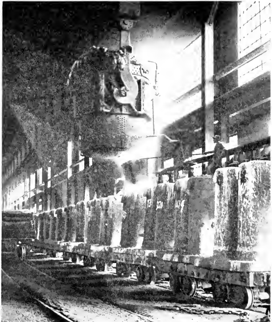
Pouring Molten Steel from Ladle into Ingot Molds
