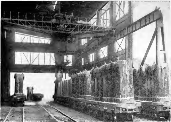
Removing the Ingot Molds from the Steel Ingots as soon as the Metal has Hardened
