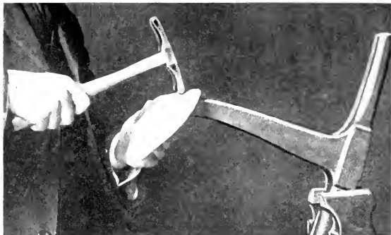
Hammering a Small Bowl out of Sheet Copper (Early Stage)
