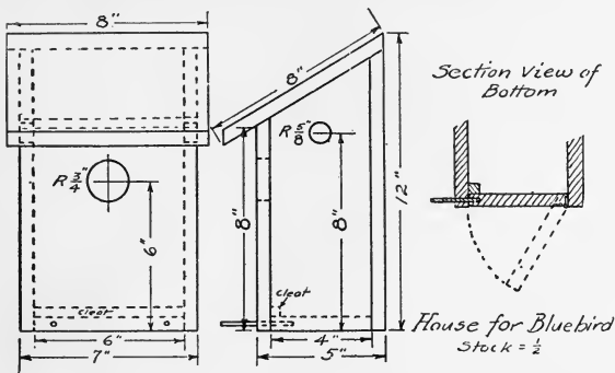
Working Drawing of a Bird House
