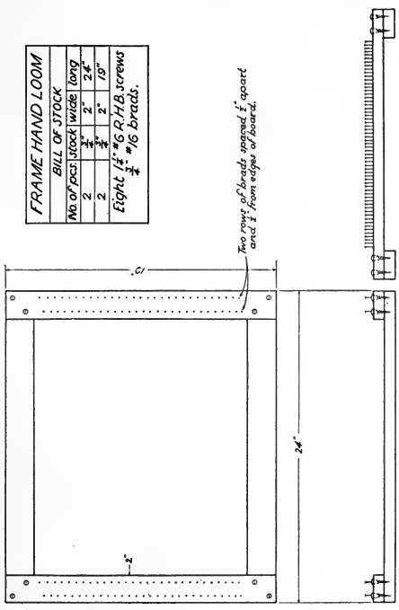
Working Drawing of the Loom Frame
