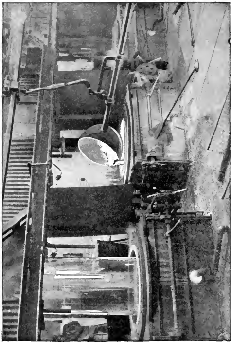
Pouring Metal for Blowing Window Glass Cylinders by Machine
