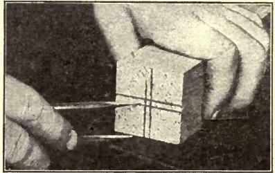
Fig. 3. Using the Compasses to Find the Center.
