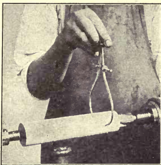
Fig. 58. Using Calipers.
