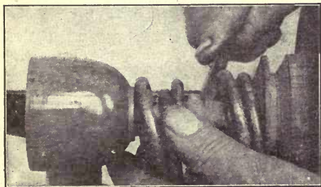
Fig. 121. Turning Between Rings.
