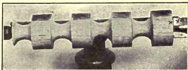
Fig. 52. Bead and Cove, Coves Completed.
