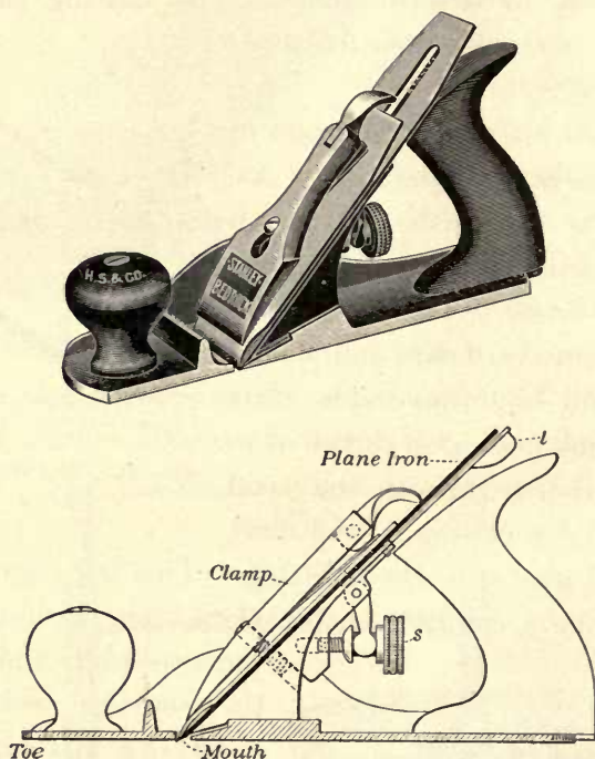
FIG. 22. Sectional Views of Iron Plane
