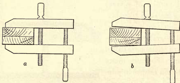
FIG. 52. Method of using the Hand Screw
