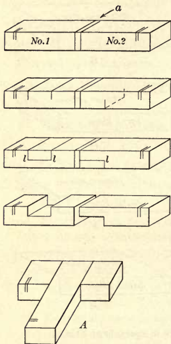
FIG. 50. Successive Steps in laying out and making a Middle Lap Joint
