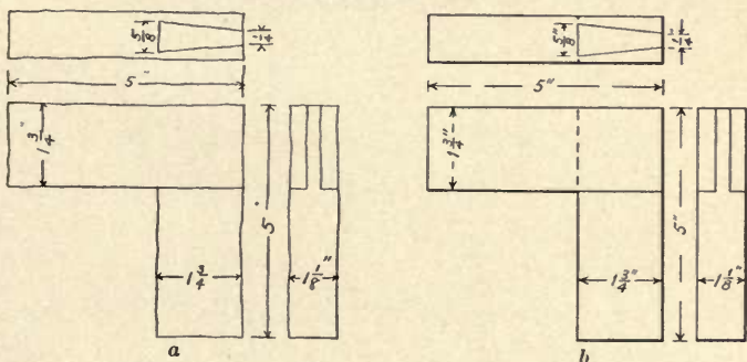
FIG. 62. Drawings of a Single Dovetail Joint
