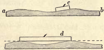
FIG. 25. Action of Short and Long Planes
