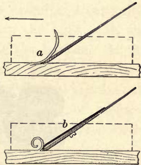
FIG. 20. The Plane Iron in Action
