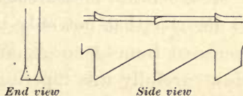
FIG. 13. Teeth of Ripsaw
