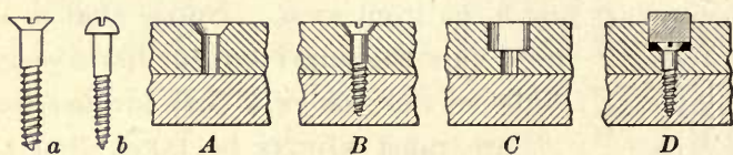
FIG. 55. Methods of using Screws
