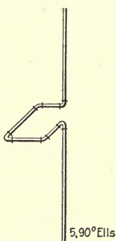
FIG. 74.—Expansion loop. Five 90° ells.
