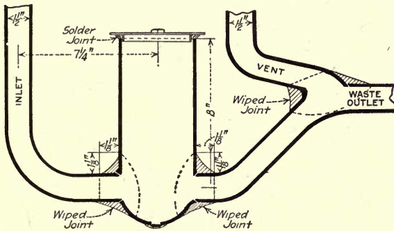
FIG. 34.—Drum trap.
