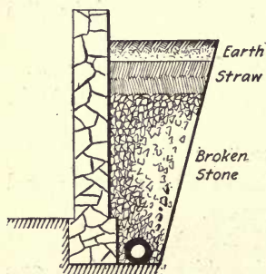
FIG. 45.—Sub-soil drain.
