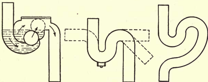
FIG. 64.—Mechanical-seal trap. FIG. 65.—Standard "S" trap. FIG. 66.—Bag trap.
