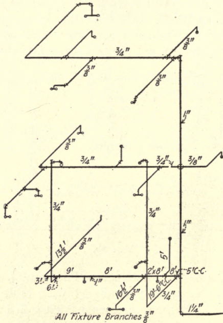
FIG. 81.—Pipe sketch.
