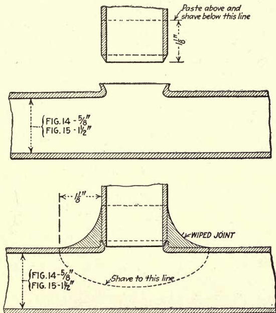
FIG. 30.—Branch joint.
