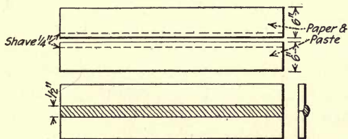
FIG. 20.—Flat seam.
