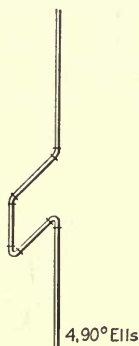
FIG. 73.—Expansion loop. Four 90° ells.
