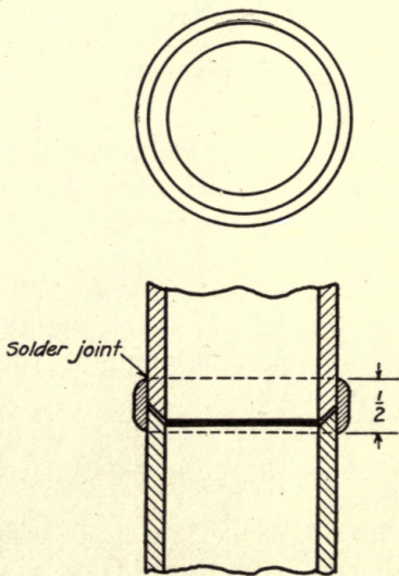
FIG. 19.—Over-cast joint.
