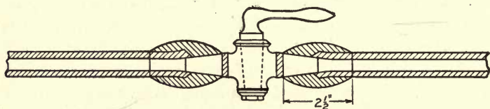
FIG. 29.—Stop cock.
