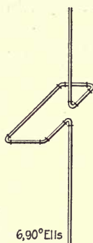
FIG. 75.—Expansion loop. Six 90° ells.
