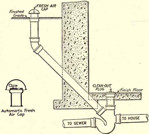
FIG. 60.—Fresh-air inlet.
