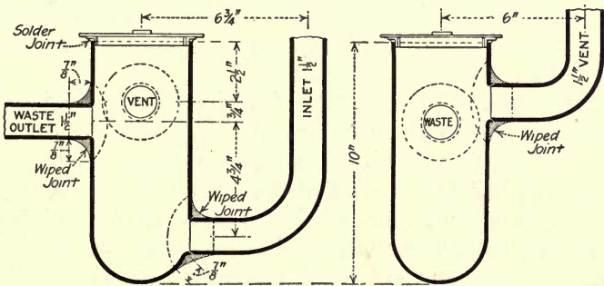
FIG. 33.—Drum trap.
