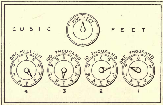
FIG. 77.—Gas-meter dials.
