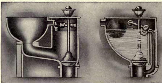
FIG. 3.—Plunger closet.
