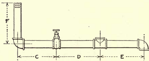
FIG. 69.— F reads center of ell to end, C reads center of ell to center of valve, D reads center of valve to center of T, E reads center of T to center of ell.
