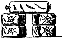
PLATE 22.—Methods of constructing loopholes with sandbags.
