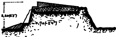
PLATE 27t.—Road embankment, defended from the rear.
