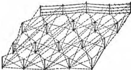
PLATE 4a.—Plan of wire entanglement.
