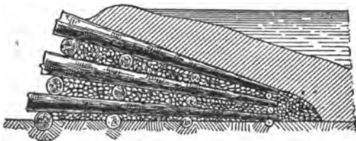
PLATE 10.—Dam construction.
