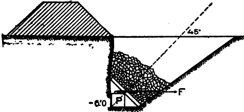
PLATE 8.—Fougass.
