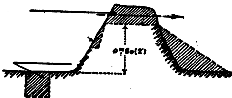
PLATE 27i.—Low wall of earth, or earth and sand heaps, more than 2 feet high (two methods, A or B ).
