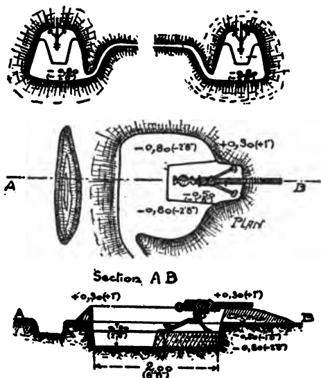
PLATE 27.—Type of cover for machine guns.
