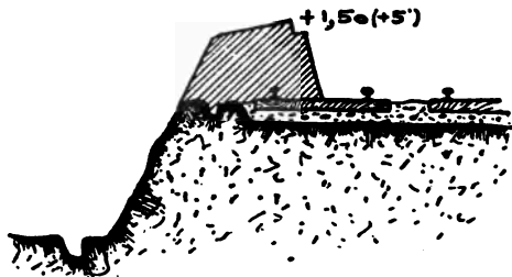
PLATE 27u.—Arrangement of a railroad embankment.
