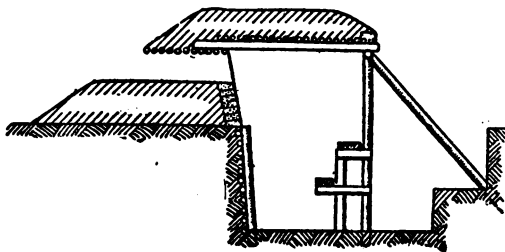
PLATE 20.—Overhead cover.
