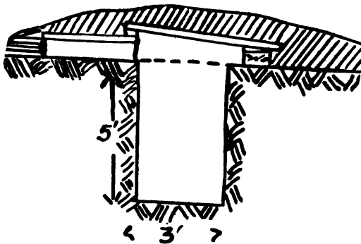
PLATE 12.—Covered type of listening post.
