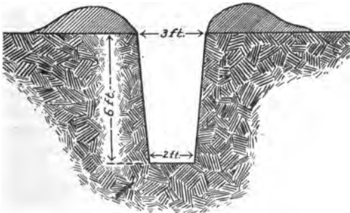
PLATE 23.—Type of communication trench.
