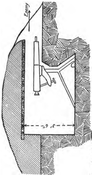
From World's Work. PLATE 26.—Profile of type of cover for machine gun.
