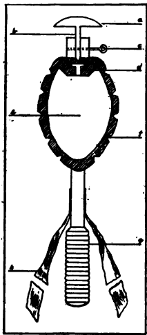
PLATE 41c.—The latest type British hand grenade.
