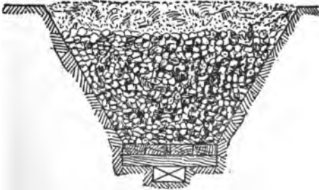
PLATE 9.—Vertical fougass.
