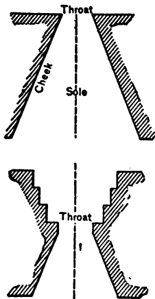
PLATE 21.—Types of loopholes.
