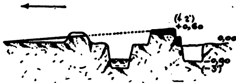
PLATE 27q.—Arrangement of a ditch full of water.
