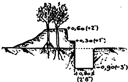
PLATE 27v.—Arrangement of a sunken road.
