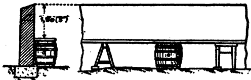
PLATE 28.—Arrangement of a wall more than 8 feet high without making loopholes.
