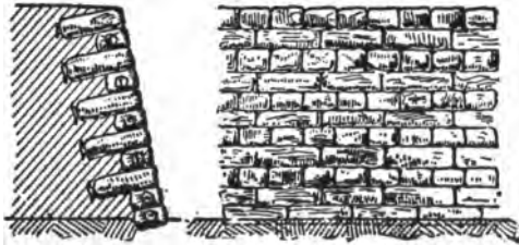
PLATE 29.—Sandbag revetment.
