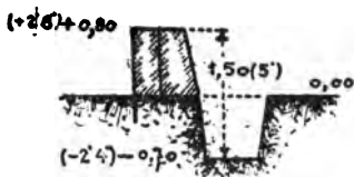
PLATE 27y.—Arrangement of a wall 2 feet 8 inches high.
