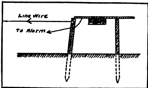
PLATE 5a.—Alarm trap.
