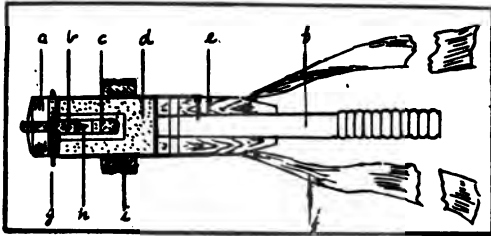
PLATE 41b.—British hand grenade No. 1.
