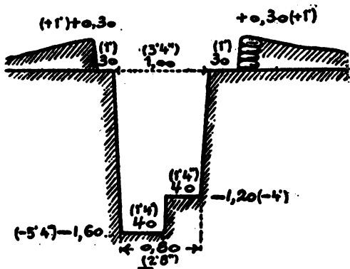
PLATE 11.—Open type of listening post.
