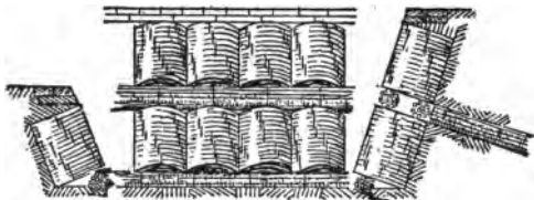
PLATE 37.—Methods of use of gabion.
