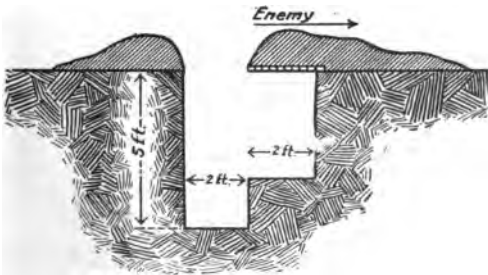
PLATE 19a.—Overhead cover.
