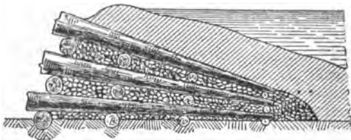
PLATE 10.—Dam construction.
