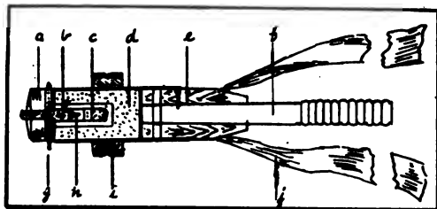
PLATE 41b.—British hand grenade No. 1.
