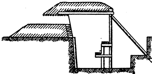
PLATE 20.—Overhead cover.
