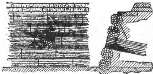
PLATE 31.—Fascine revetment.
