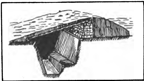
PLATE 20a.—Overhead cover.
