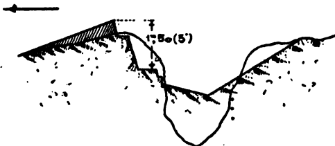
PLATE 27p.—Arrangement of a large ditch.
