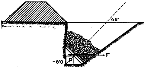
PLATE 8.—Fougass.
