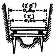
PLATE 17.—Details of trench drainage.
