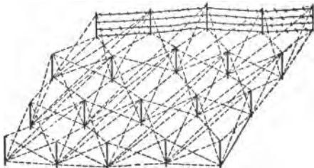
PLATE 4a.—Plan of wire entanglement.
