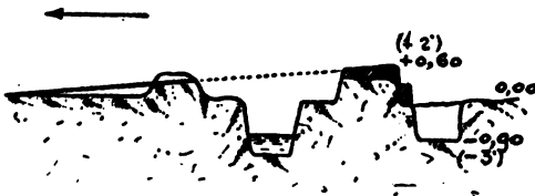
PLATE 27q.—Arrangement of a ditch full of water.
