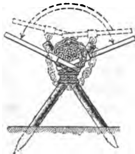
PLATE 30.—Method of using the fascine choker.
