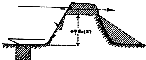
PLATE 27i.—Low wall of earth, or earth and sand heaps, more than 2 feet high (two methods, A or B).
