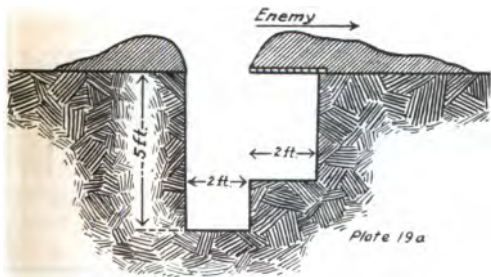
PLATE 19a.—Overhead cover.
