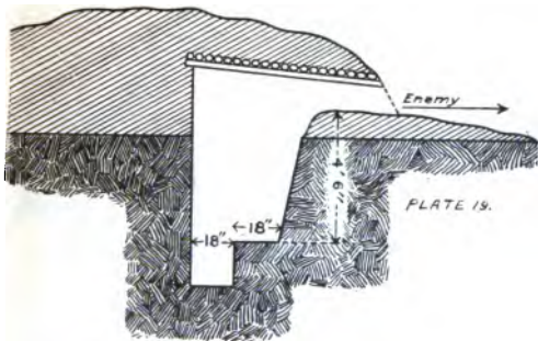
PLATE 19.—Overhead cover.
