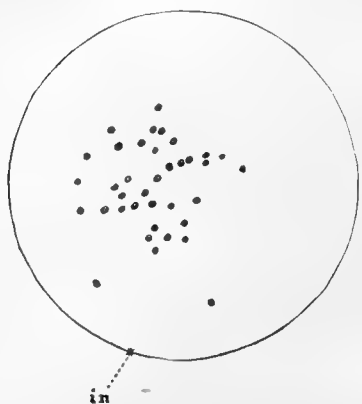
FIG. 6.—Diagram of egg in invagination stage, constructed from serial sections, to show all the primary yolk nuclei present. For details of this egg, see Table I (II, a ), Invagination. in = point of invagination, nearly in the plane of the paper.
