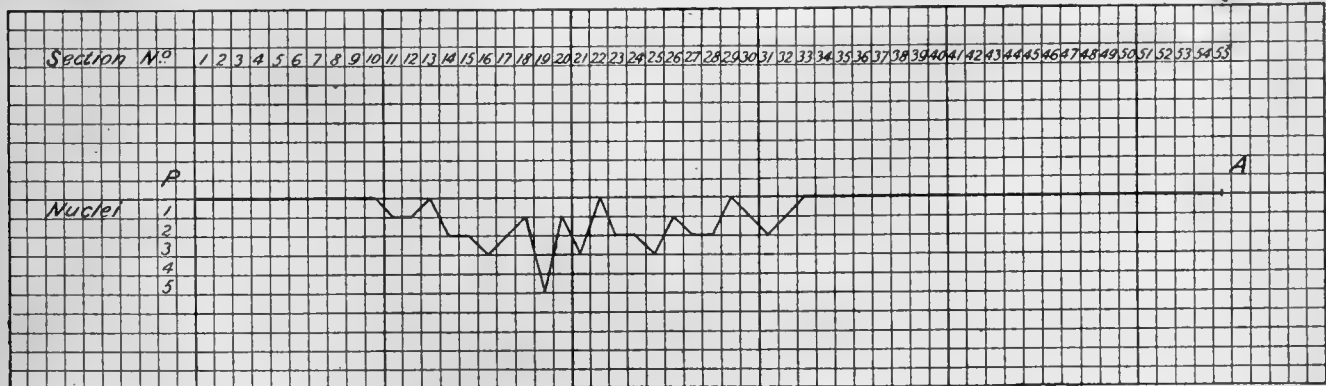
FIG. 9.—Curve showing the distribution of the primary yolk nuclei in the invagination stage, egg No. II, b, Table I. (Compare with Fig. 7.)
