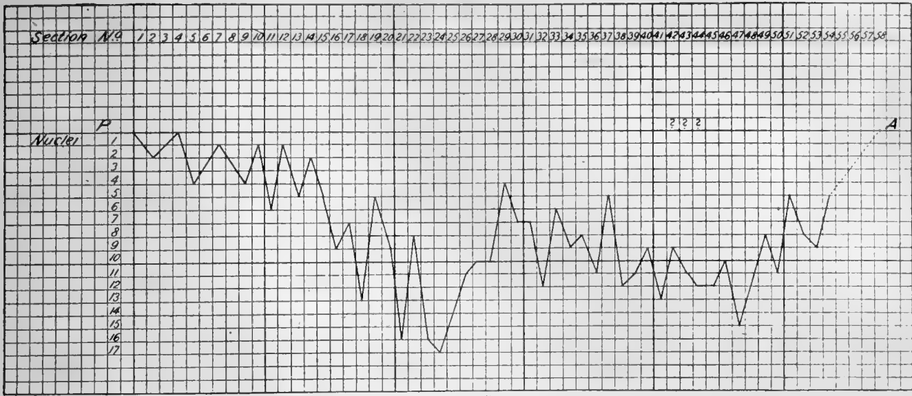
FIG. 8.—Curve showing distribution of all nuclei, exclusive of primary yolk nuclei, in the same egg as represented by Figs. 6 and 7. (See Table I, Invagination stage, II, a.) A, Anterior; P, Posterior; Abp, Ventral plate; EA, Embryonic area.
