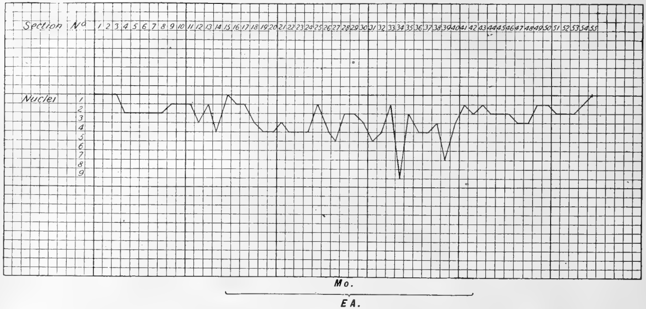
FIG. 12.—Curve showing distribution of wandering cells in Stage V (Early egg-nauplius). (Compare Fig. 11, and for details, see Table I, Stage, II b.) E A, Embryonic area; Mo, Mouth.
