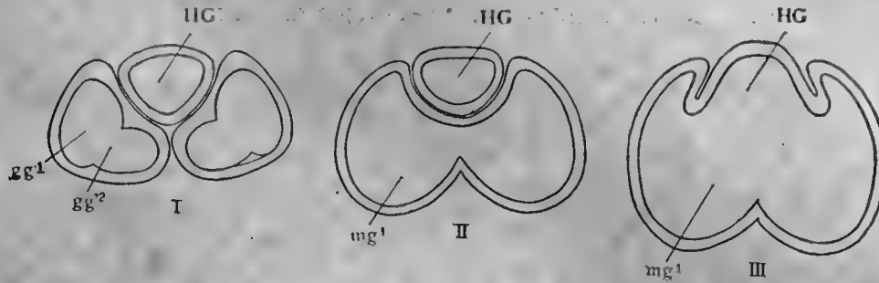
FIG. 1.—Diagrams of transverse sections through the alimentary tract of an embryo of Alphacis sauleyi which is nearly ready to hatch, to show the origin of the gastric gland from the postero-lateral lobes of the midgut. Section I cuts the hindgut and lobes of the "liver," Section II the hindgut where it merges into the mesenteron. gg^1 , gg^2 , Secondary lobules of mg^1 ; HG, hindgut; mg^1 , postero-lateral lobes of midgut.
