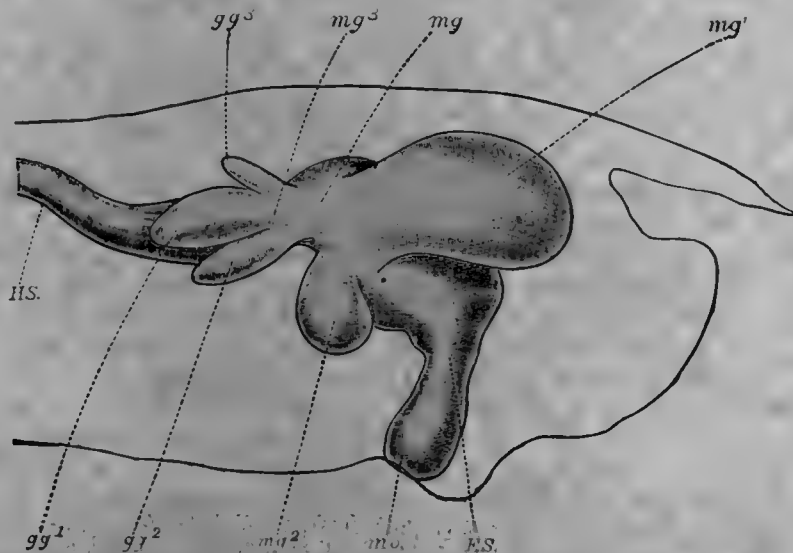
FIG. 2.—Semi-diagrammatic representation of the alimentary tract and its appendages in the first larva of Alphacis sauleyi . The middle line of the body is also shown. FS, foregut; gg^1 - gg^3 , secondary lobules of postero-lateral lobe of midgut; HS, hindgut; mg, midgut; mg^1 - mg^3 , anterior, lateral, and postero-lateral divisions of midgut; mo, mouth.
