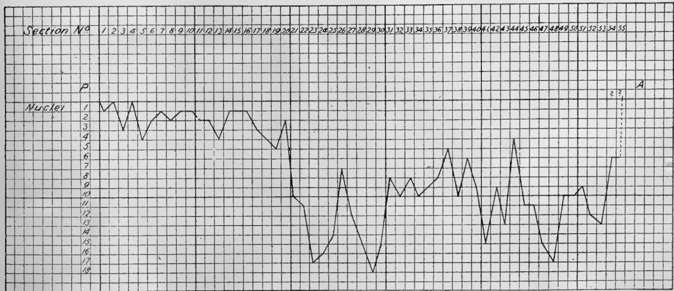
FIG. 10.—Curve showing distribution of all nuclei, exclusive of primary yolk nuclei, in the same egg as represented by Fig. 9. (See II, b, Table I, and compare with Fig. 8.) A, Anterior; P, Posterior; Abp, Ventral plate; EA, Embryonic area.
