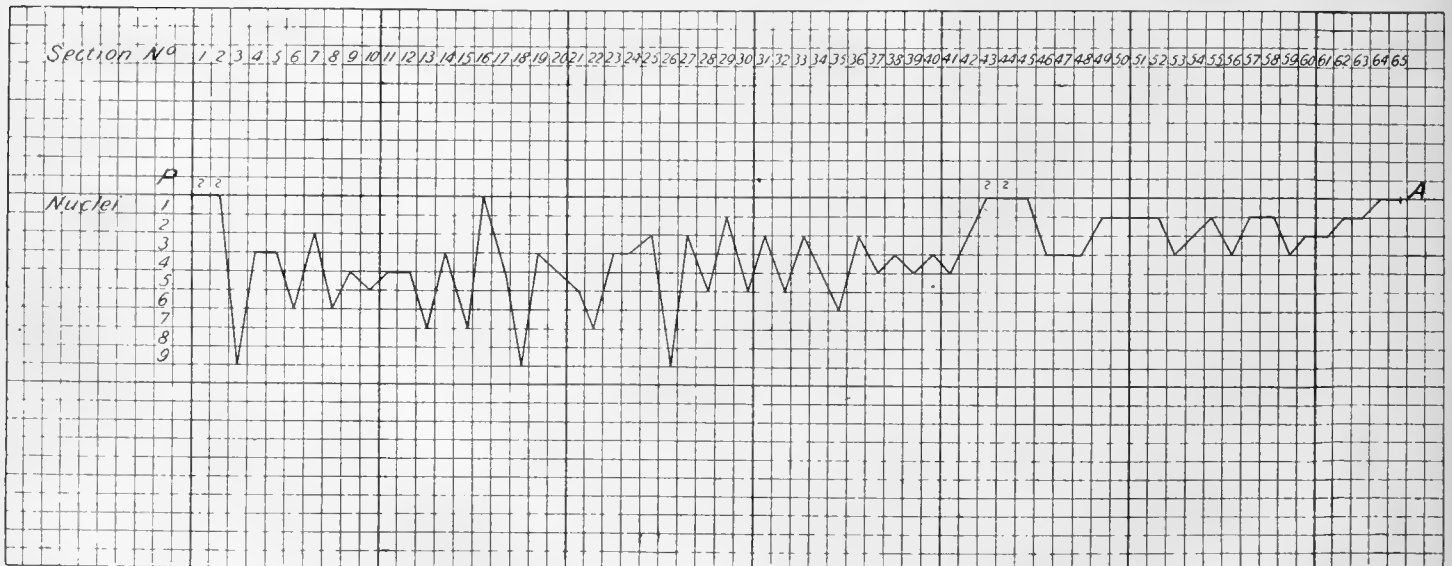
FIG. 13.—Curve showing the distribution of wandering cells in Stage V, \alpha . (v. Table I.) A, Anterior; P, Posterior.
