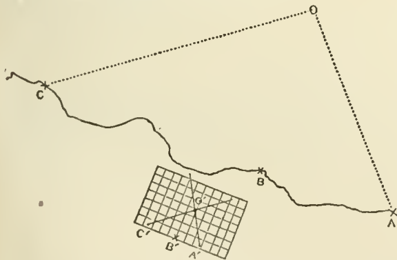
FIG. 31.—Watkin Position-finder.
