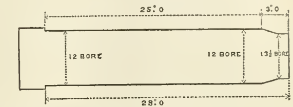
FIG. 10.—Greener's choke.
