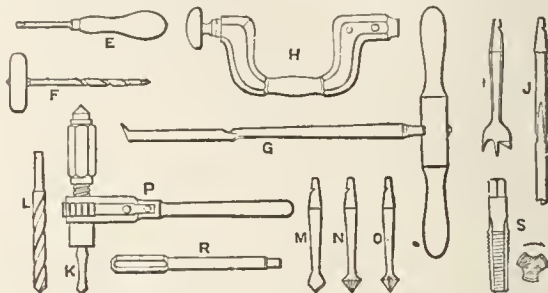
FIG. 5.—Boring tools.
