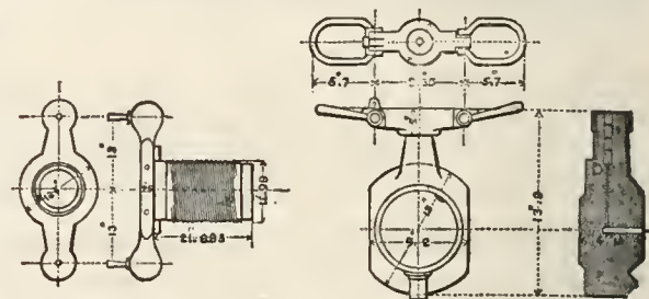
FIG. 42.—Breech Screw.
