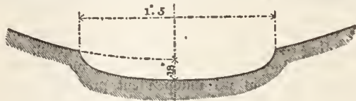
FIG. 33.—8-inch Howitzer (section of grooves).
