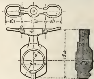
FIG. 43.—Vent Piece.
