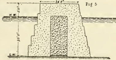
ANSTRUTHER BREAKWATER.
