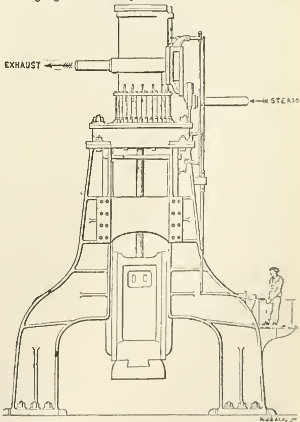
FIG. 4.—Steam Hammer.
