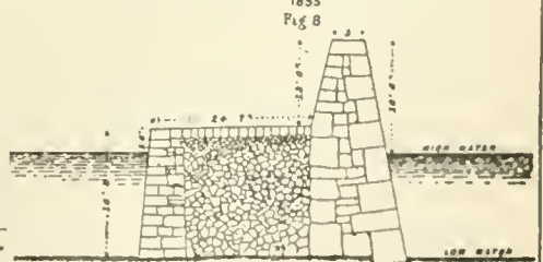
NETHER BUCKIE, 1855.
