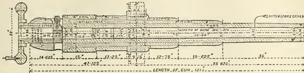
FIG. 25.—40-pounder Armstrong Rifled Breech-loader.
