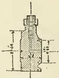
FIG. 28.—40-pounder Vent Piece (section).
