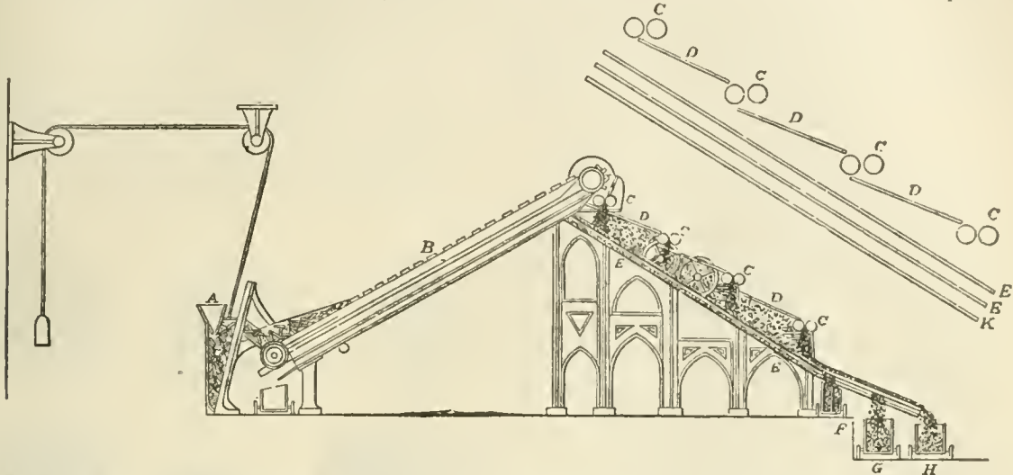
FIG. 6.—Granulating machine. A, bopper, with raising arrangement; B, endless band; C,C,C,C, four pairs of rollers; D,D,D, short screens; E,E, long screens; F, box for dust; G, box for grain; H, box for chucks; K, bottom board.
