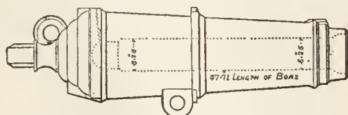
FIG. 21.—32-pounder Carronade.
