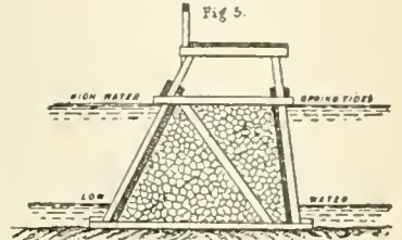
BLYTH BREAKWATER, 1858.
