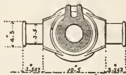
FIG. 36.—13-pounder of 8 cwt. (front view).
