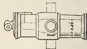
FIG. 24.—Coehorn Howitzer.
