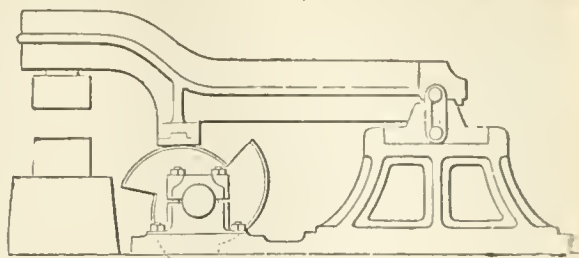
FIG. 2.—Lift Hammer.
