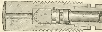
FIG. 8.—Crusher gauge.
