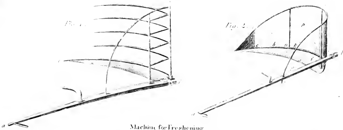
Machine for Freshening SEA WATER
