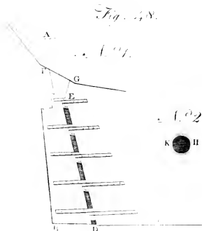
BOSWELL'S improved CAPSTAN.
