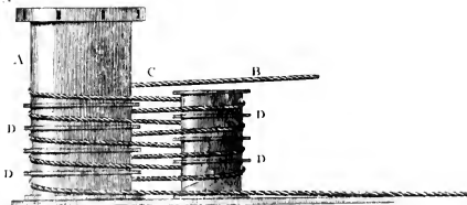
BOSWELL'S improved CAPSTAN.
