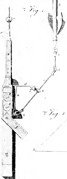
SOUNDING Machine.
