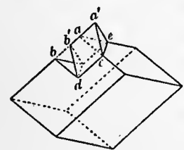
FIG. 91.—Glide-plane of Calcite.
