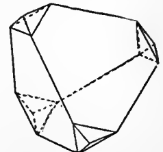
FIG. 33.—Combination of Tetrahedron and Rhombic Dodecahedron.
