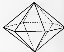
FIG. 70.—Hexagonal Bipyramid.
