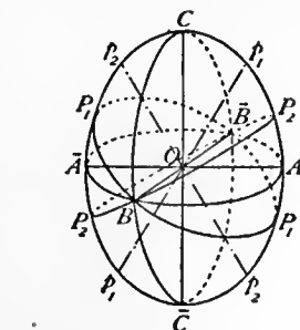
FIG. 98.—Optical Indicatrix of a Biaxial Crystal.
