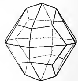
FIG. 35.—Dyakis-dodecahedron.
