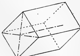
FIG. 57.—Brachy-prism and Macro-pinacoid.
