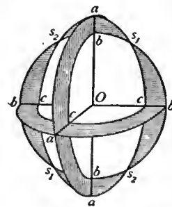
FIG. 99.—Ray-Surface of a Biaxial Crystal.
