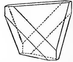
FIG. 31.—Combination of Tetrahedron and Cube.
