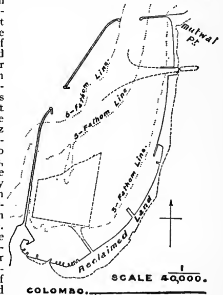
FIG. 5.—Colombo Harbour.
