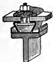
FIG. 7.—Rendle's "Invincible" Glazing.
