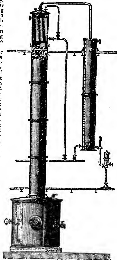
FIG. 4.—Benzol Still (elevation),
