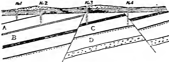
FIG. 1.—Proving by Boreholes.
