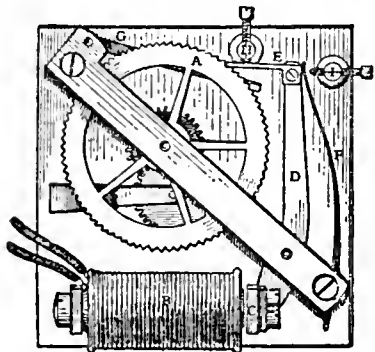
FIG. 33.—Hope Jones's Dial-driving Device.
