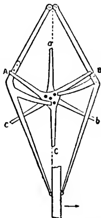
FIG. 20.—Double Three-legged Escapement.
