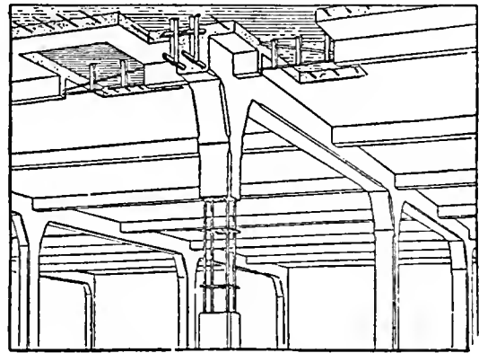
FIG. 3.—Hennebique System.
