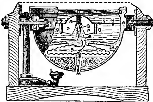
FIG. 5.—Liquid Compass.
