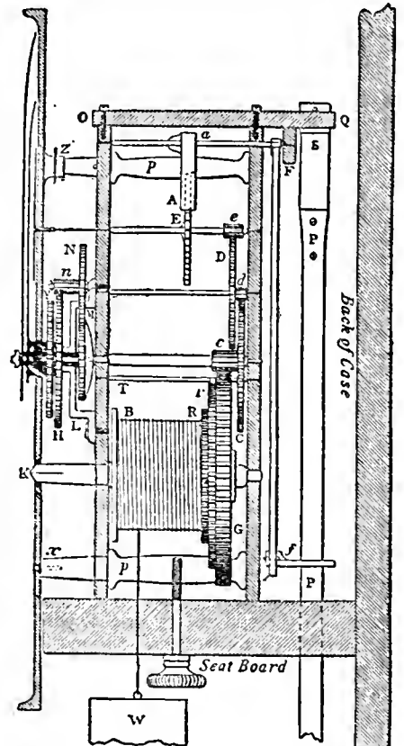
FIG. 3.—Section of House Clock.
