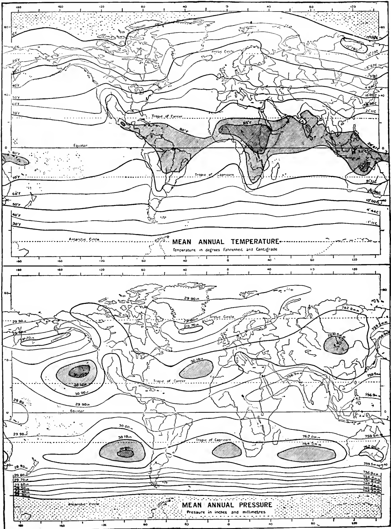
Annual Distribution of Temperature and Pressure.
