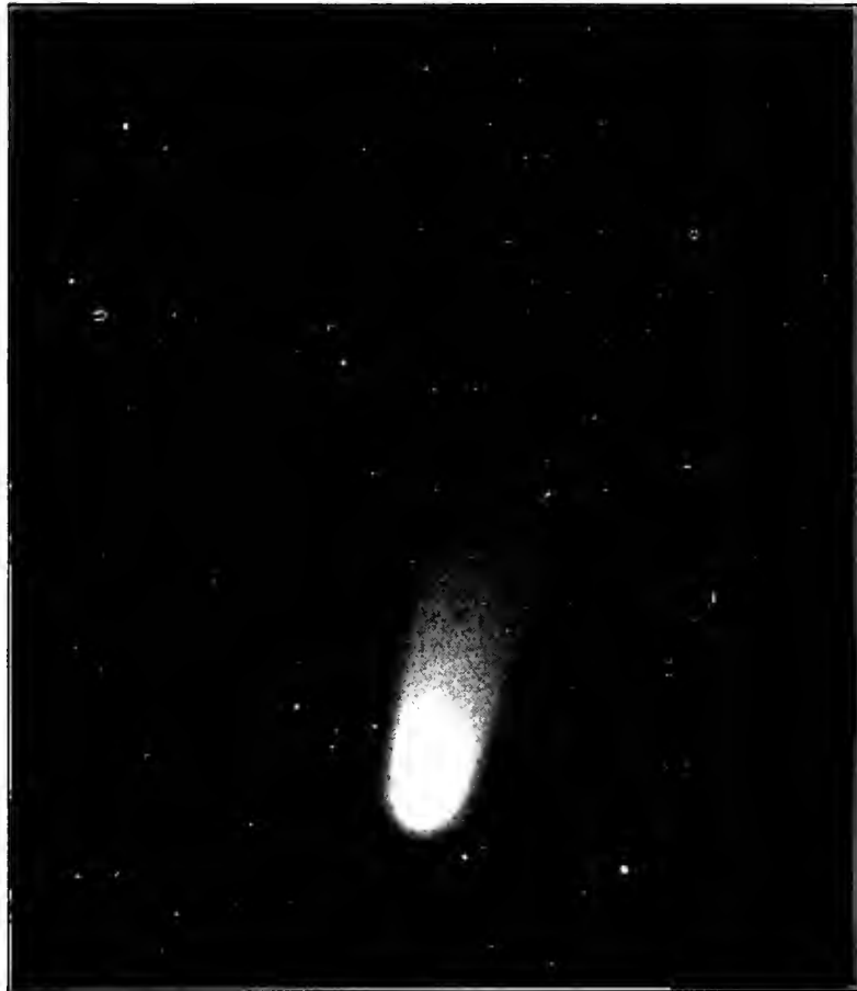
Fig. 3.—Halley's Comet, 1910, April 27.
