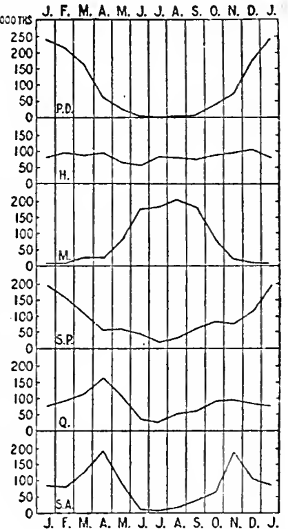
FIG. 5.—Annual march of rainfall in the tropics.
