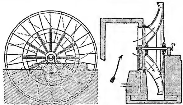
FIG. 13.—Waddle Fan.
