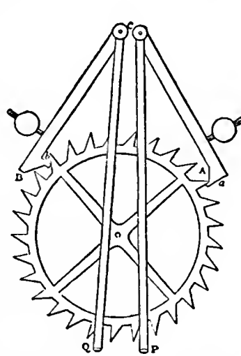
FIG. 17.—Mudge's Gravity Escapement.
