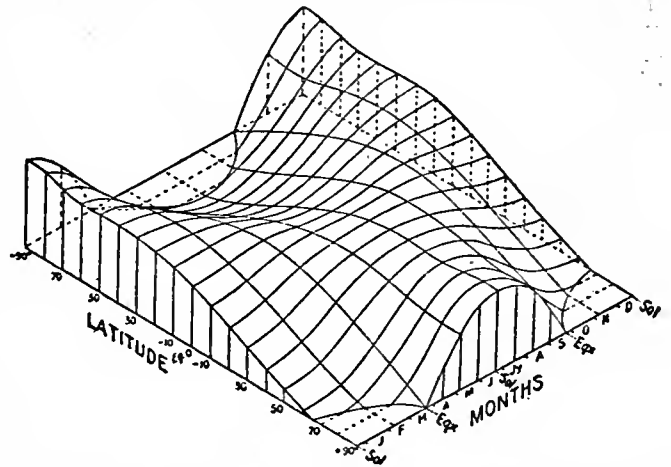
FIG. 1.—Distribution of Insolation over the Earth's Surface.
