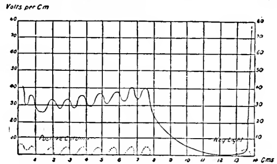
Pressure 2.25 m.m. Discharge in Hydrogen Current 0.568'10^-3 amperes
