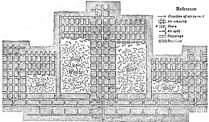
FIG. 5.—Pillar Working.
