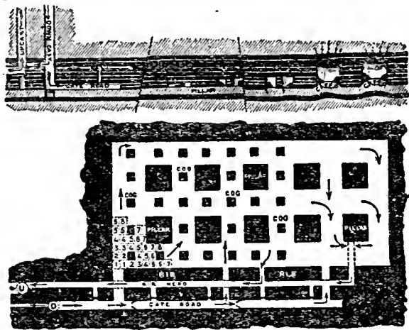
FIG. 9.—South Staffordshire method of working Thick Coal.
