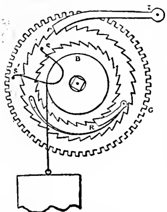
FIG. 25.—Harrison's Going-Ratchet.
