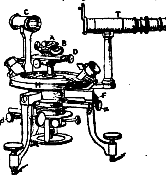
FIG. 3.—Horizontal-Circle Goniometer.
