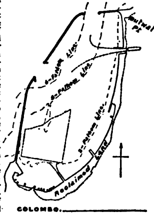
FIG. 5.—Colombo Harbour.
