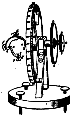
FIG. 2.—Vertical-Circle Goniometer.
