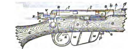
FIGS. 5 and 6.—Lee-Metford.
