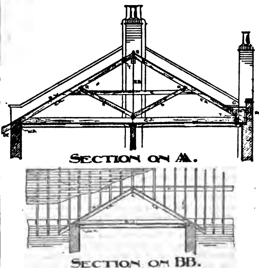
FIGS. 6 and 7.—Roof for Domestic Building.
