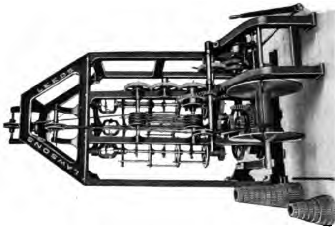
Fig. 18.—Haskell-Daves Vertical Rope Machine.
