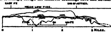
FIG. 14.—Deltaic Jetty Outlet, South Pass, Mississippi.
