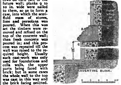
FIG. 4.—EXAMPLE OF MARBLE LINING, from the Cella of the Temple of Concord. A. Slabs of Phrygian marble. B. Plinth moulding of Numidian "giallo." C. Slab of cipollino (Carystian marble). D. Paving of porta santa. E and F. "nucleus" and "rudus" of concrete bedding. G, G. Iron clamps run with lead to fix marble lining. H. Bronze clamp. J. Cement backing.
