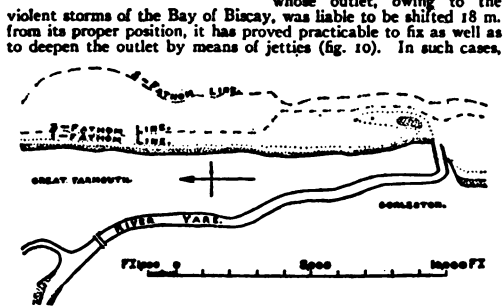
FIG. 10.—Shifting Outlet, fixed by Jetties: River Yare.
