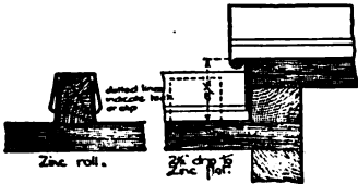
FIGS. 17 and 18.—Details of Zinc Flats.
