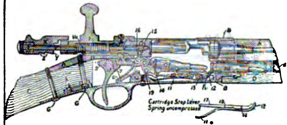
FIG. 16.—Lebel Rifle.
