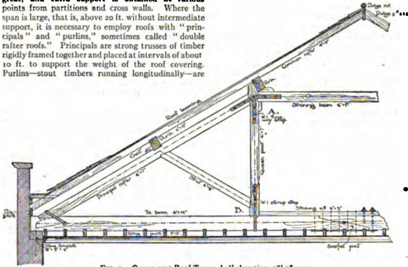
FIG. 3.—Queen-post Roof Truss; half elevation, 38' 0" span
