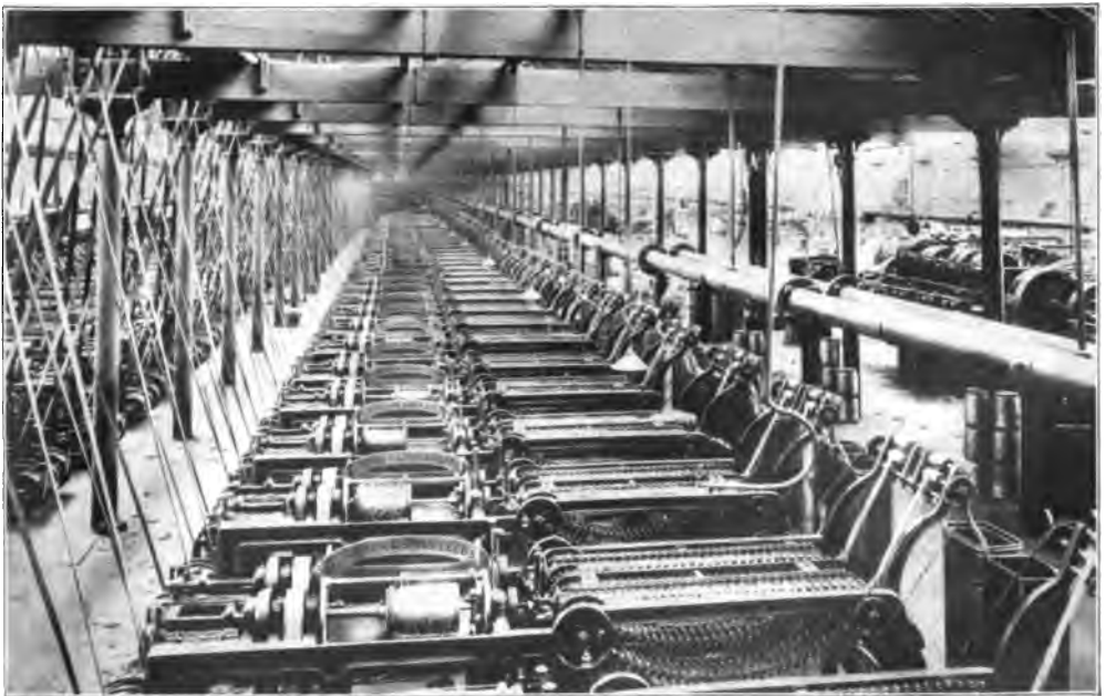
Fig. 15.—Binder Twine Spinning, Connswater Mill.
