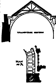
FIGS. 15 and 16.—Westminister Cathedral: choir-vaulting.
