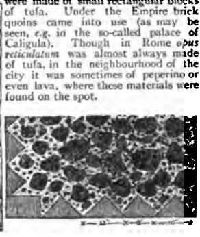
FIG. 3.—SECTION OF CONCRETE WALL, showing the use of bricks merely as a facing.
