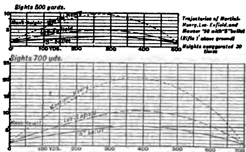
FIG. 20.—Trajectories.
