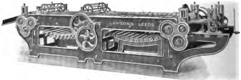
Fig. 11.—Good's Hackling and Spreading Machine.
