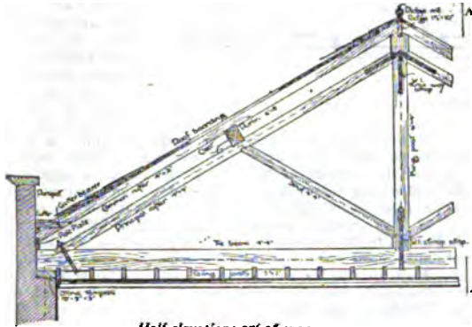
Figs. 1 and 2.—King-post Roof Truss.
