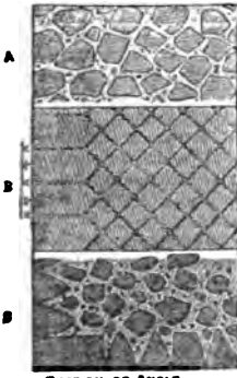
FIG. 2.—SECTION OF ANGLE faced with (A) Opus Incertum and (B) Opus Reticulatum. C shows the section, similar in both.
