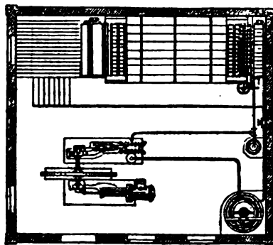
FIG. 6.—General Arrangement of an Ice Factory.
