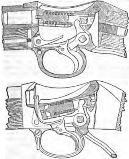
FIG. 2.—Martini-Henry.
