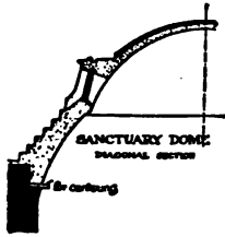
FIG. 14.—Westminister Cathedral: diagonal section through sanctuary dome.
