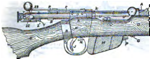
FIGS. 7 and 8.—Lee-Metford.
