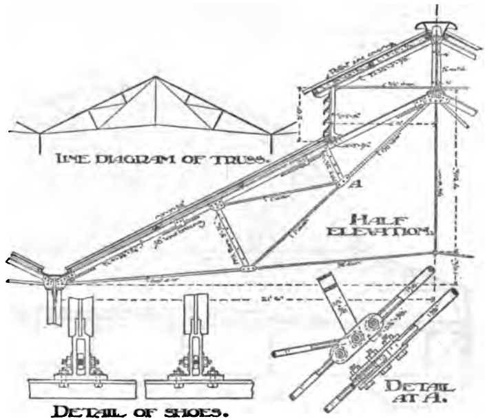
FIG. 10.—Roof at Cardiff Station.
