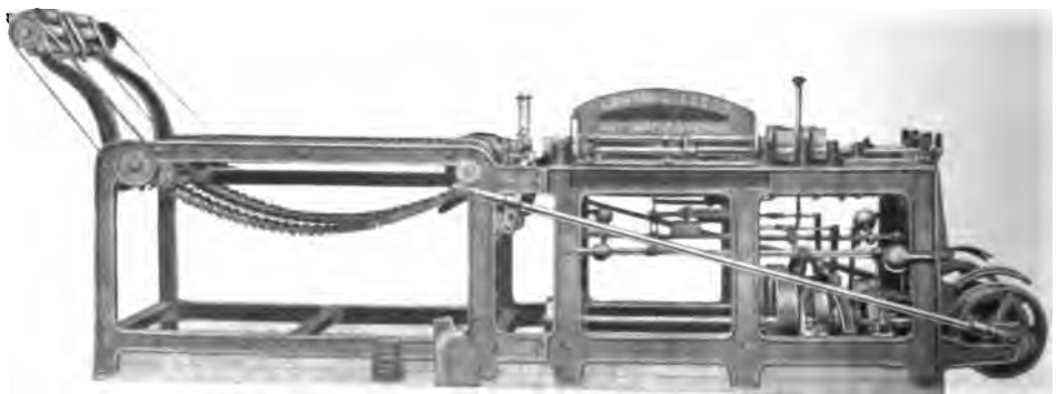
Fig. 13.—Spinner or Jenny.
