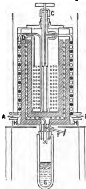
FIG. 2.—Laboratory Liquid Air Machine.
