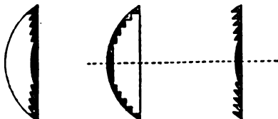
FIG. 31.—Buffon's Lens.
