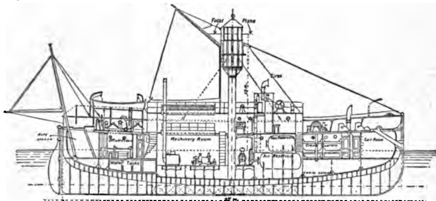
Longitudinal Section FIG. 47.—Sandettié Lightship.
