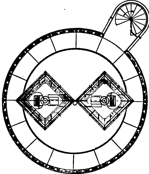
FIG. 43A.—The Vierge Apparatus and Lantern. Plan at focal plane.
