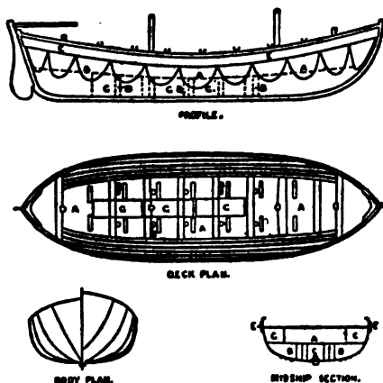
FIG. 4.—Plans, Profile and Section of Cromer Type of Life-boat. A, Deck. C, Side air-cases above deck. B, Relieving valves for automatic discharge of water off deck. E, Wale, or fender. G, Water-ballast tanks.
