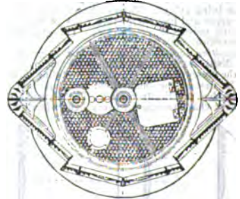
FIG. 39.—Pendeen Apparatus. Plan at Focal Plane.
