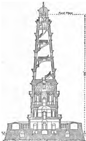
FIG. 1.—Cordouan Lighthouse.
