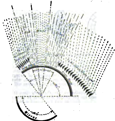
FIG. 38.—Gage Roads Direction Light.
