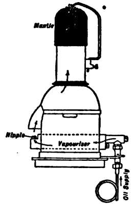
FIG. 44.—"Chance" Incandescent Oil Burner, with 85 mm. diameter mantle.
