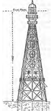
FIG. 26.—Cape San Thomé Lighthouse.
