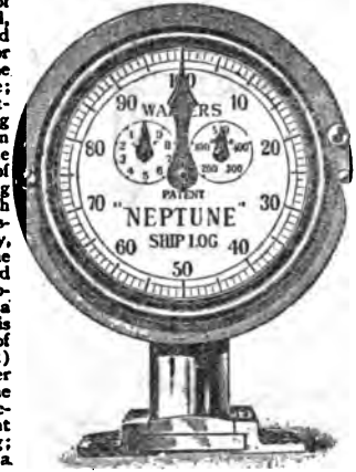
FIG. 7.—Dial-plate of Neptune Log.
