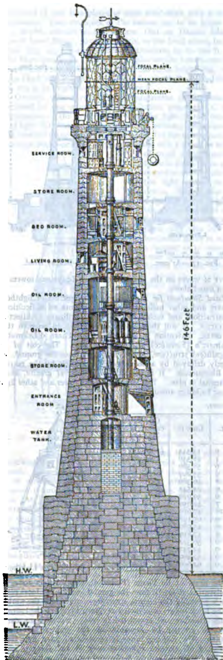
FIG. 13.—Bishop Rock Lighthouse.
