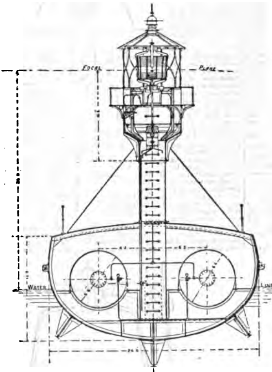
FIG. 49.—Otter Rock Light-vessel.
