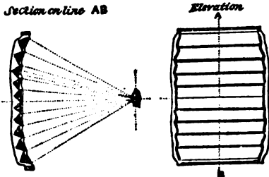
FIG. 37.—Chance's Dioptric Spherical Mirror.
