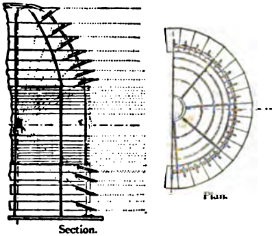
FIG. 35.—Fixed Apparatus at Chassiron Lighthouse (1827).
