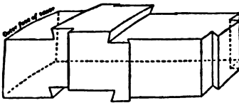
FIG. 23.—Perspective drawing of Dovetailed Stone (Wolf Rock).
