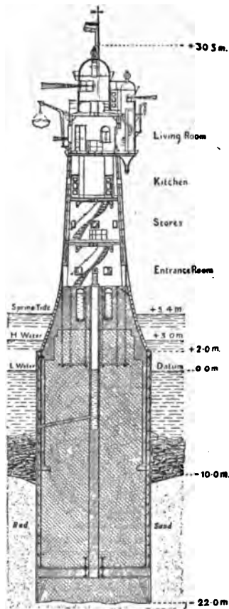
FIG. 21.—Rothersand Lighthouse.
