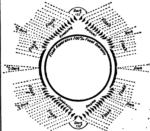
FIG. 45.—Isle of May Apparatus.
