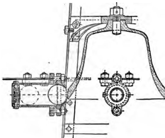
FIG. 52.—Buoy Bell.
