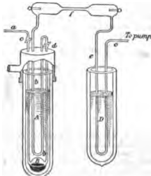
FIG. 9.—Apparatus for continuous Spectroscopic Examination.
