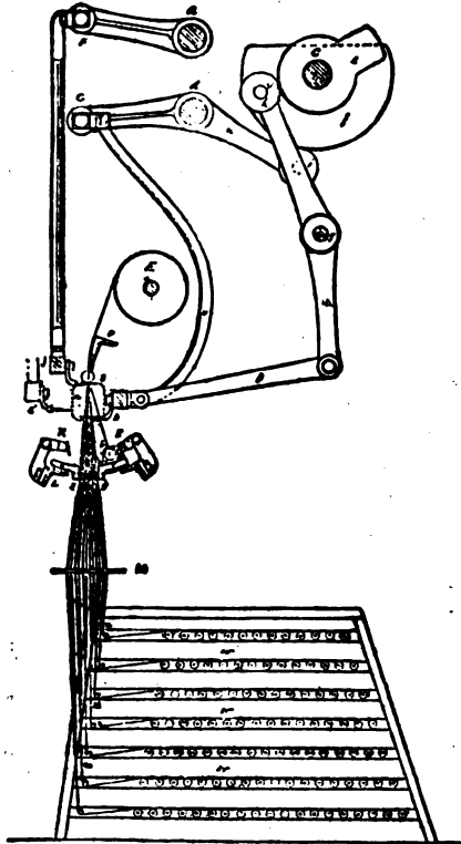
FIG. 49.—Section of Lace Machine.
