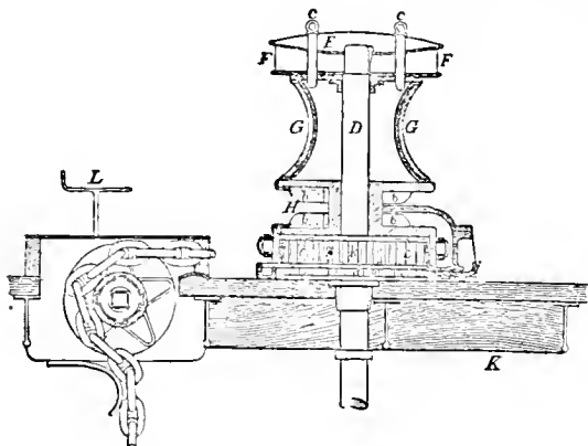
FIG. 1.—Vertical Section of Capstan.
