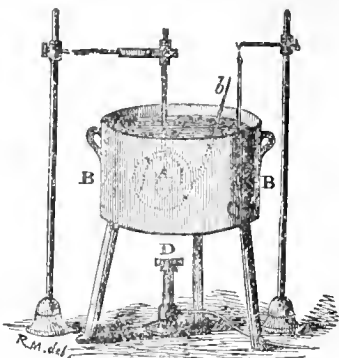
FIG. 8.—Dumas's Vapour-density Apparatus. A, glass globe, supported by wire claw; b, projecting portion of neck; B, bxb; C, thermometer; D, gas-burner for heating bath.
