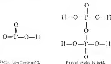
Meta-phosphoric acid.
