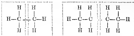
Dimethyl = ethane.
