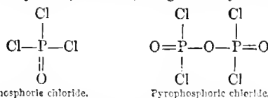
Phosphoric chloride. Pyrophosphoric chloride.
