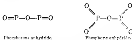
Phosphorous anhydride.
